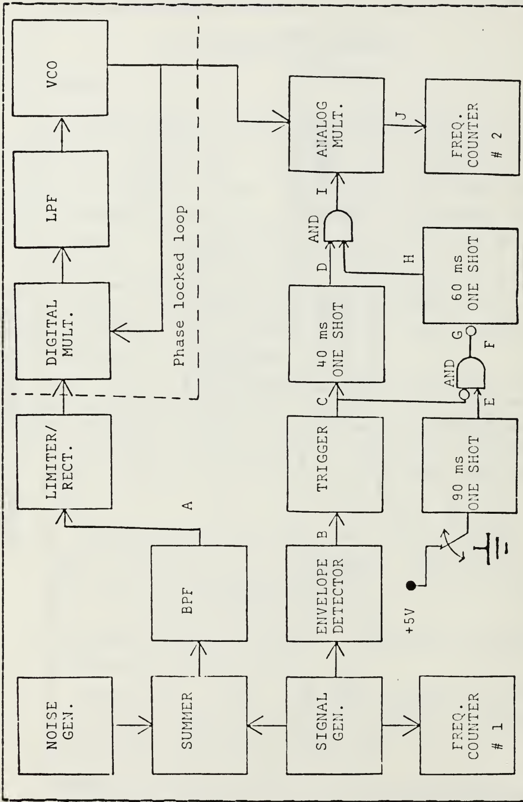
Figure 3.2 Circuit Block Diagram.
