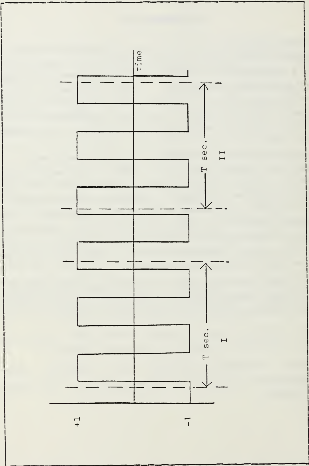
Figure 2.1 Zero Crossings/Window Relationship.
