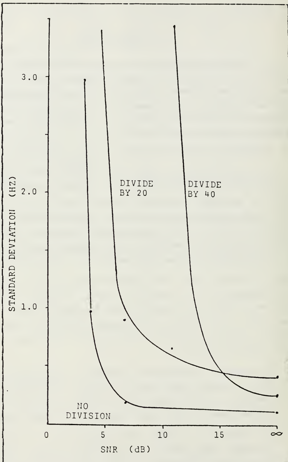
Figure 5.1 Tone Measurements.
