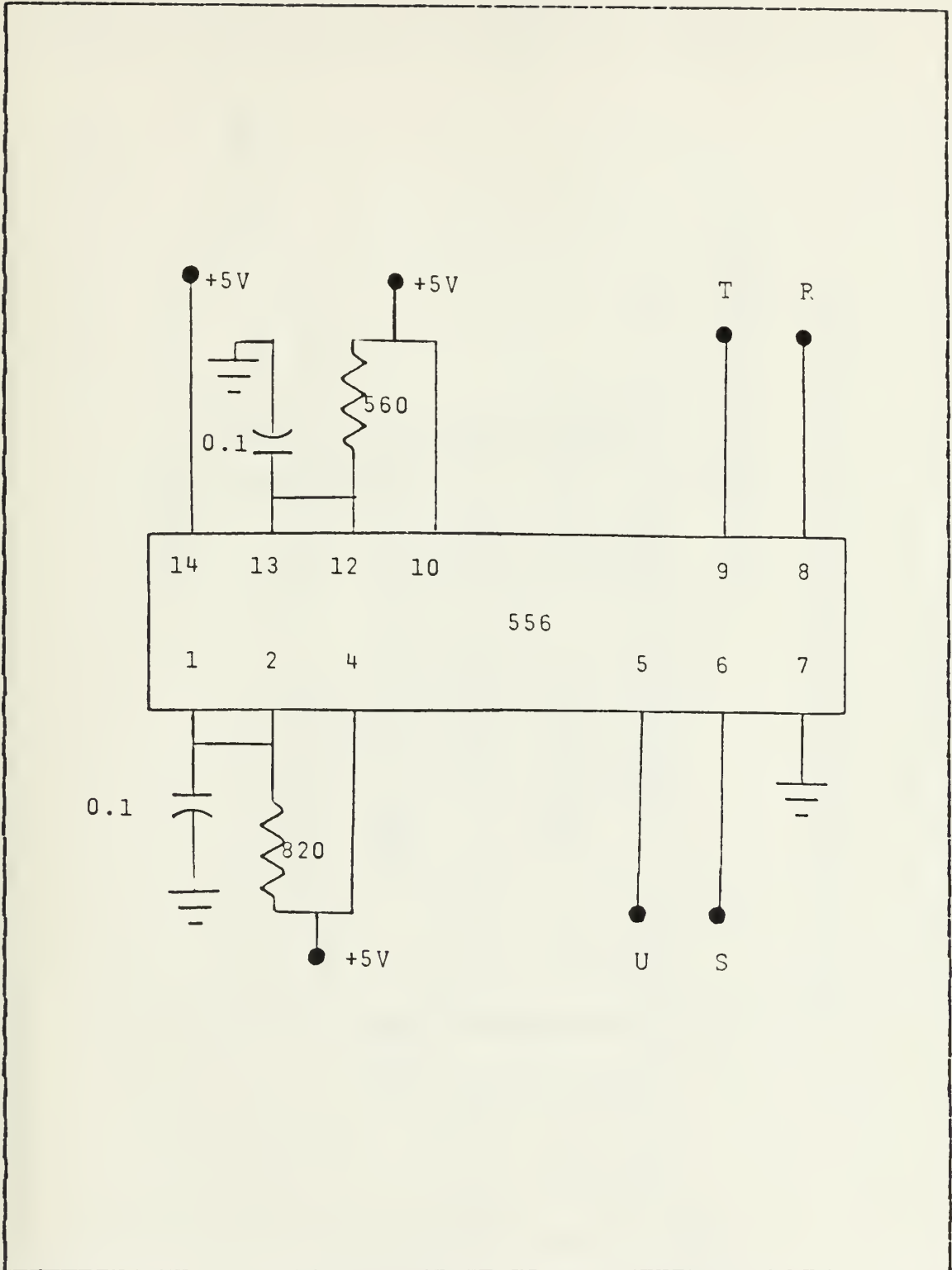
Figure A.10 60 and 90 \mu sec One Shots.
