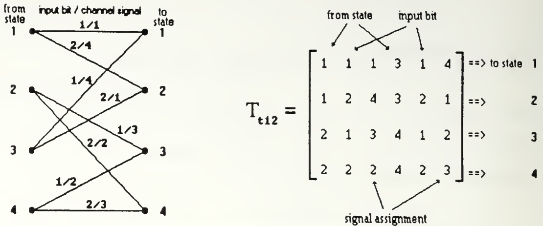
Signal assignment trellis for rate 1/2, 4-FSK, 4 state code with corresponding T matrix
