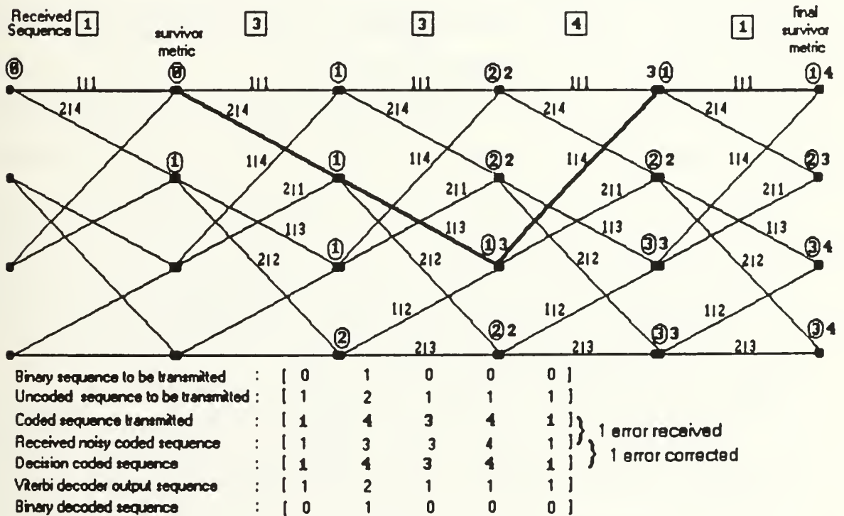
Figure 2.6 Example Viterbi decoder.
