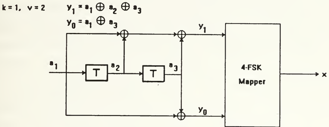
Figure 4.3 TCM encoder for rate 1/2, 4-FSK, 4 state code.
