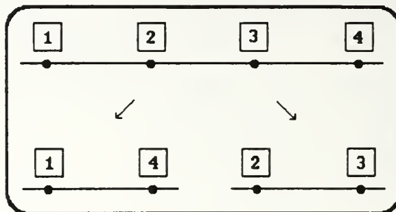
Figure 2.4 4-FSK signal set and set partitioning
