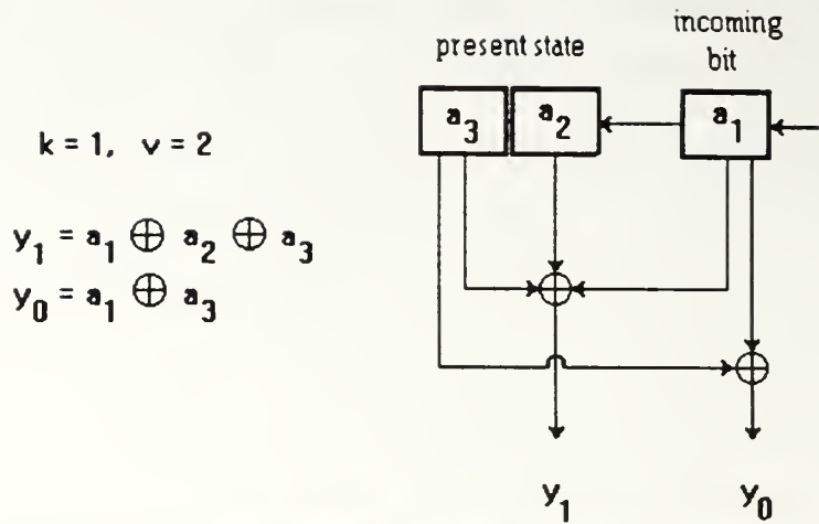
Figure 2.1 Inputs, state variables, and encoder connections for rate 1/2 code
