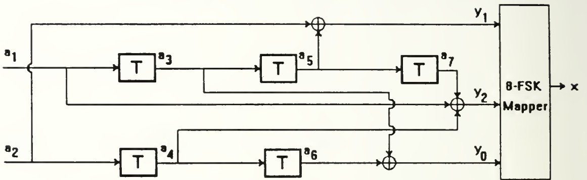
Figure 4.17 TCM encoder for rate 2/3, 8-FSK, 32 state code.
