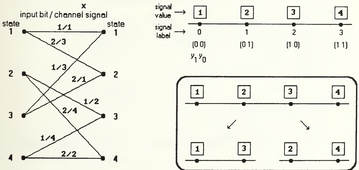
Figure 4.6 4-FSK trellis, signal set and set partitioning.
