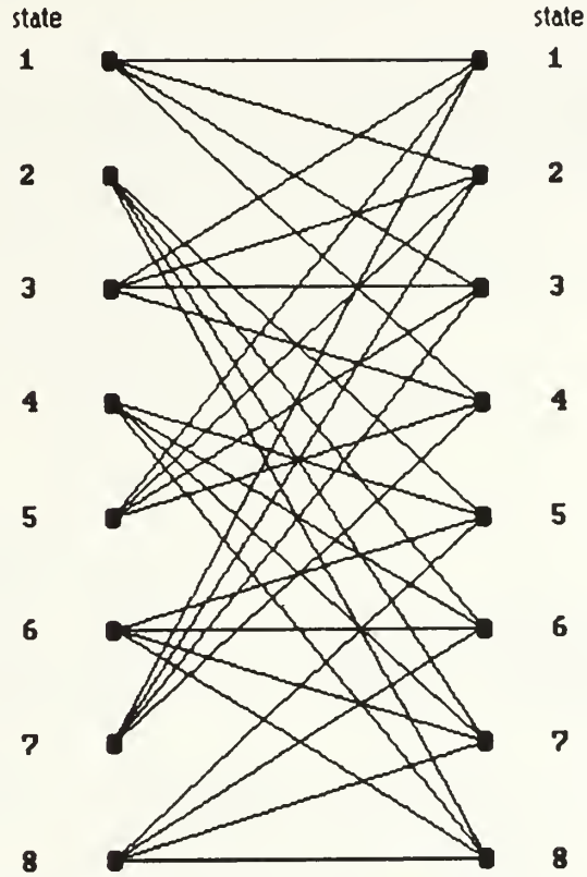
Figure 4.13 Trellis for rate 2/3, 8-FSK, 8 state code.
