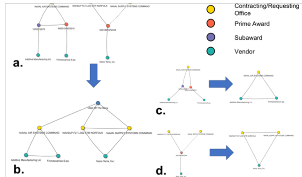
Example contract network (top) and folded network (bottom) within the Department of the Navy
