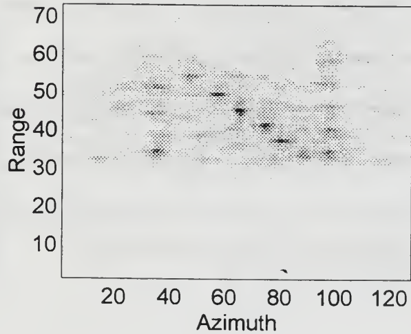
25d Chirped-Focused SAS Image of N-target
