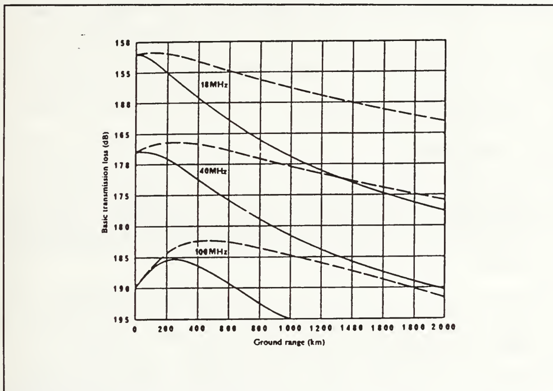
Figure 12. Loss versus Range
