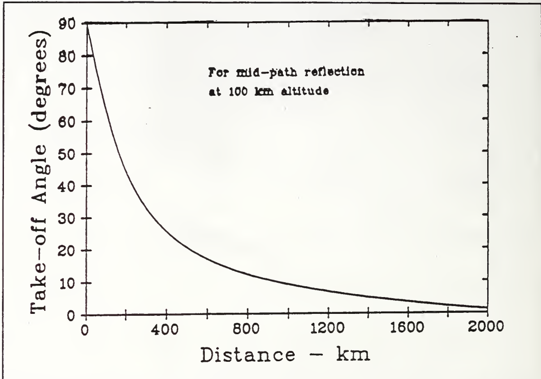
Figure 10. Take-off Angle
