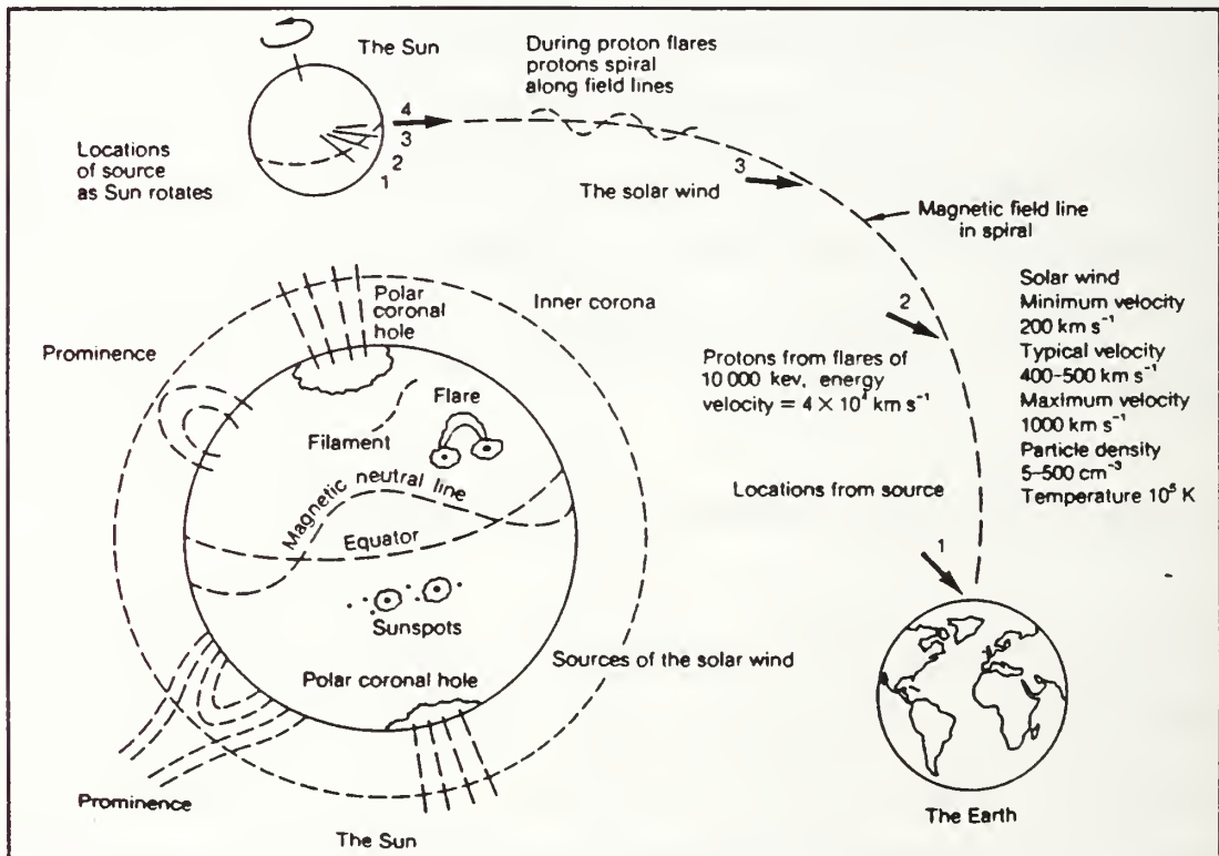
Figure 13. Solar Features and Solar Wind
