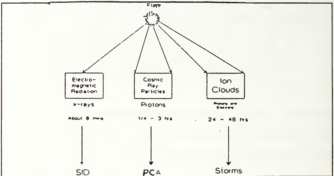
Figure 15. Solar Flare Activity
