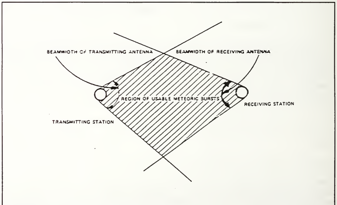
Figure 8. Antenna Beam Width
