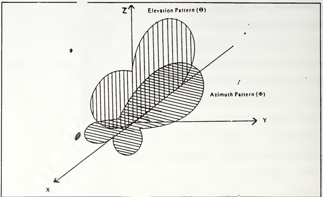
Figure 7. Antenna Radiation
