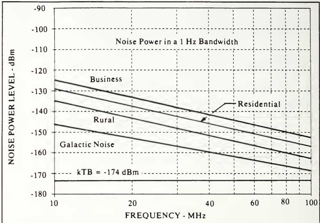
Figure 11. Artificial Noise
