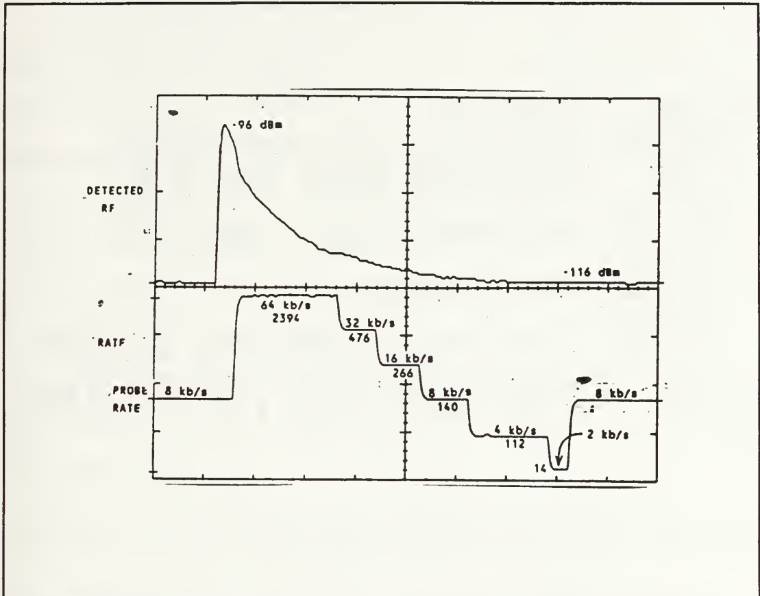
Figure 17. Variable data rates
