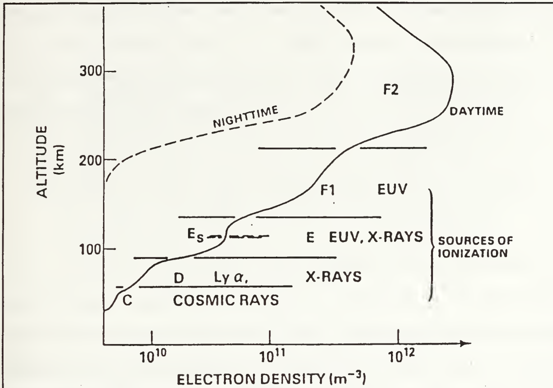
Figure 14. Ionospheric Layers
