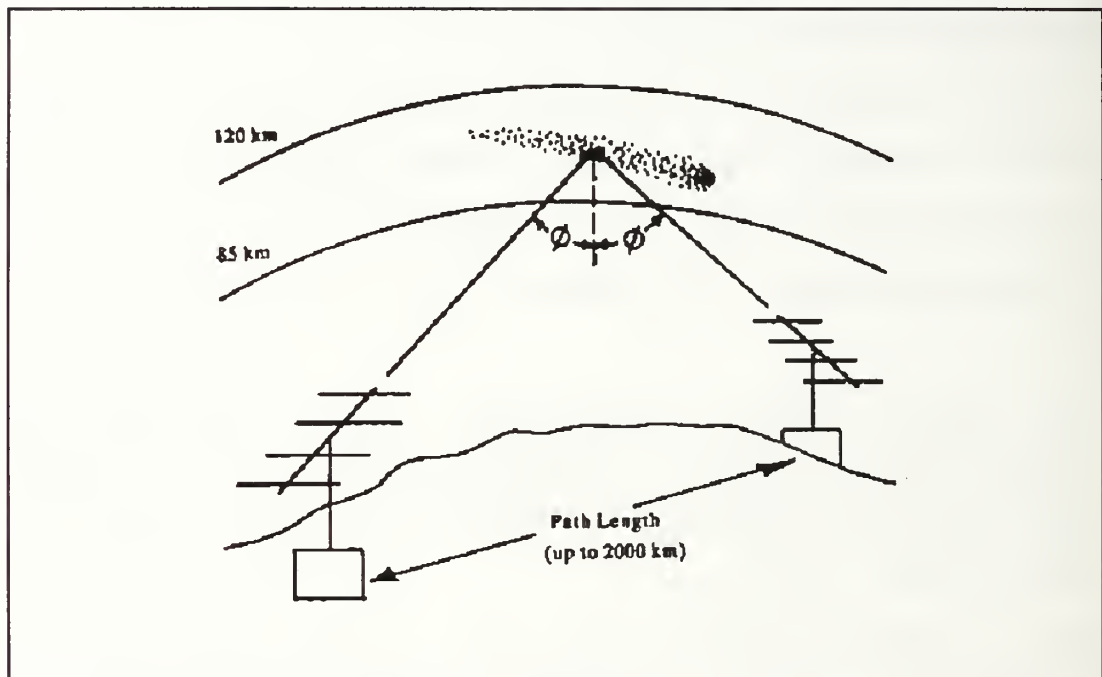
Figure 1. Meteor Burst Overview
