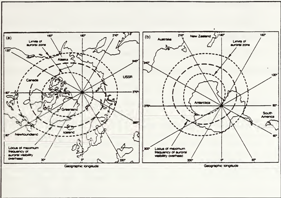
Figure 16. Auroral Zones
