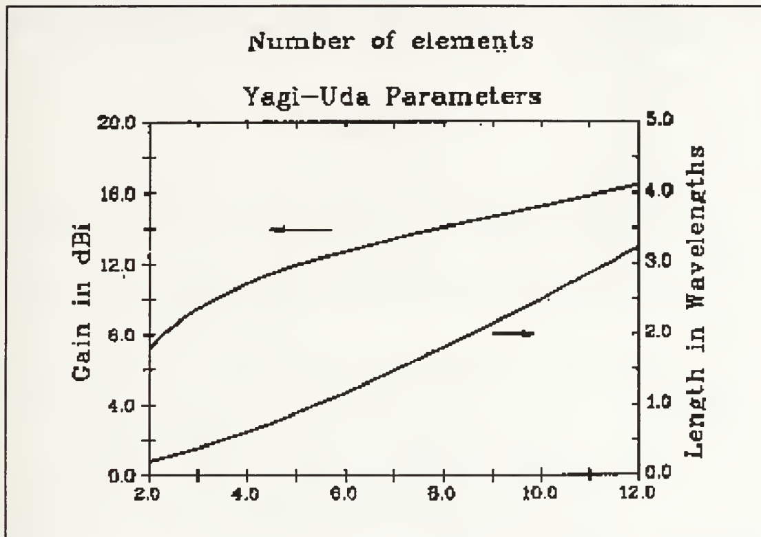
Figure 9. Antenna size versus gain
