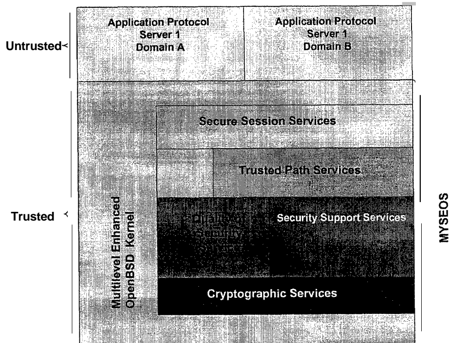
Figure 2. MYSEA Server
