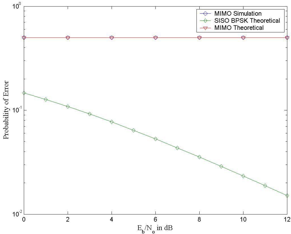
Figure 17. Results in Multipath Fading Channel.
