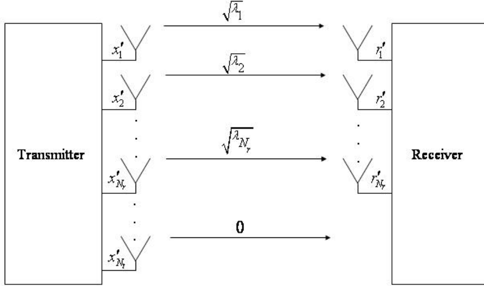
Figure 5. The equivalent MIMO model N_r < N_t (After Reference [1]).
