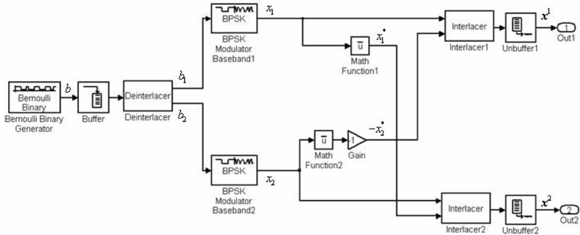
Figure 11. MIMO Transmitter Simulation.
