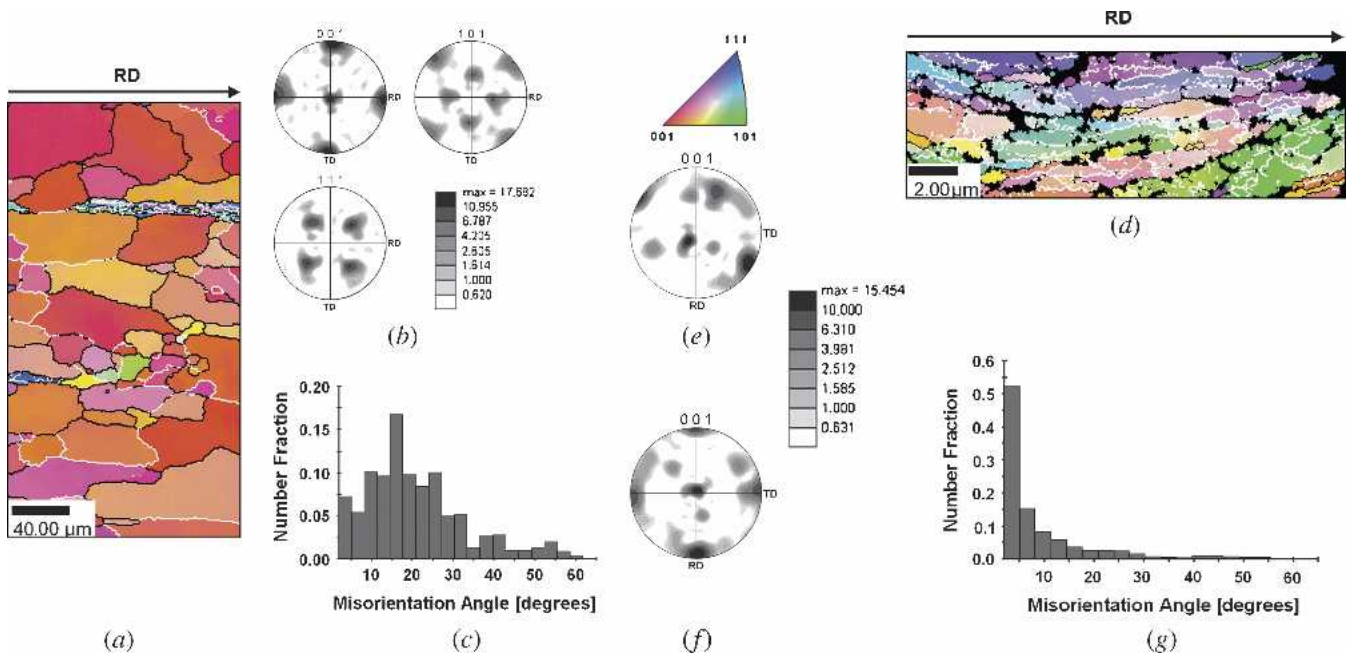
Fig. 7—Inverse-pole-figure maps for the ND, pole figures, and misorientation distributions for (a) through (c) high-purity aluminum and (d) through (g) commercial-purity aluminum after rolling to an effective strain of 3.4. On the inverse-pole-figure maps, low-angle boundaries are white, and high-angle boundaries are black: (e) as deformed and (f) after -60 deg rotation about ND followed by -20 deg rotation about RD.
