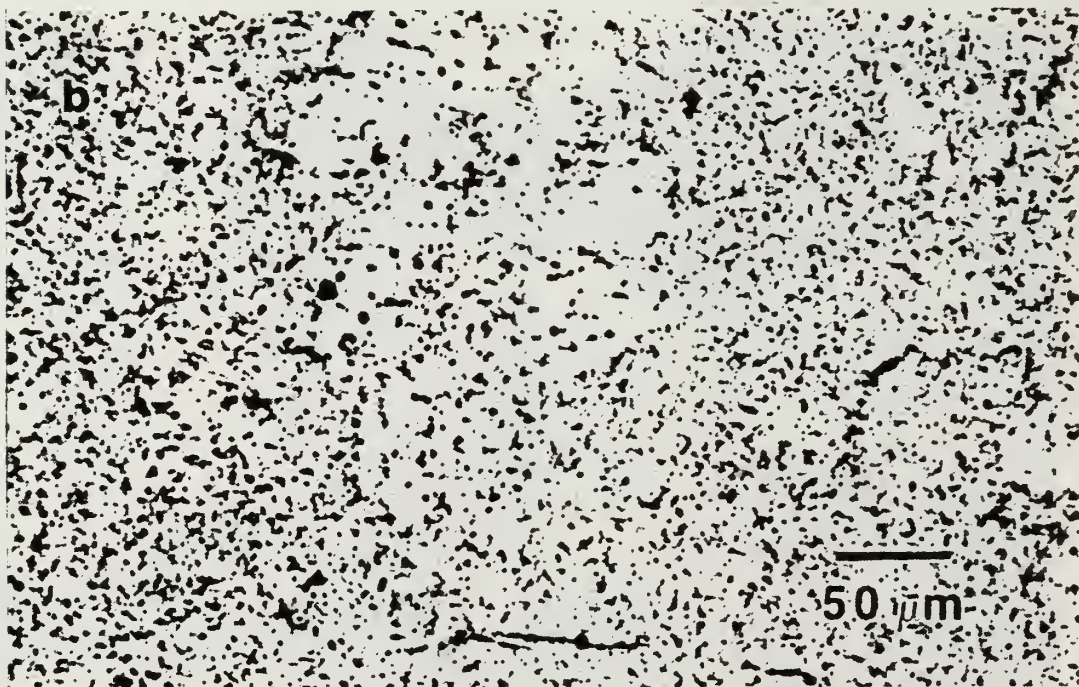
Figure 4.17 Optical micrographs of two Al-10Mg-01Zr alloys taken using unpolarized light techniques after: (a) Processing at 350°C using TMP V (b) Processing at 350°C using TMP VI.
