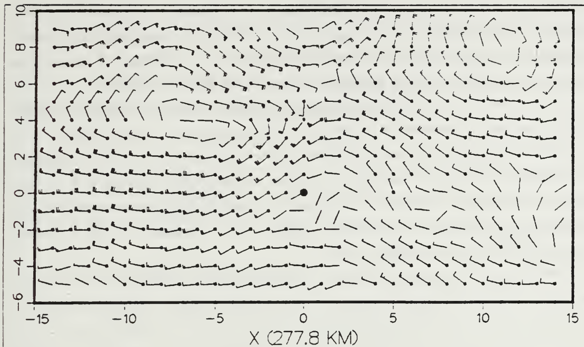
Figure 3.7 As in Fig. 3.3, except for Category FAST minus Category SLOW.
