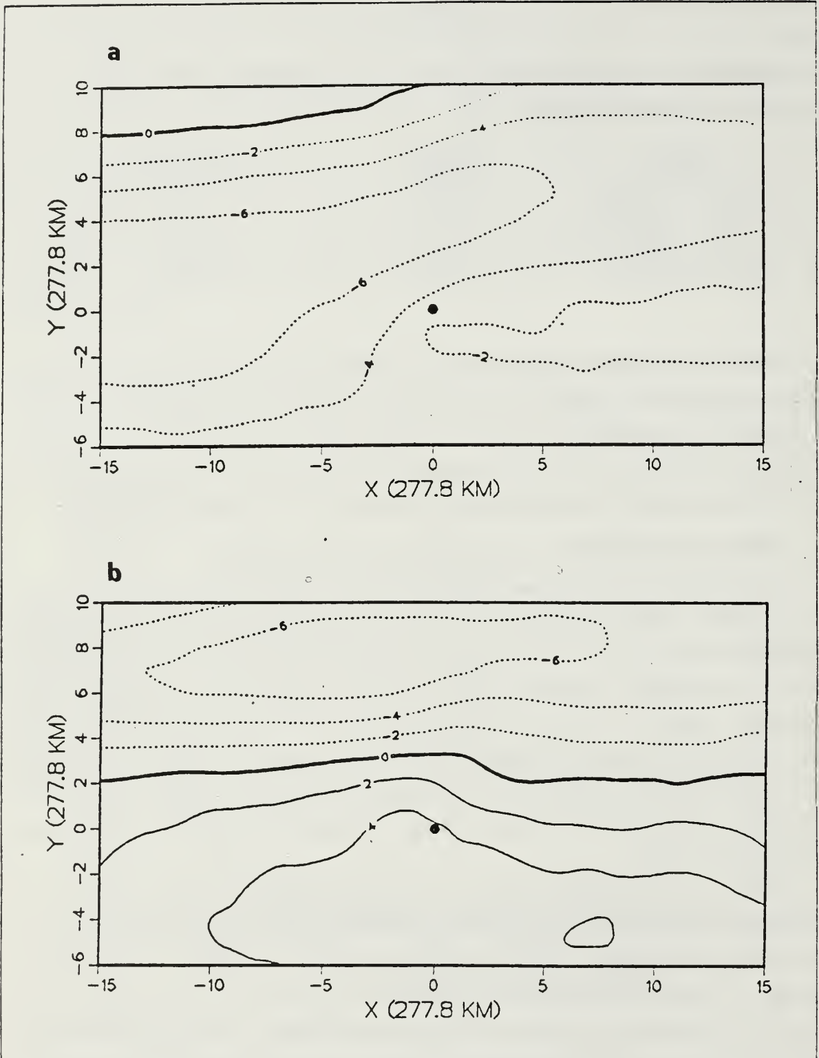
Figure 2.8 (a) Mode 1 and (b) mode 2 for the 250-700 mb zonal shear (normalized fields multiplied by 100).
