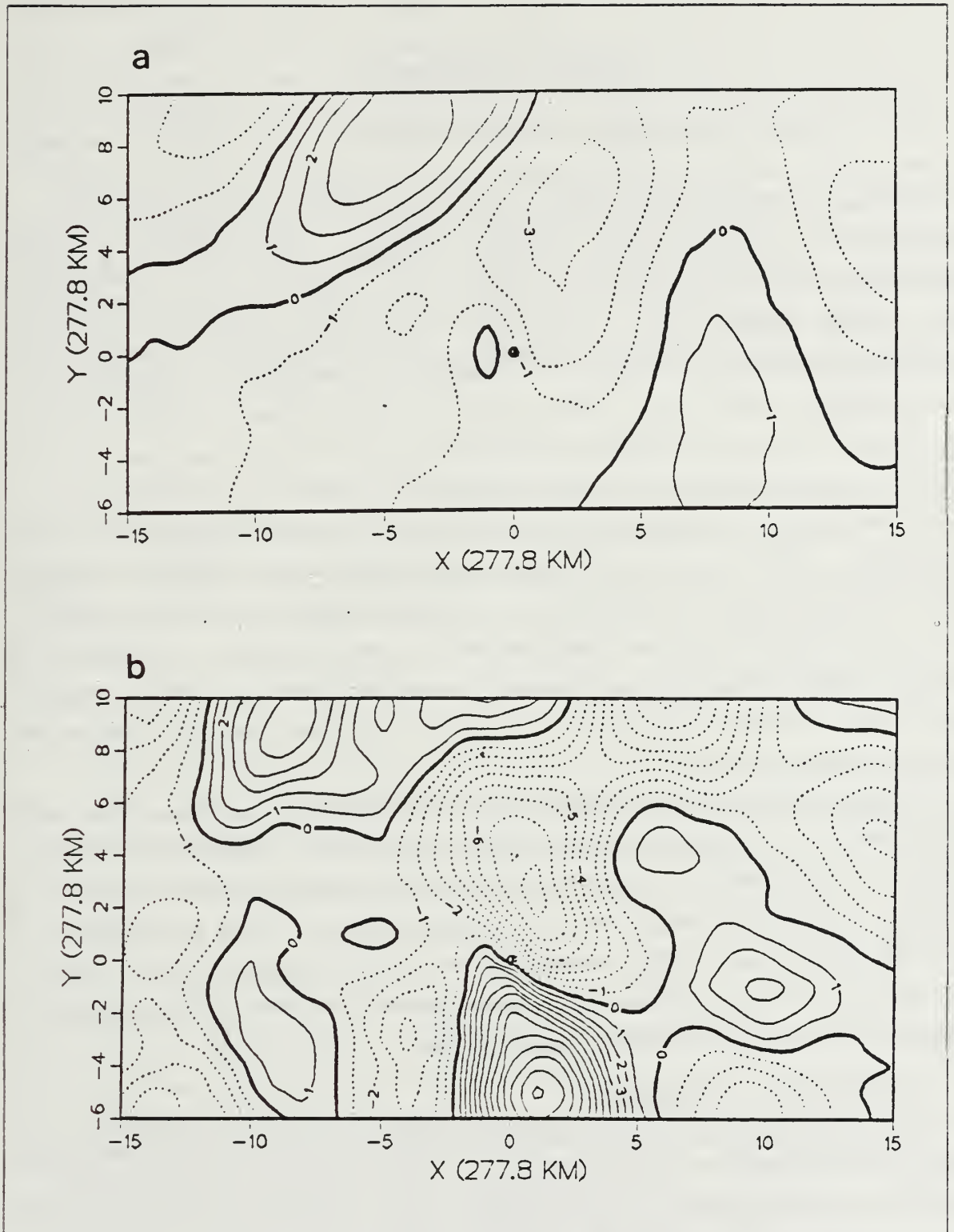
Figure 2.12 As in Fig. 2.11, except for meridional shear using (a) only 5 and (b) 35 eigenvectors.
