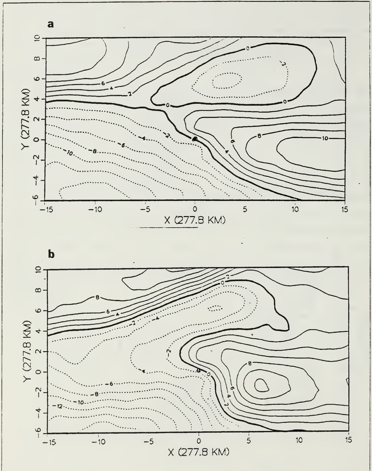
Figure 2.11 Reconstruction of the 400-700 mb zonal shear of Typhoon Hope using (a) only 5 and (b) only 25 eigenvectors.
