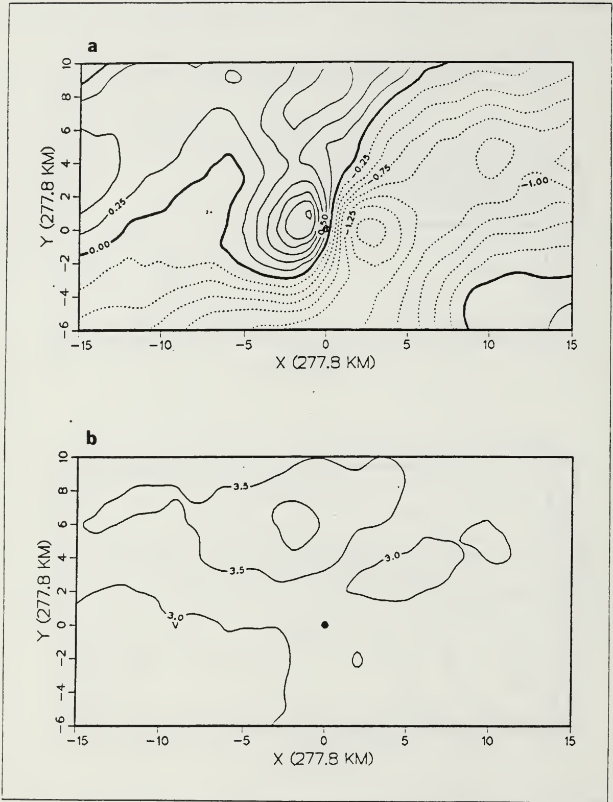
Figure 2.4 As in Fig. 2.3, except for V-component.
