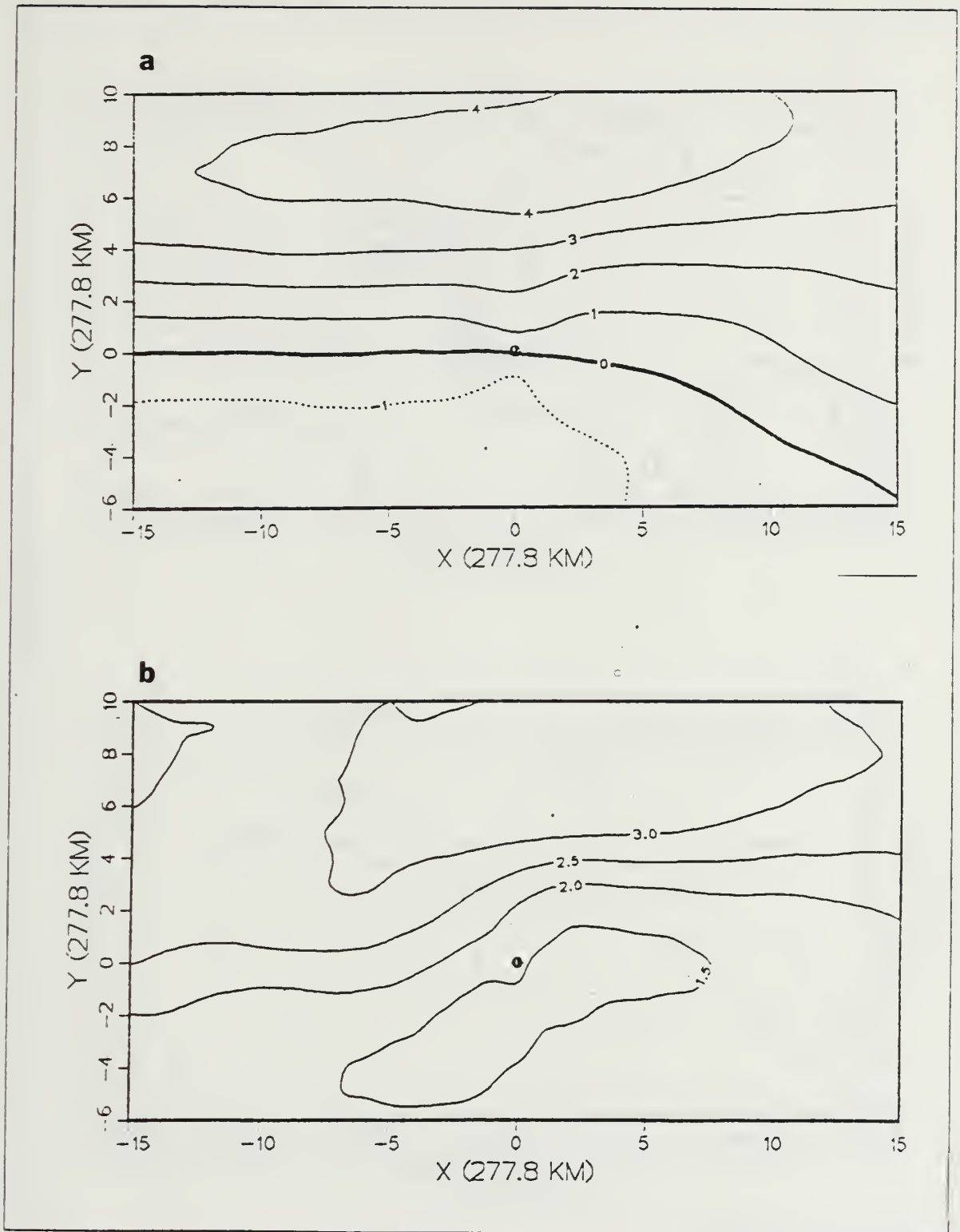
Figure 2.1 (a) Mean and (b) standard deviations of the U-component shear (m/s per 100 mb) for the 400-700 layer.
