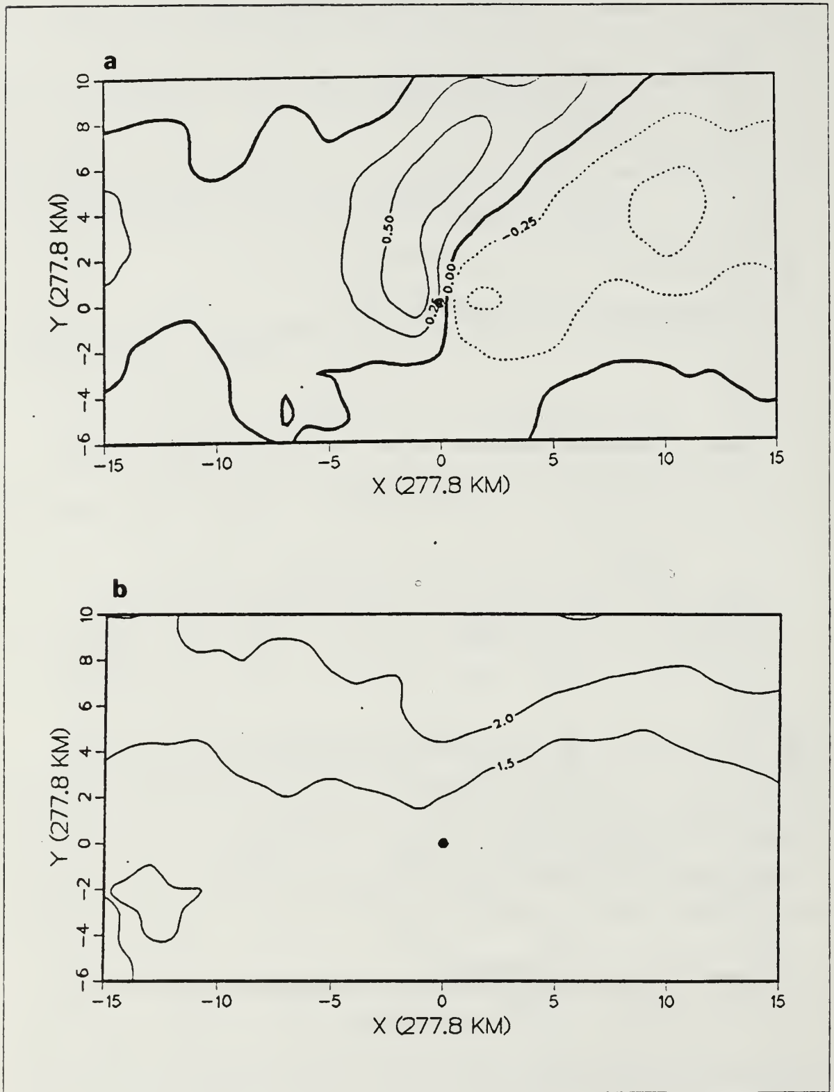
Figure 2.2 As in Fig. 2.1, except for V-component.
