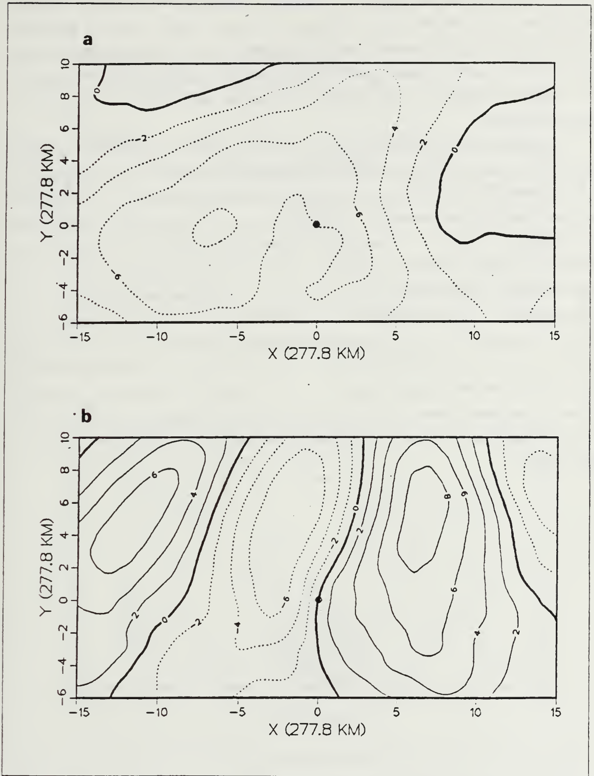
Figure 2.9 As Fig. 2.8 except for meridional shear modes.
