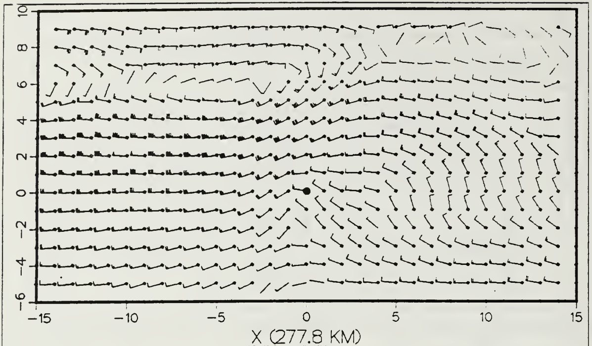
Figure 3.3 Difference in the 250-700 mb wind shear (m/s per 100 mb) for Category NE minus Category NW with symbols as in Fig. 3.2.
