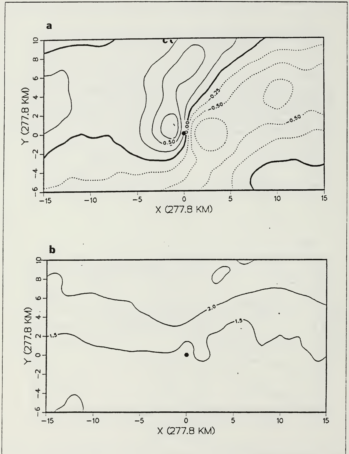
Figure 2.6 As in Fig. 2.5, except for V-component.
