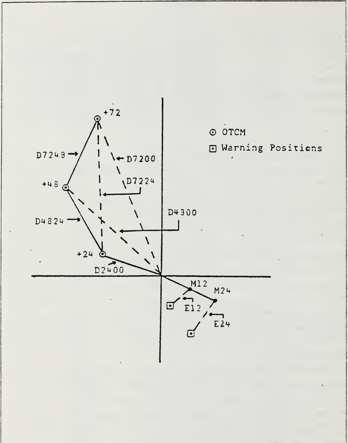
Figure 4:1 The OTCM forecast positions at +24, +48 and +72 h (circled dots) and backward extrapolation positions at M12 and M24 h that are used to define potential predictors (Table 6) in the regression analysis.
