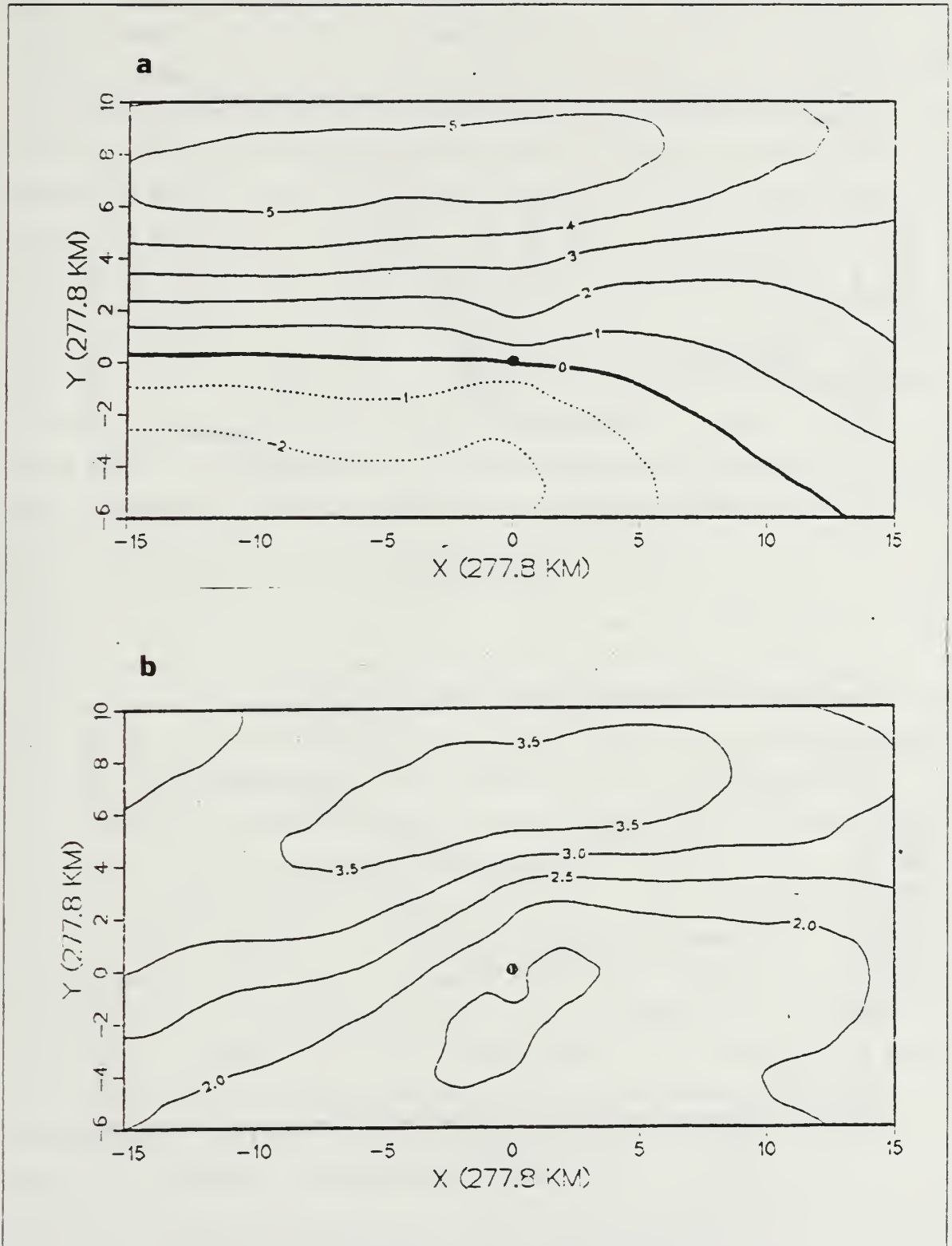
Figure 2.5 As in Fig. 2.1, except for 250-700 mb shear layer.
