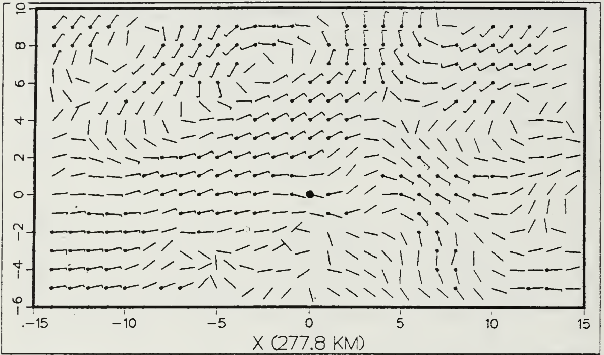
Figure 3.10 As in Fig. 3.9, except for fast minus slow terciles of Category NW storms.
