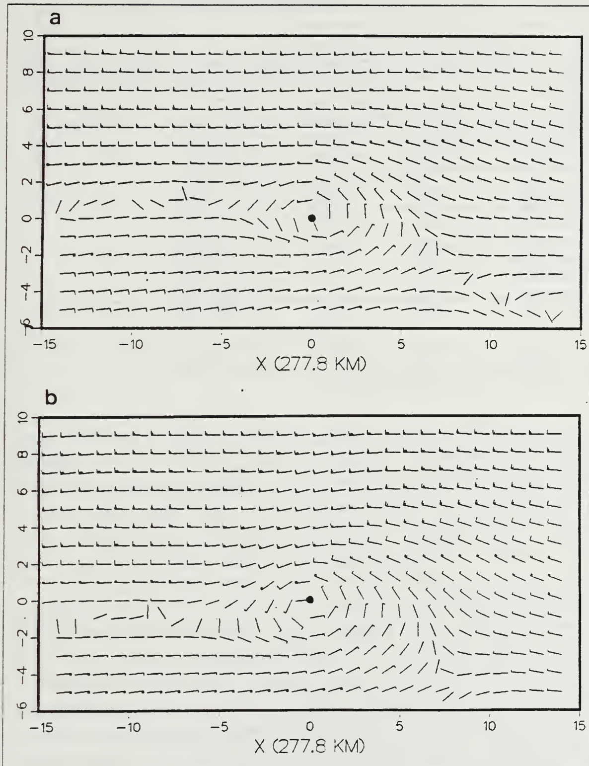
Figure 3.2 Composite 250-700 mb wind shear ( \text{m/s per } 100 \text{ mb} ) fields for (a) Category NW and (b) Category NE storms. Short (long) windbarbs and flags represent 1 (2.5) and 5 \text{m/s} shears.
