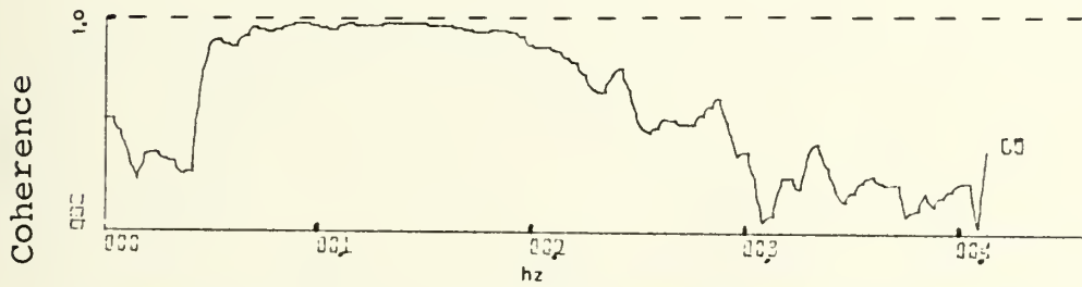
Coherence of Vertical and Horizontal Velocity Component. Depth 8.35 Meters, 21 October 1971.
