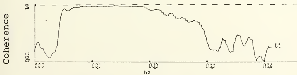
Figure 12. Coherence of Wave Height and Vertical Velocity. Depth 8.35 Meters, 21 October 1971.
