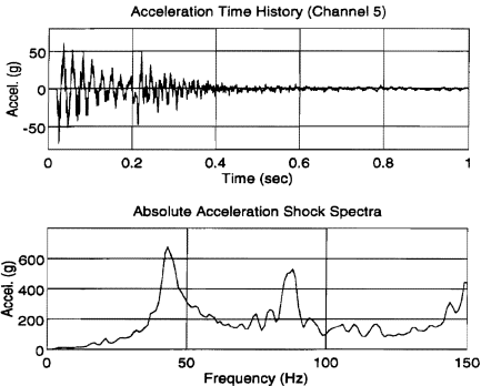
Figure 9. Acceleration Time History (Channel 5) and Absolute Acceleration Shock Spectra for Test 4 Blow 7.
