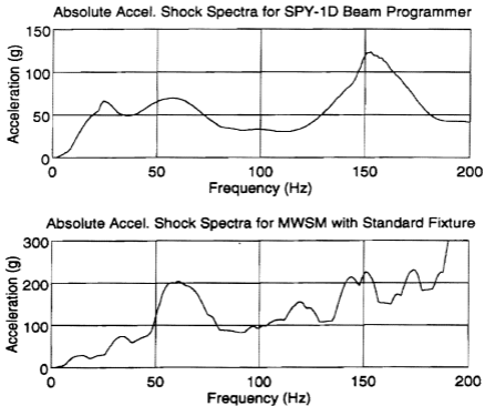
Figure 3. DDG-51 Pretrial Predicted Absolute Acceleration Shock Spectra Versus MWSM with Standard Fixture Actual Absolute Acceleration Shock Spectra.
