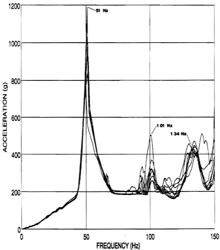
ABSOLUTE ACCELERATION SHOCK SPECTRA FOR TEST 3 (9 DROPS)
