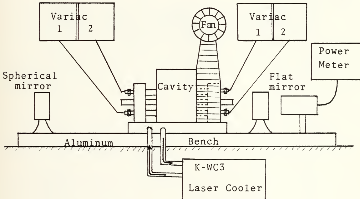
Schematic sketch of the laser system
