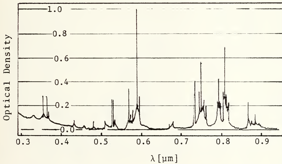
Fig. 5. Absorption spectrum of Nd:YAG at 300°K
