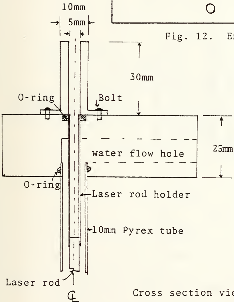
Fig. 13. Laser Rod Mounting Assembly
