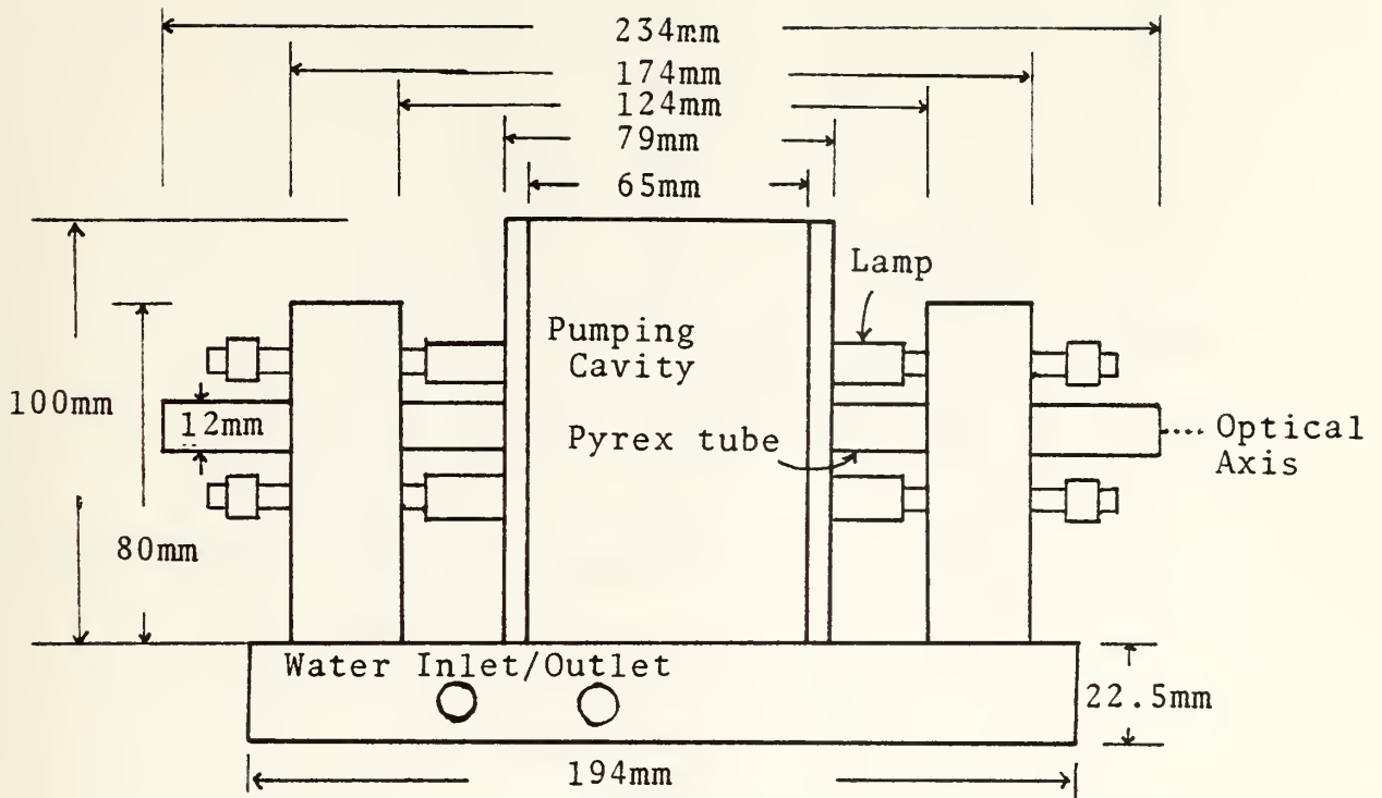
Front view of pumping cavity scale; 2mm:1mm
