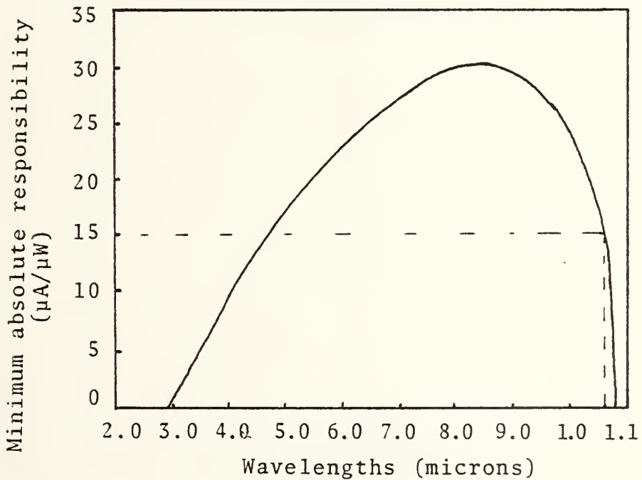
Fig. 16. The spectral response of PIN-10DP
