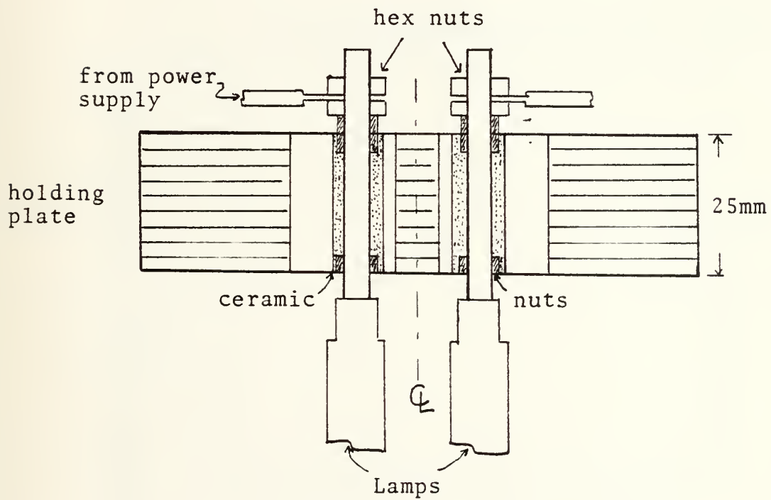
Cross section view: Scale 1:1
