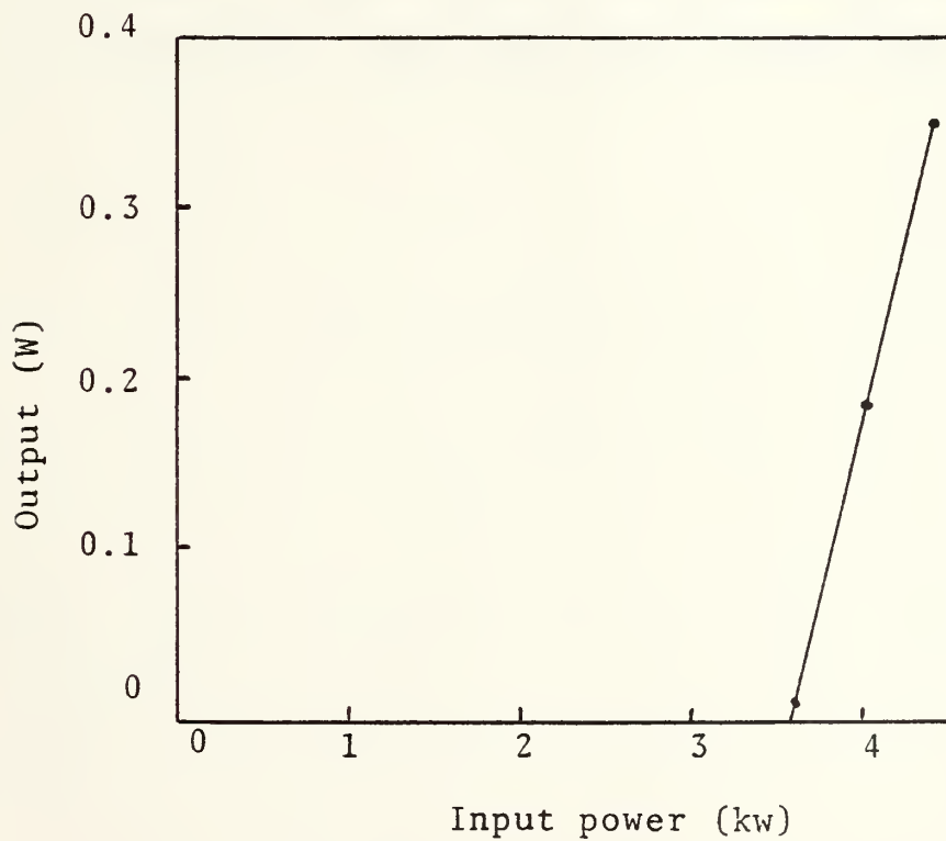
Fig. 18. Laser output of homemade system
