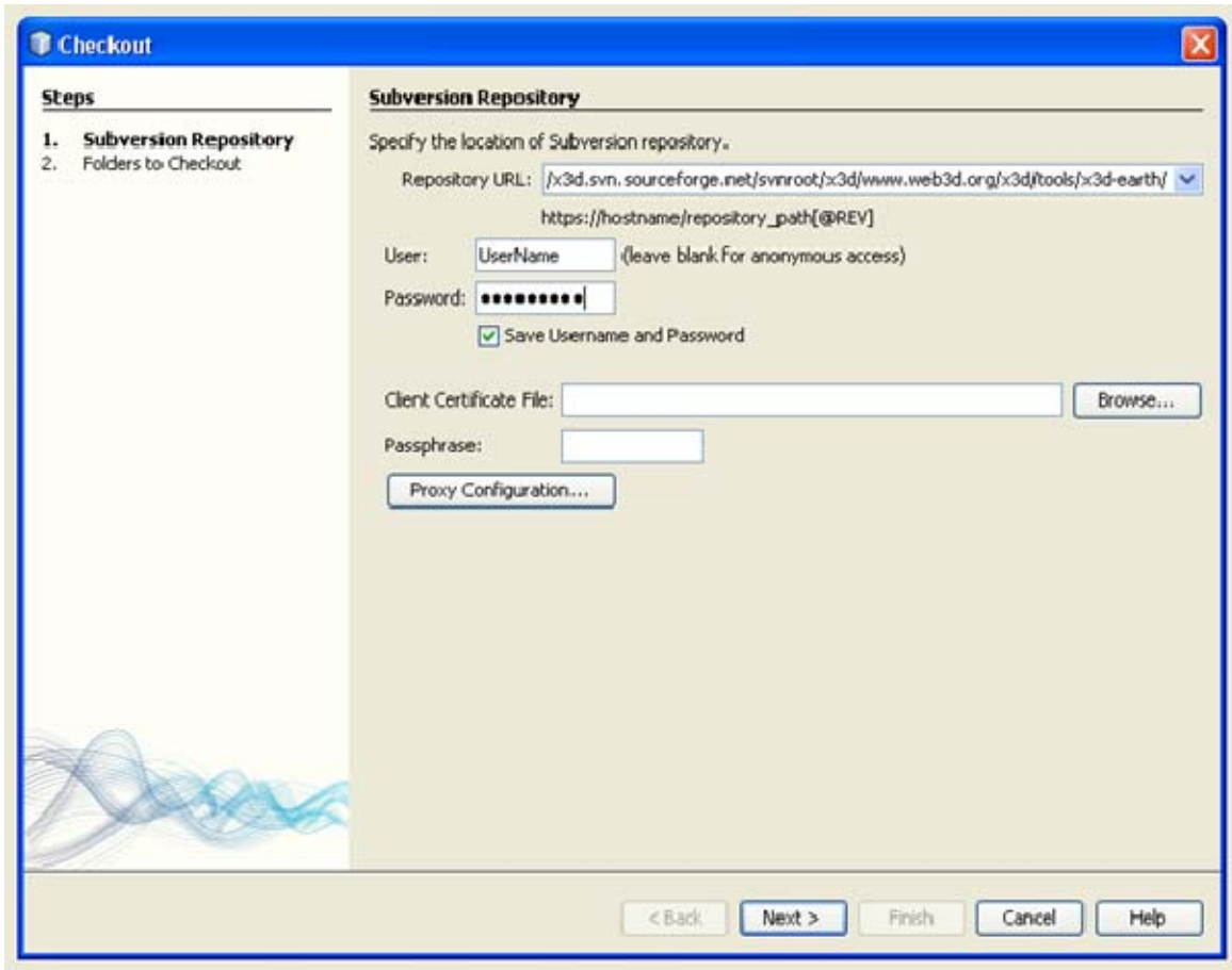
Figure 64. Subversion Repository
