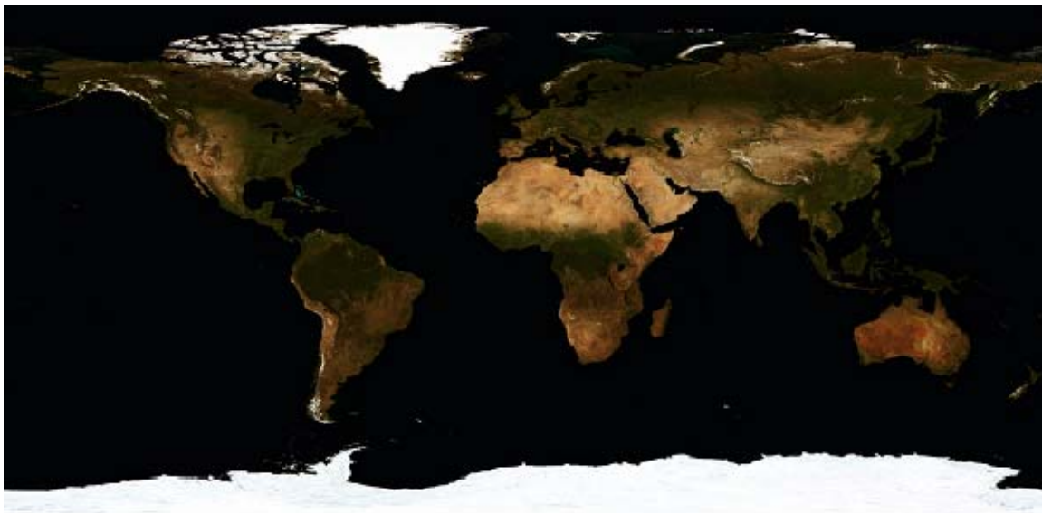
Figure 35. Blue Marble Imagery (From Stockli et al., 2005)
