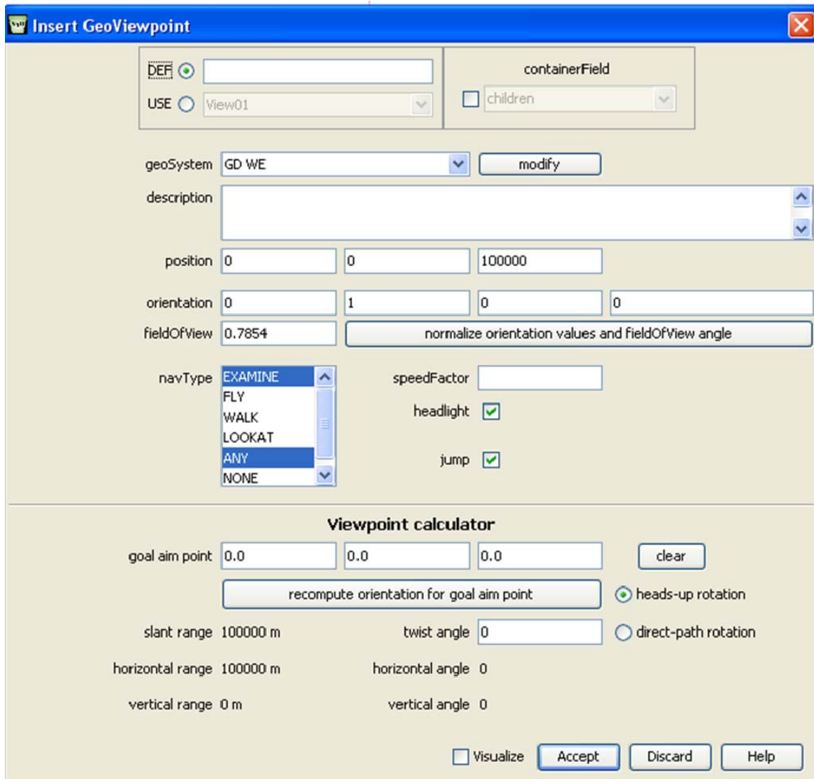
Figure 42. GeoViewpoint Editing Panel in X3D Edit
