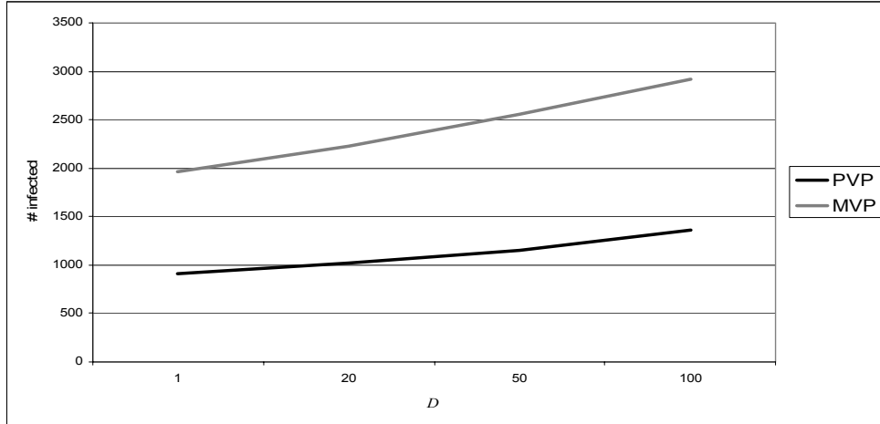
Figure 4.4: Number of Infected as a Function of the Detection Threshold.
