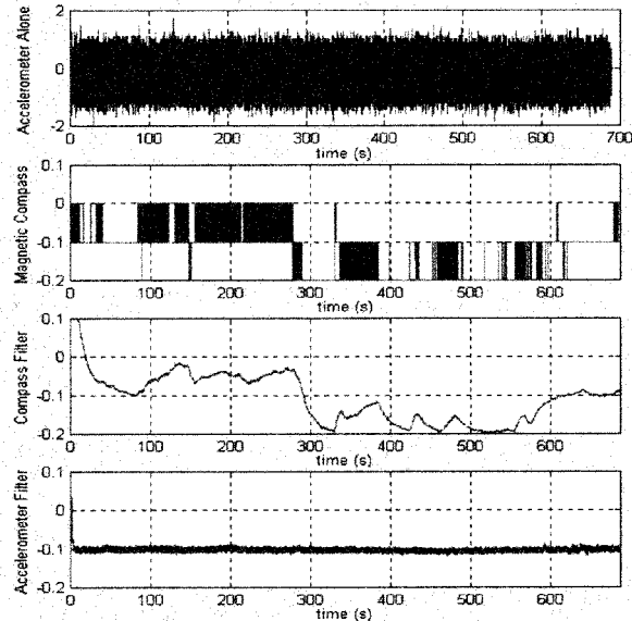
Fig. 4. Roll estimation in static conditions ( ^{\circ} ).
