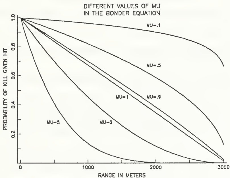
Figure 2. Various values of u for the Bonder range equation
