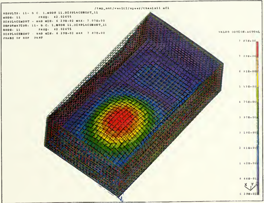
Figure 3.7. 42.02 Hz Mode Shape.
