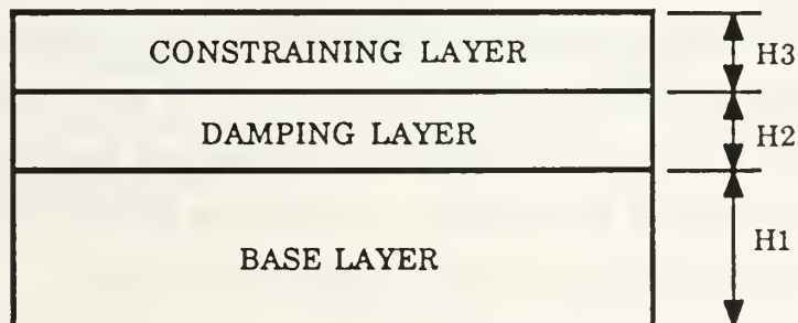
Figure 2.5. Simple Constrained Viscoelastic Layered Damping Treatment.
