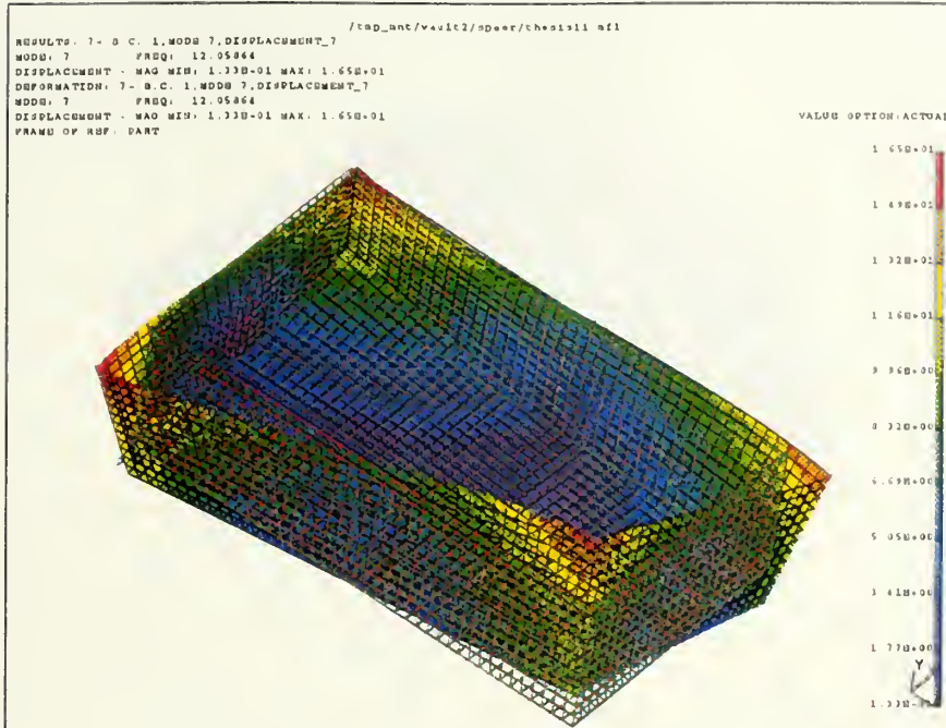
Figure 3.3. 12.05 Hz Mode Shape.
