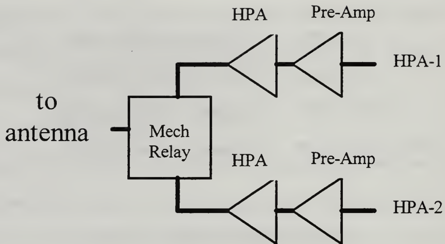
Figure 10 RF HPA PCB Block Diagram
