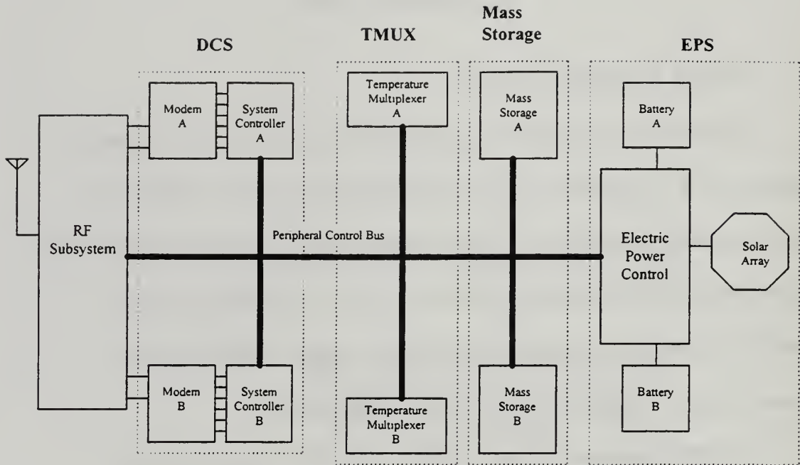
Figure 2 PANSAT System Diagram
