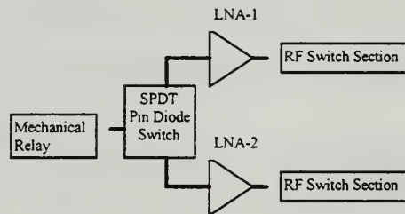
Figure 8 RF LNA PCB Block Diagram
