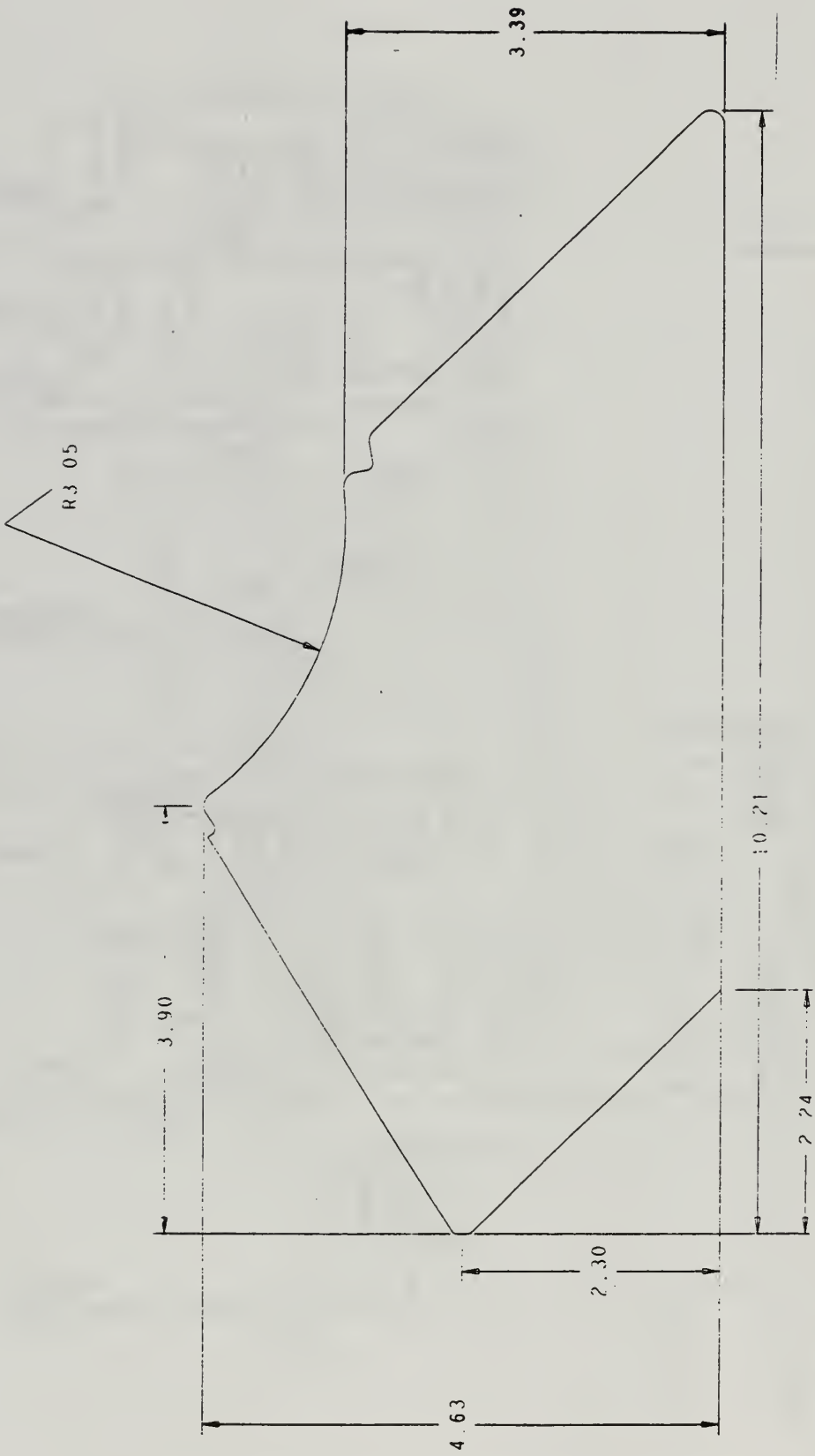
Figure 40 RF HPA PCB - Physical Size
