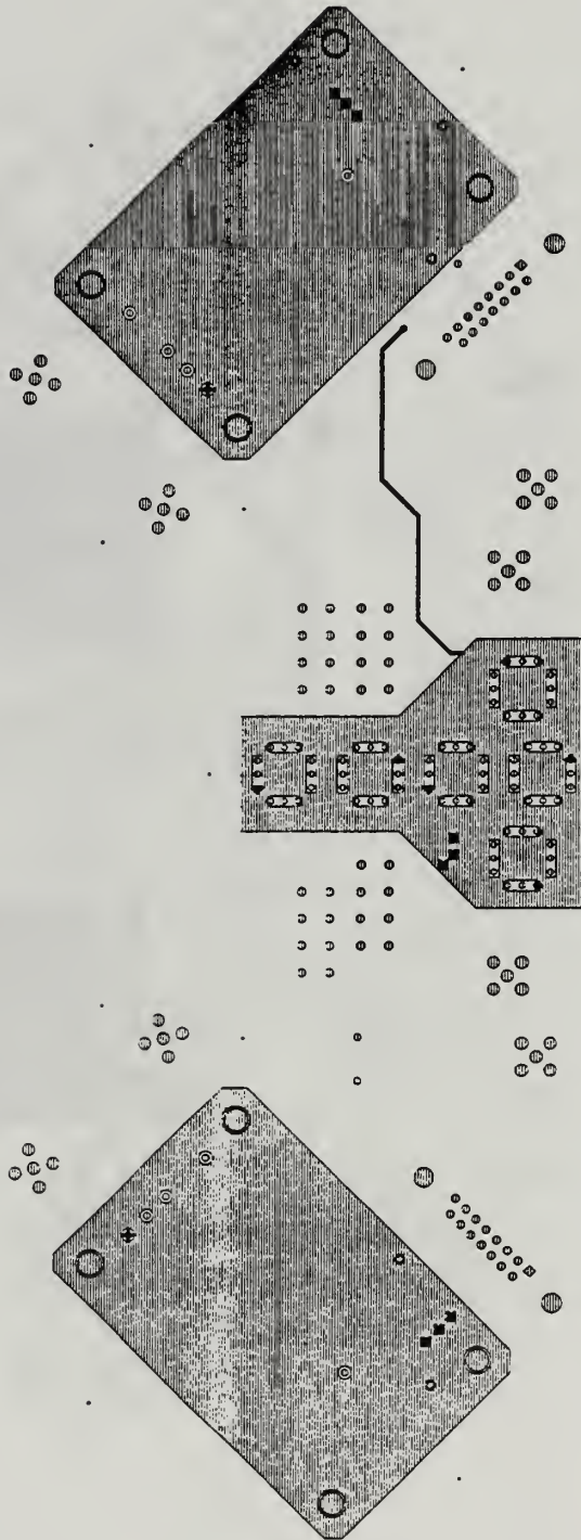
Figure 24 RF Switching PCB - Power Layer Photoplot
