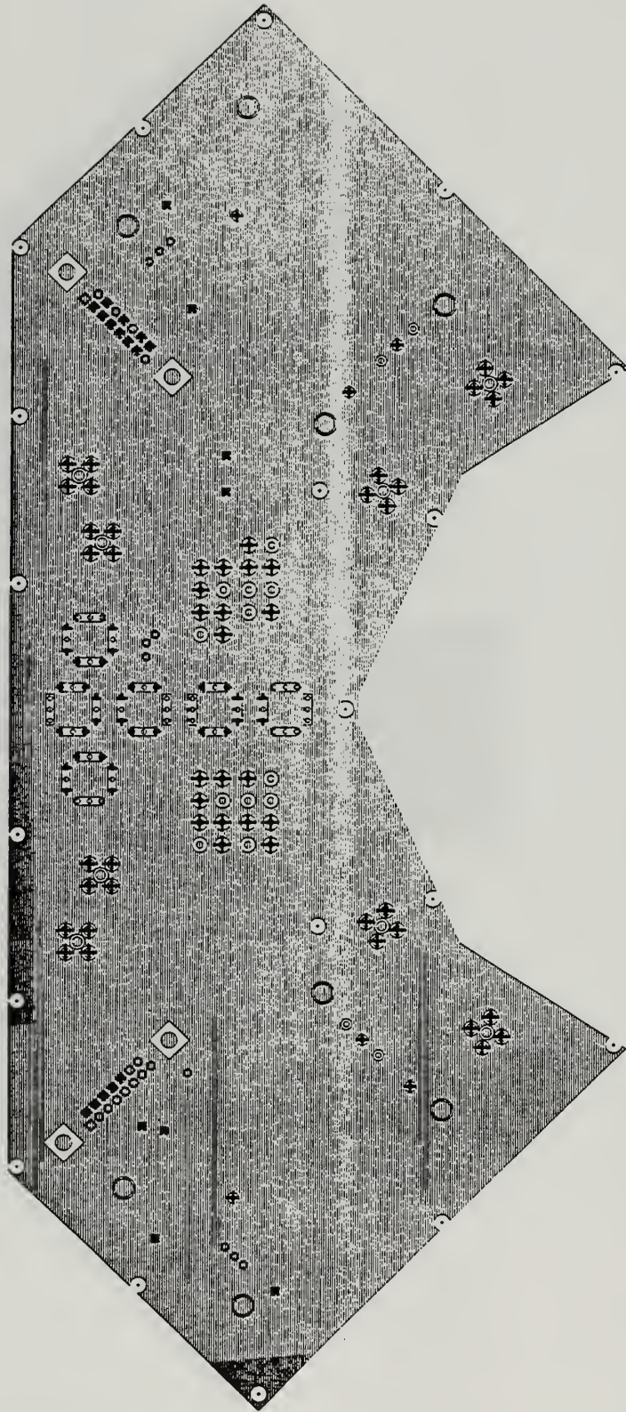
Figure 26 RF Switching PCB - Ground2 Layer Photoplot
