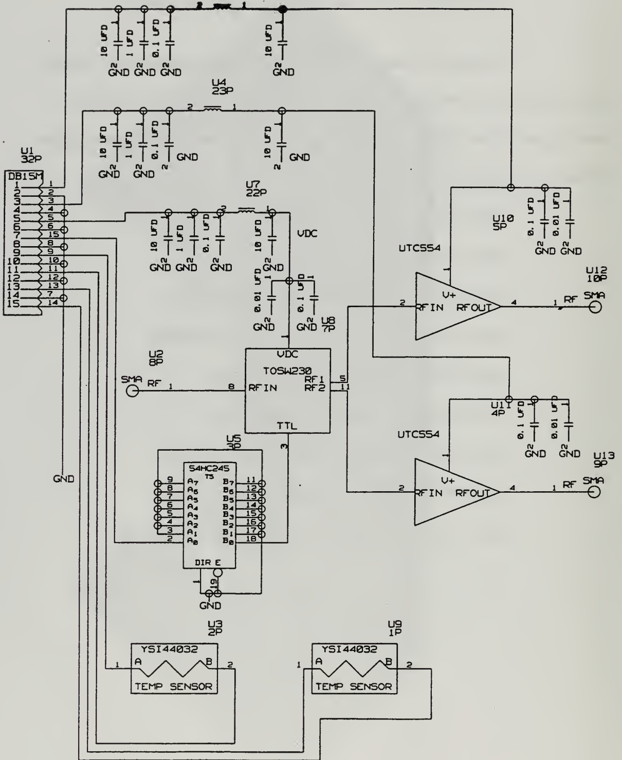
Figure 29 RF LNA Circuit Schematic
