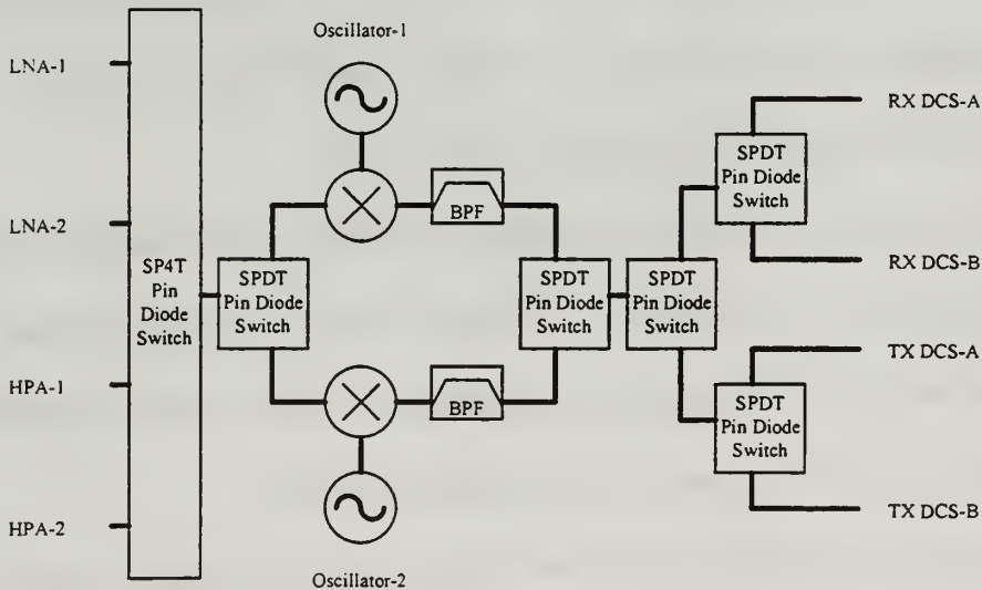
Figure 5 RF Switch PCB Block Diagram
