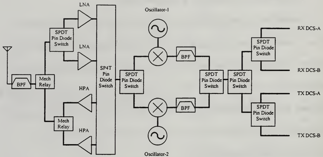
Figure 3 RF subsystem Block Diagram
