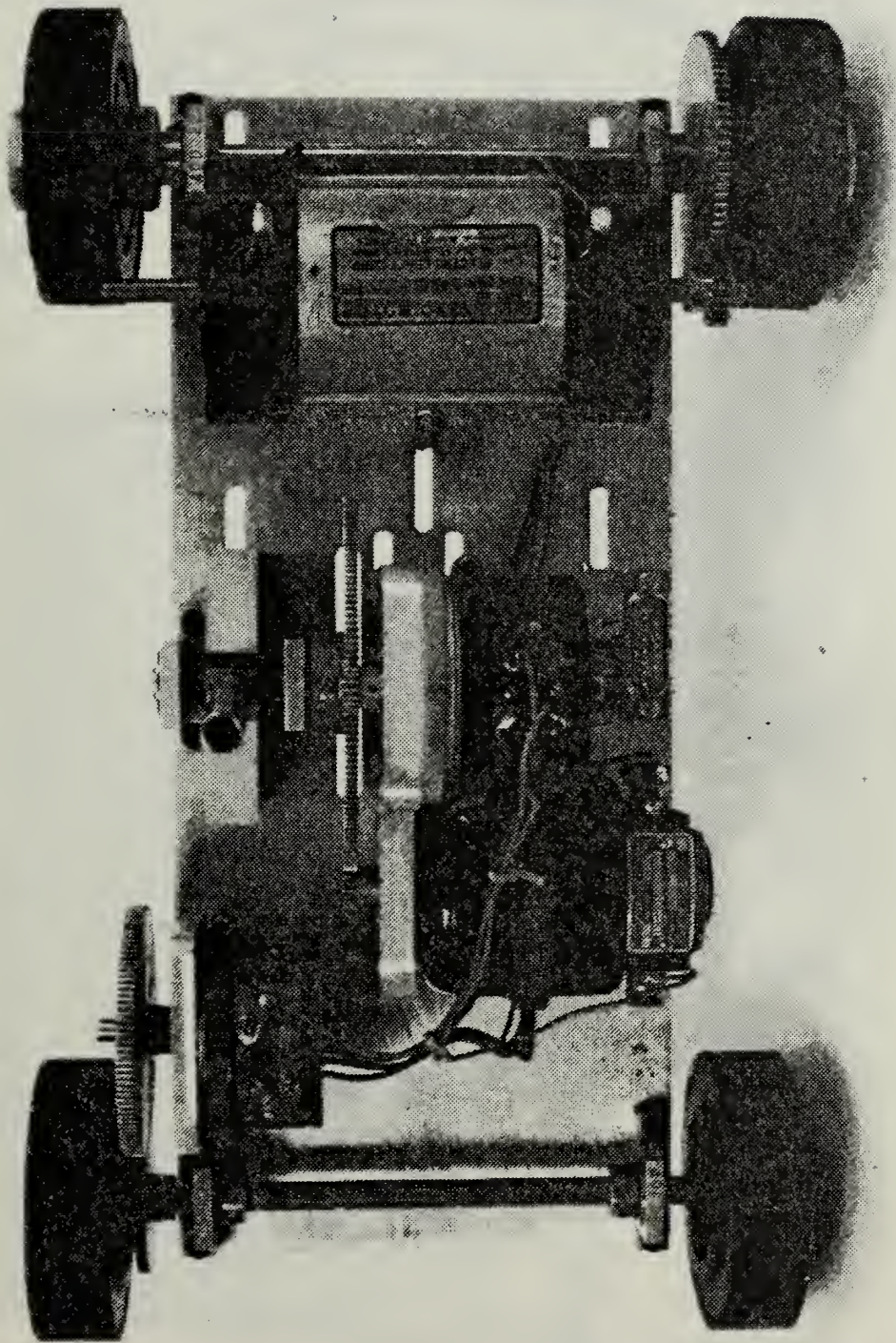
Figure 4. CART TOP VIEW
