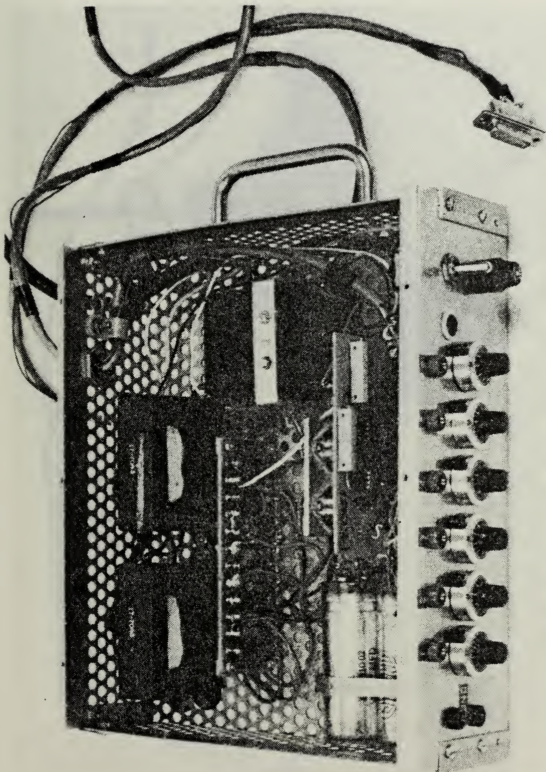
Figure 5. CONTROLLER/POWER SUPPLY--INSIDE VIEW
