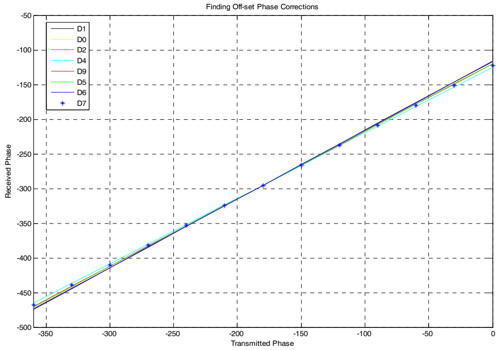
Figure 43 The approximate linear curve fit received phase vs. transmitted phase.
