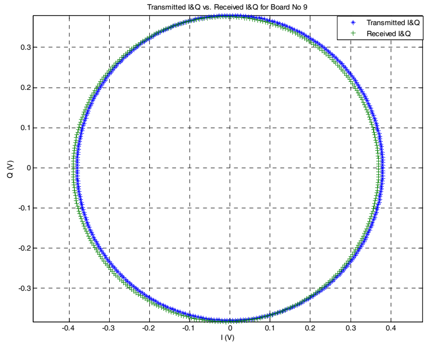
Figure F-15. Transmitted I and Q vs. received I and Q values for Board 9.
