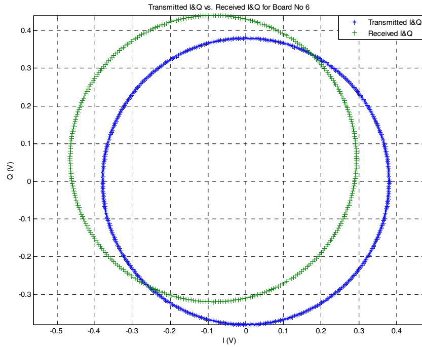
Figure F-11. Transmitted I and Q vs. received I and Q values for Board 6.
