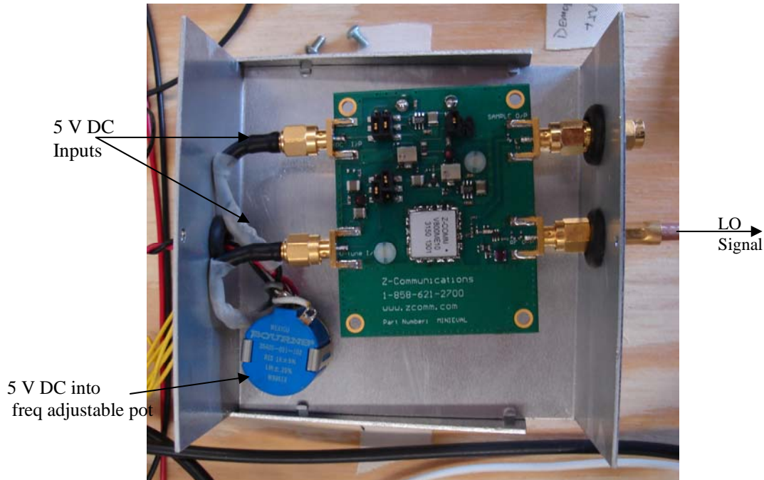
Figure 34 LO Configuration.
