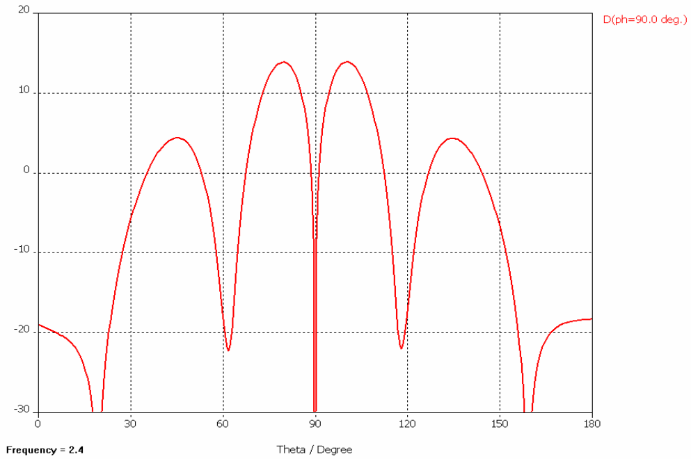
Figure 27 The difference pattern of the array of dipoles with ground plane modeled in CST Microwave Studio (broadside). [19]
