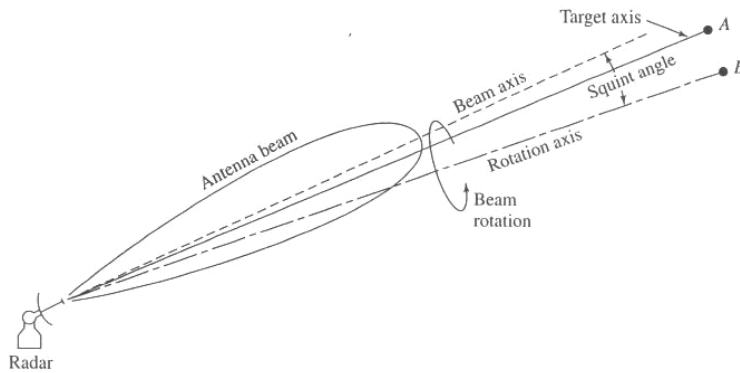
Figure 5 Conical-scan tracking. [9]
