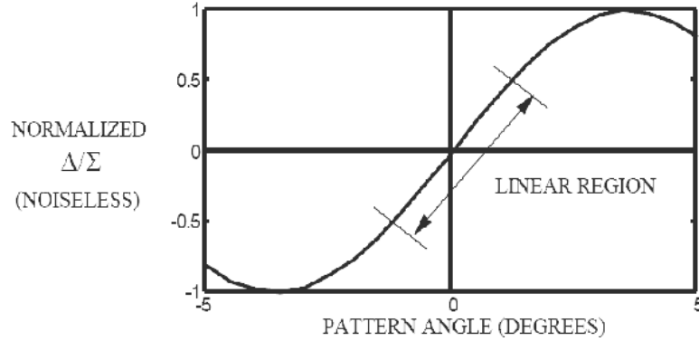
Figure 8 Normalized \Delta/\Sigma vs. pattern angle. [12]
