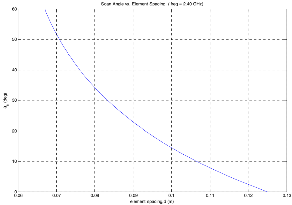
Figure 12 Element Spacing ( d ) for no grating lobes vs. Scan Angle ( \theta_s ).
