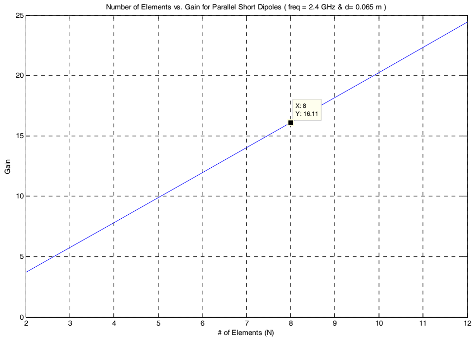
Figure 15 Gain vs. number of elements.
