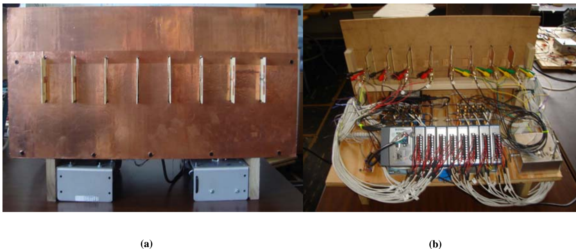
Figure 49 a) The front view of the current system configuration. b) The back view of the current system configuration.
