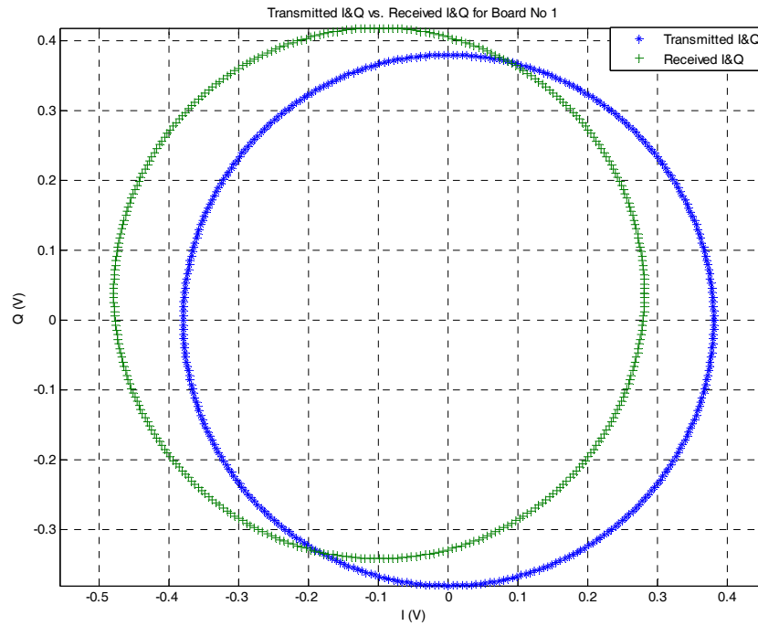
Figure F-3. Transmitted I and Q vs. received I and Q values for Board 1.
