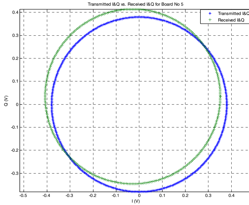
Figure F-9. Transmitted I and Q vs. received I and Q values for Board 5.
