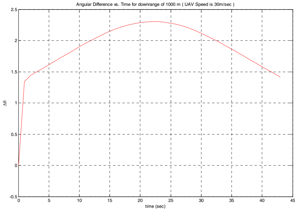
Figure 18 Angular difference (tracking error) vs. time for a UAV 1000 m downrange at a speed of 30 m/sec.
