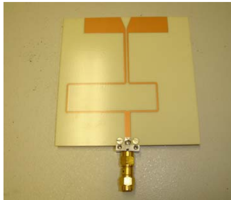
Figure 30 One of the printed circuit dipoles used in the array.
