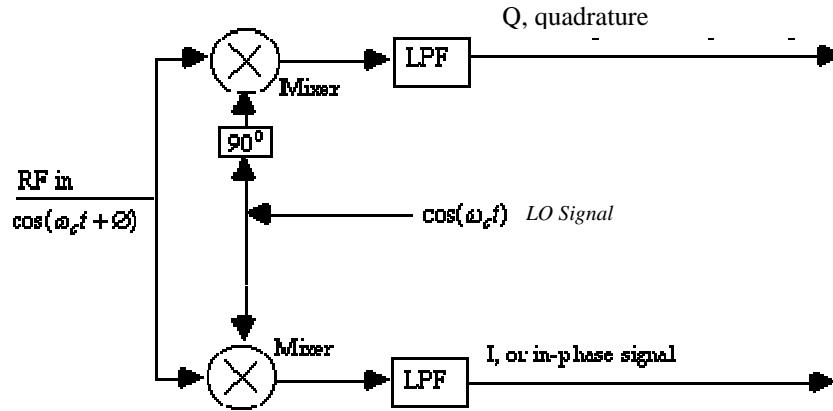
Figure 32 Quadrature demodulator recovers both the in-phase and quadrature phase components of the input signal. [21]
