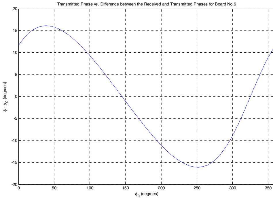
Figure F-12. Transmitted phase vs. the difference between the received and transmitted phases for Board 6.
