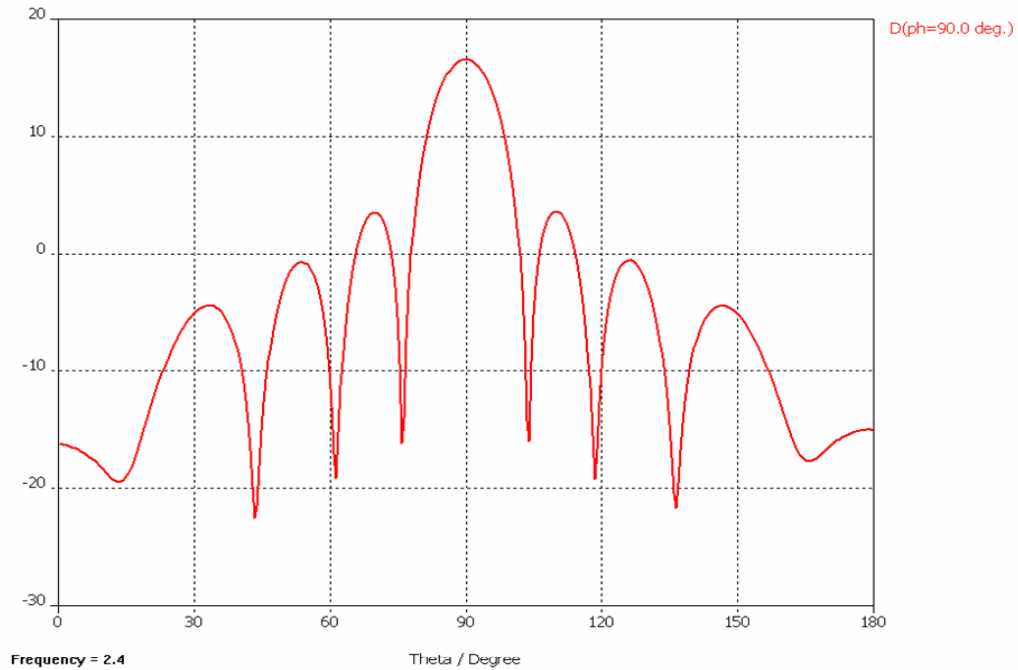
Figure 25 The sum pattern of the array of dipoles with ground plane modeled in CST Microwave Studio (broadside). [19]
