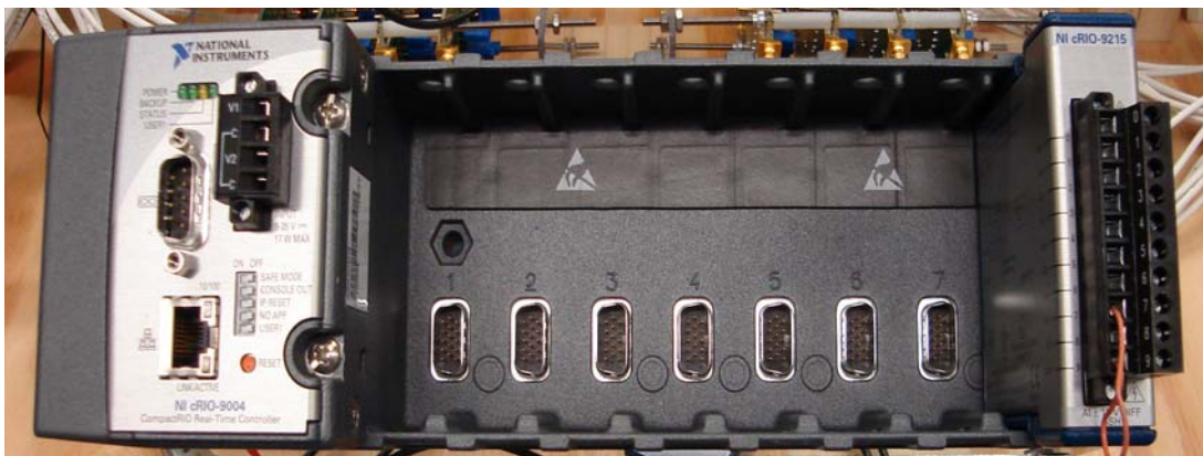
Figure 36 The reconfigurable chassis NI cRIO-9104 with the real-time embedded controller, cRIO-9004 and analog input module, NI cRIO-9215.
