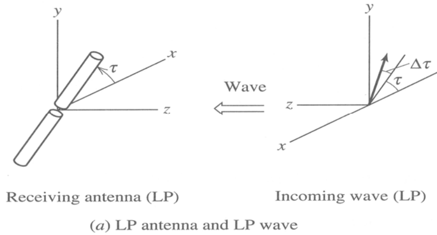
Figure 22 Illustration of reception of a linearly polarized incident wave by a linearly polarized receiving antenna. (After [15].)
