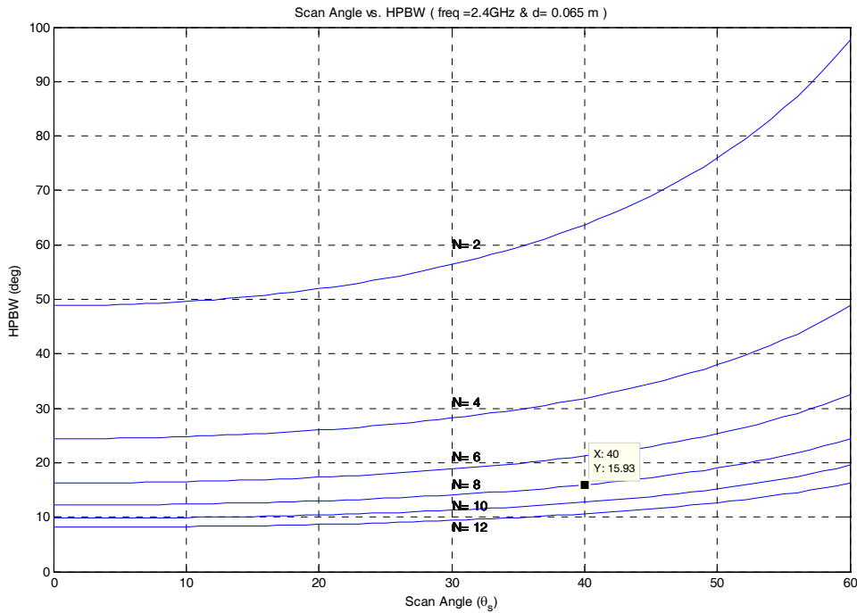
Figure 16 Scan angle ( \theta_s ) vs. half power beamwidth.
