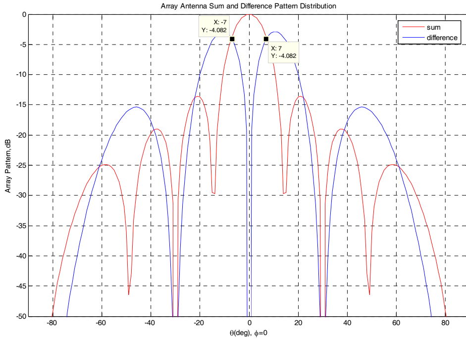
Figure 19 Array antenna sum and difference pattern distribution.
