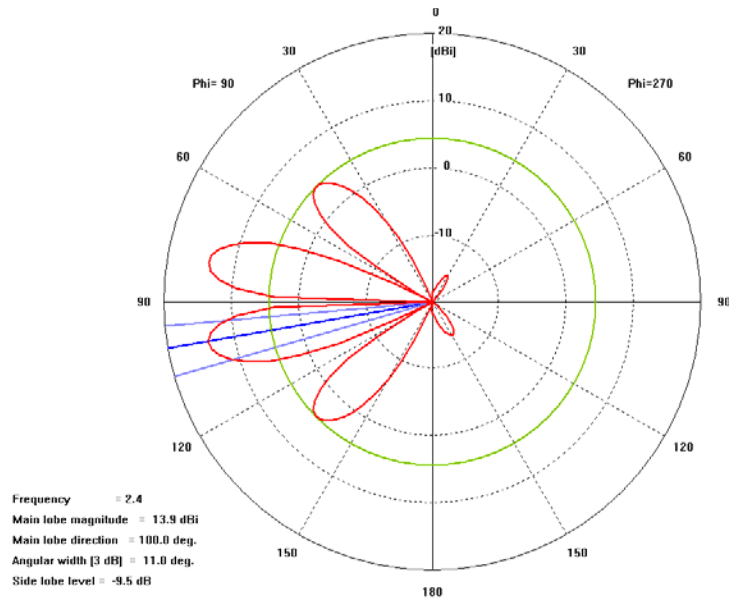
Figure E-3. The difference pattern of the array, no scan.
