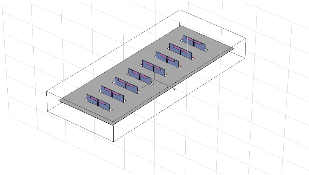
Figure 23 The top view of the ground plane and an array of dipoles modeled in CST Microwave Studio. [19]
