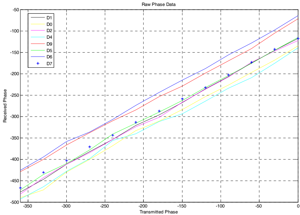
Figure 42 Transmitted phase vs. received phase for each demodulator with an LNA.
