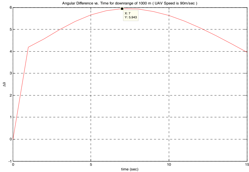
Figure 21 Angular difference (Tracking Error) vs. time for a UAV downrange 1000 m at a UAV speed of 90 m/sec.
