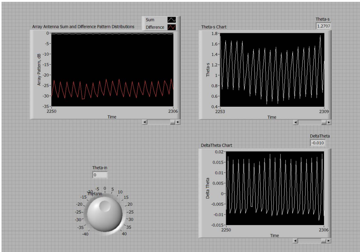
Figure 48 The front panel of host VI showing array sum and difference amplitudes (left), beam scan angle (upper right) and pointing correction (lower right).
