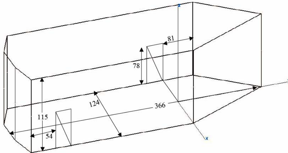
Figure 40 Specification of the anechoic chamber at the Naval Postgraduate School, Monterey, CA (Spanagel Hall Room 604) [27]
