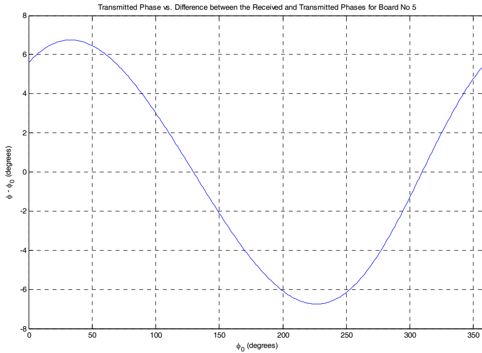
Figure F-10. Transmitted phase vs. the difference between the received and transmitted phases for Board 5.
