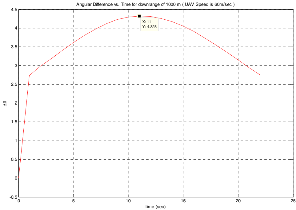
Figure 20 Angular difference (Tracking Error) vs. time for a UAV 1000 m at a speed of 60 m/sec.
