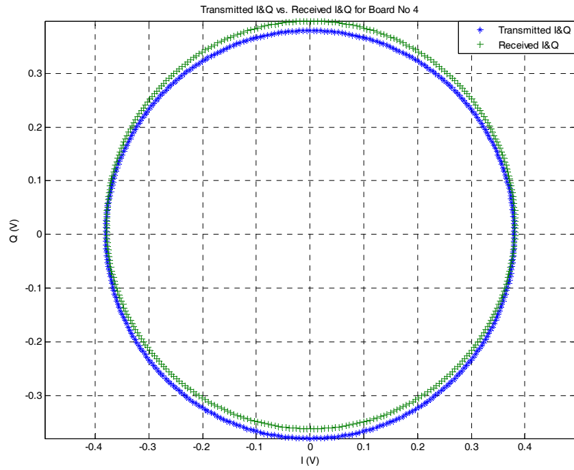
Figure F-7. Transmitted I and Q vs. received I and Q values for Board 4.
