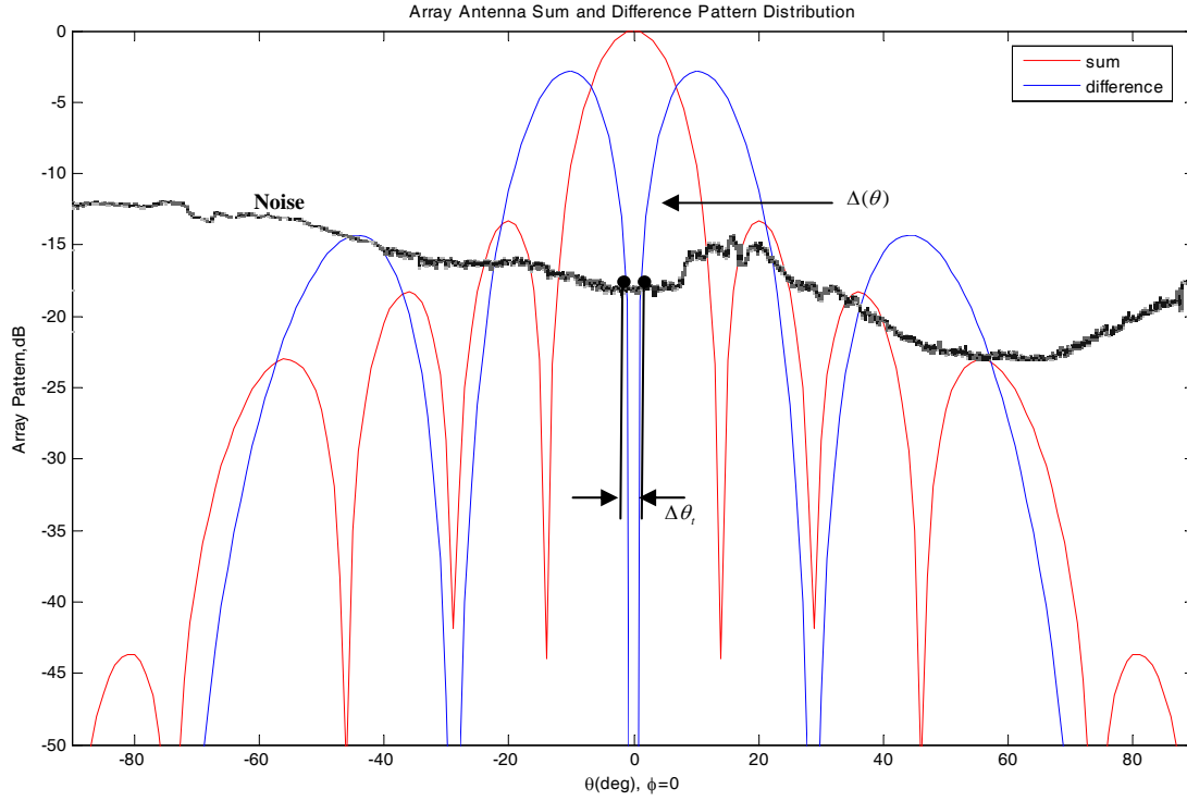
Figure 9 Noise contribution to the monopulse pattern. Half power beamwidth is entered as 16 degrees.
