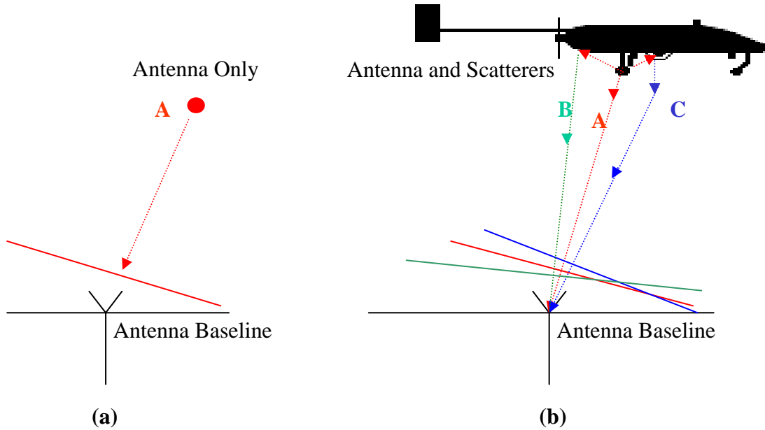
Figure 10 (a) Plane wave from A incident on the antenna. (b) Plane waves from three different sources incident on the antenna. (After [9].)
