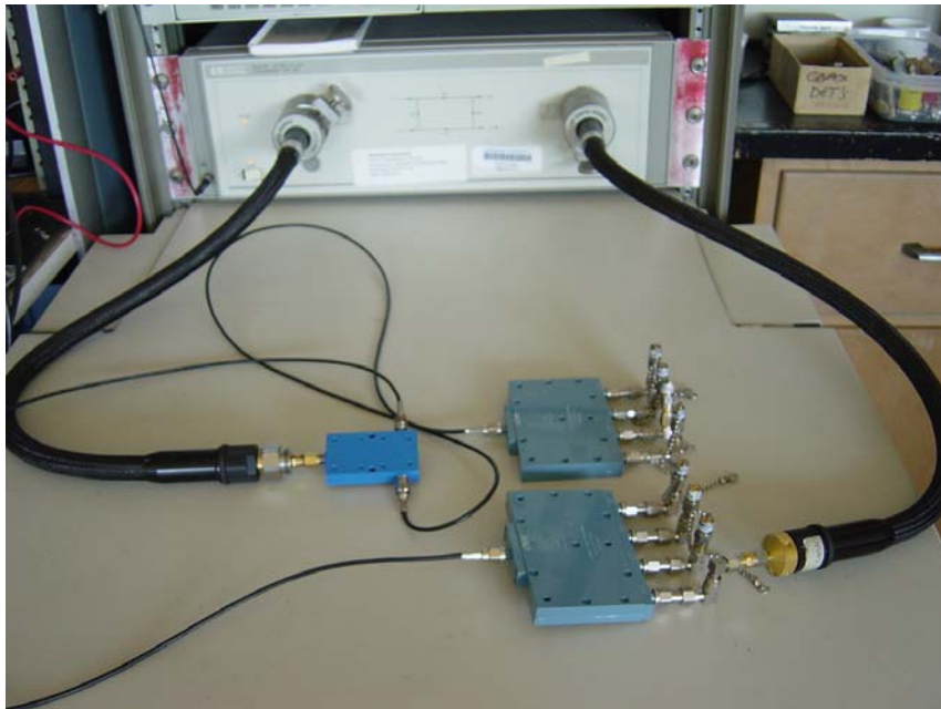
Figure 39 The setup for deviation from linear phase measurement for 4-way splitters.
