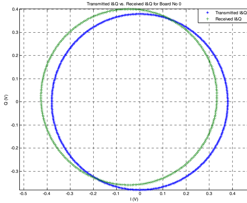
Figure F-1. Transmitted I and Q vs. received I and Q values for Board 0.
