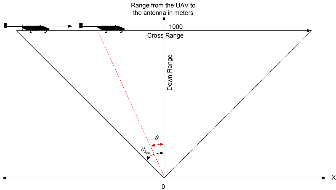
Figure 17 UAV tracking by the array located at x=0 .
