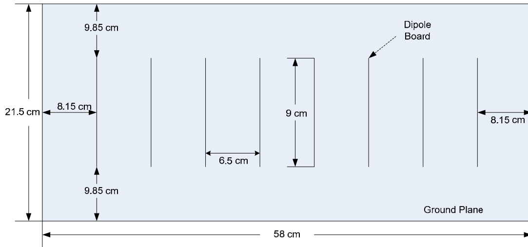
Figure 14 Drawing of the array and ground plane.
