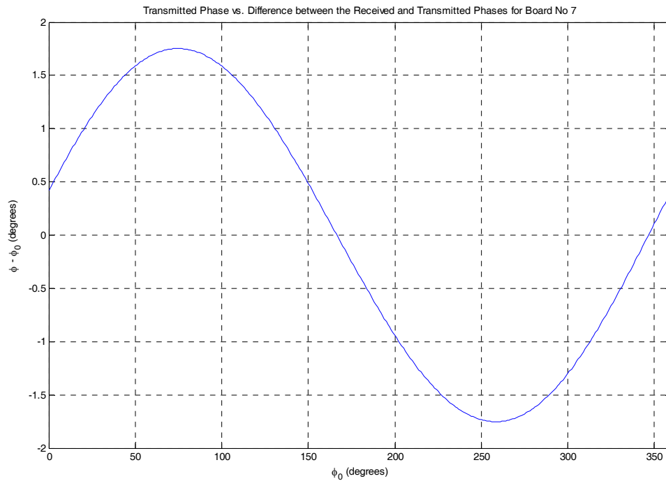
Figure F-14. Transmitted phase vs. the difference between the received and transmitted phases for Board 7.
