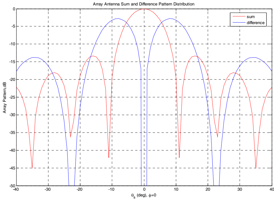
Figure 46 Calculated array antenna sum and difference pattern distributions for broadside excitation when the beam is scanned.
