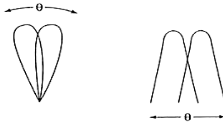
Figure 6 Two squinted antenna beams in polar and rectangular coordinates. (After [9].)
