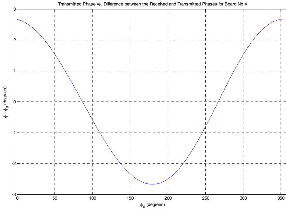
Figure F-8. Transmitted phase vs. the difference between the received and transmitted phases for Board 4.
