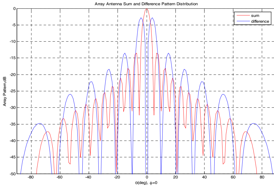
Figure 7 The sum and difference patterns of an array antenna.
