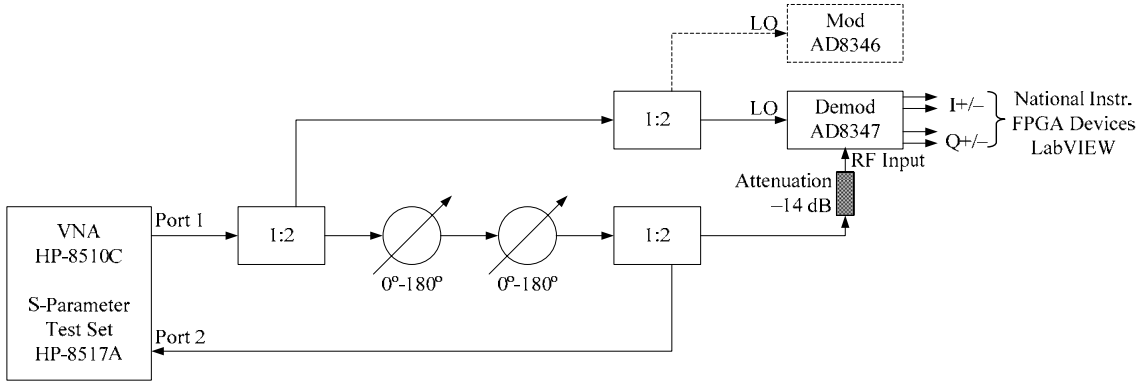
Figure 37 The demodulator setup. [25]
