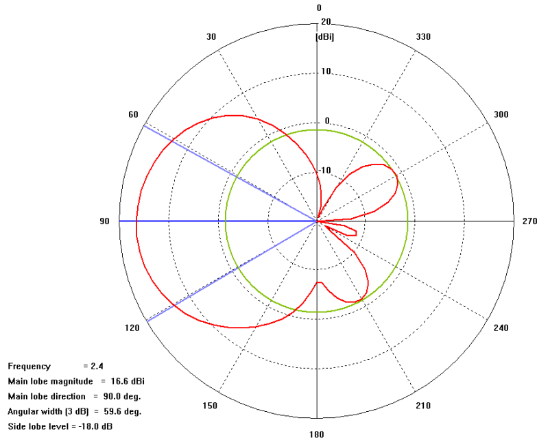
Figure E-1. The E-Plane of the array.
