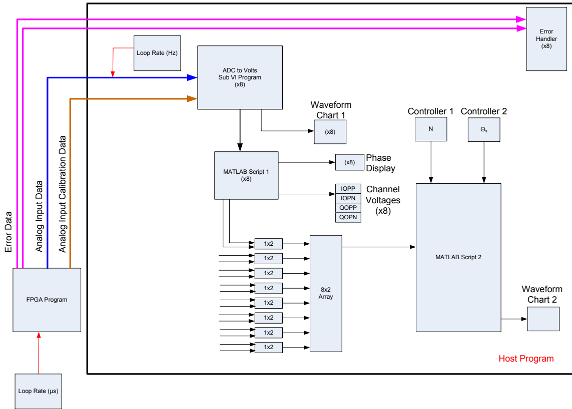
Figure 41 LabVIEW Software Data Flow Diagram.
