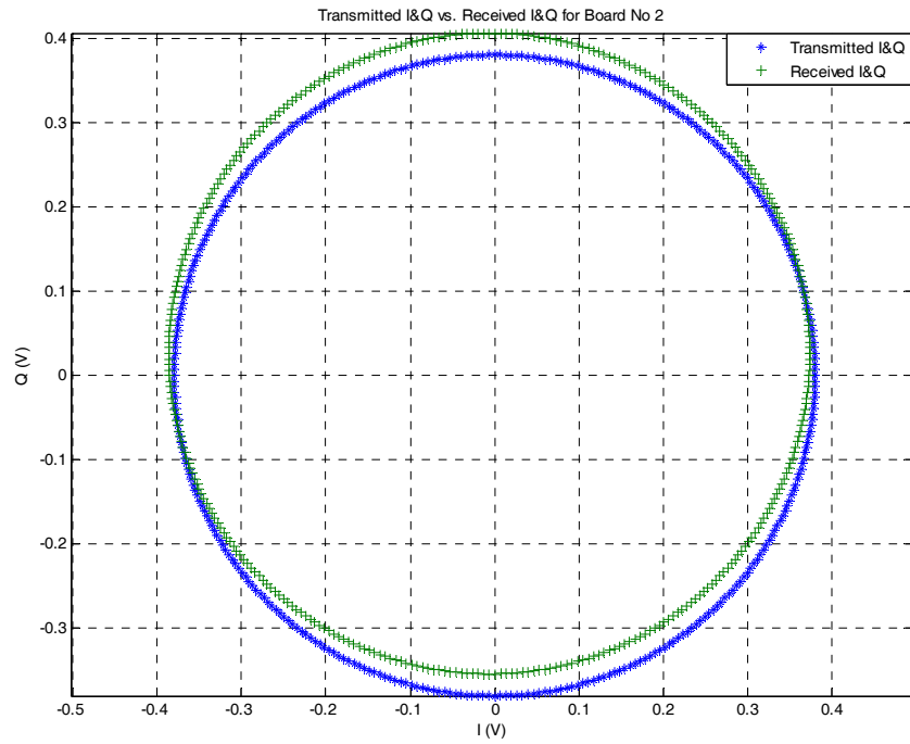
Figure F-5. Transmitted I and Q vs. received I and Q values for Board 2.
