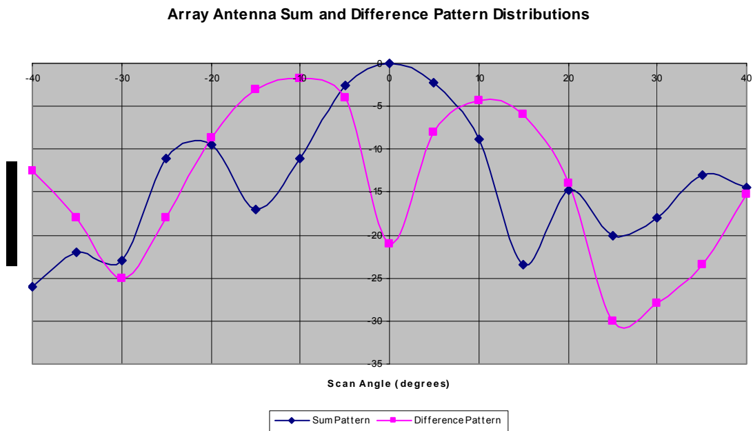
Figure 45 Measured array antenna sum and difference pattern distributions for broadside excitation when the beam is scanned.
