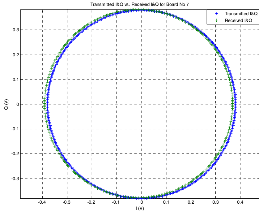
Figure F-13. Transmitted I and Q vs. received I and Q values for Board 7.
