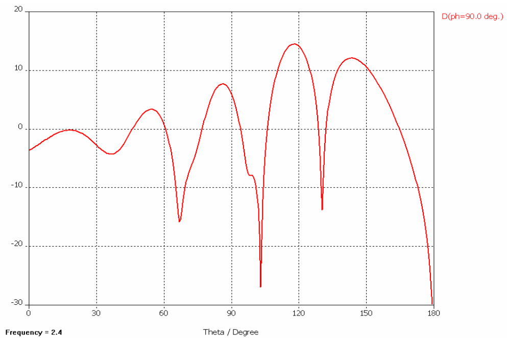
Figure 28 The scanned difference pattern of the array of dipoles with ground plane modeled in CST Microwave Studio, scanned 40° from broadside. [19]
