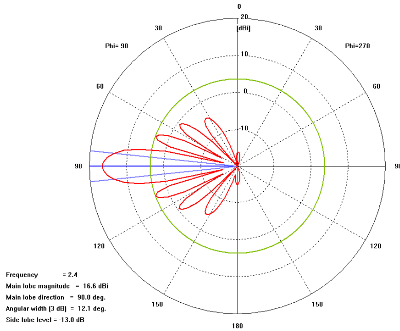
Figure E-2. The sum pattern of the array, no scan.
