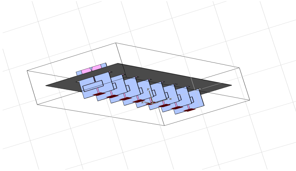
Figure 24 The bottom view of the ground plane and an array of dipoles modeled in CST Microwave Studio. [19]
