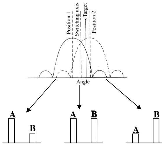
Figure 4 The outputs of a lobe-switching antenna pattern. (After [9].)
