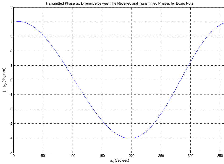
Figure F-6. Transmitted phase vs. the difference between the received and transmitted phases for Board 2.
