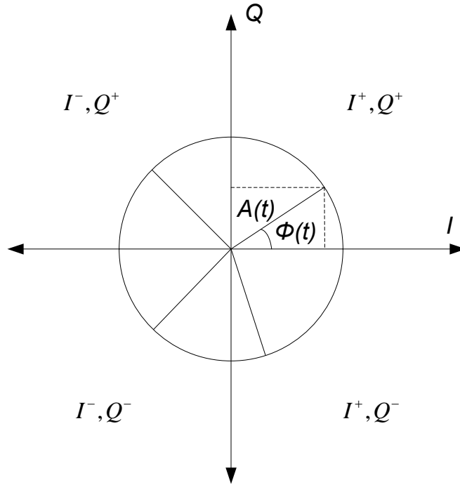
Figure 38 Phasor In-phase and Quadrature-Phase plane.
