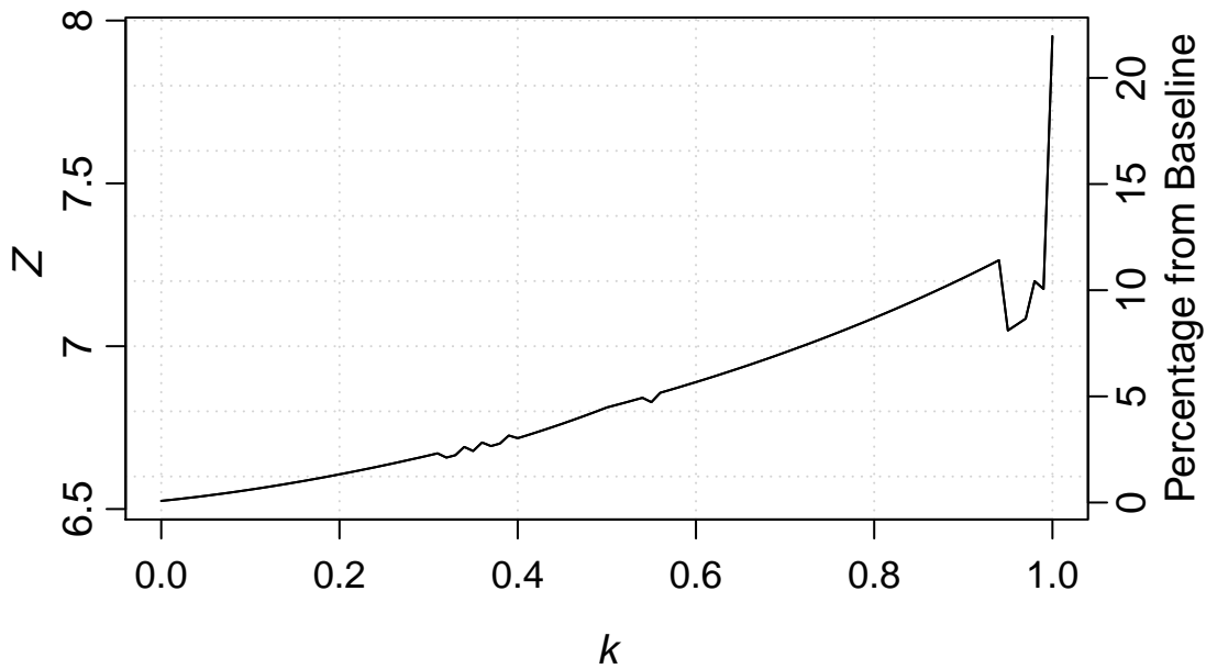
Figure 4.5: Objective value of the robust formulation for optimistic demands as a function of k .
