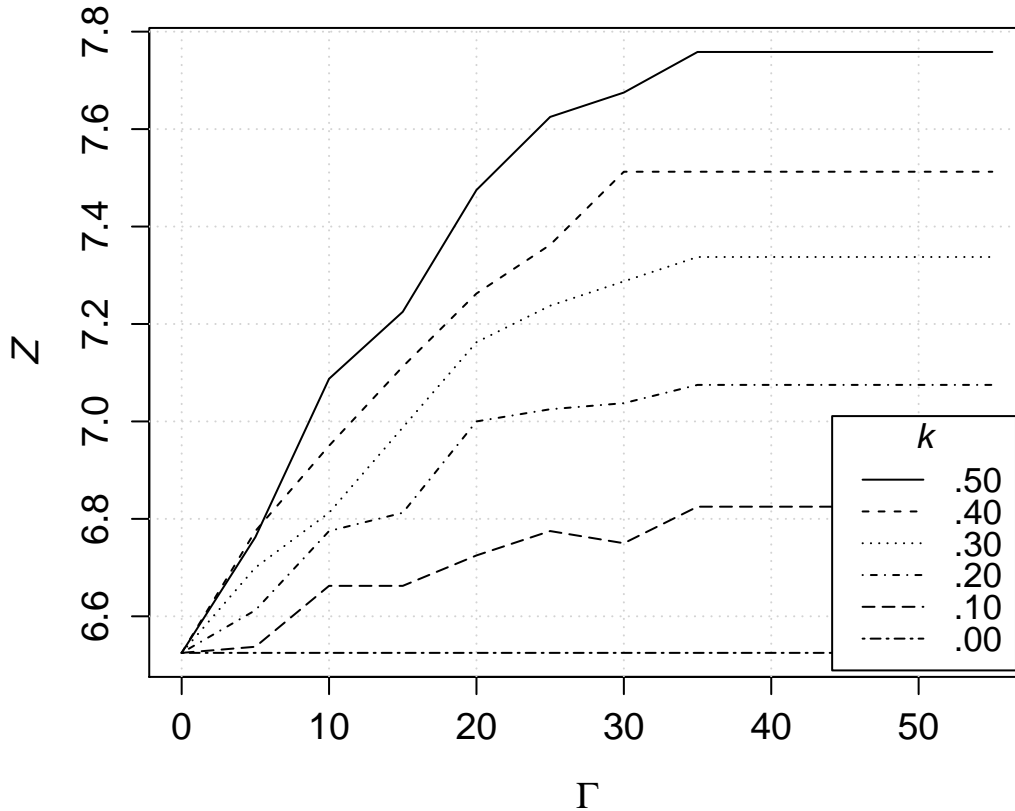
Figure 4.7: Objective value of the robust formulation for optimistic budgets as a function of \Gamma for various k values.
