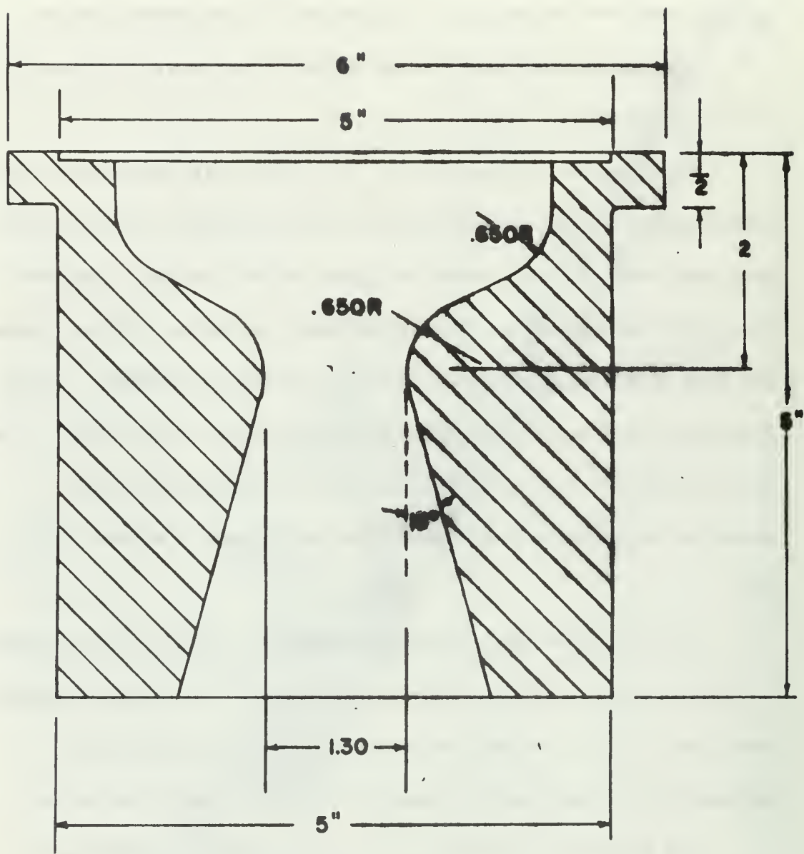
FIGURE 21. NOZZLE
