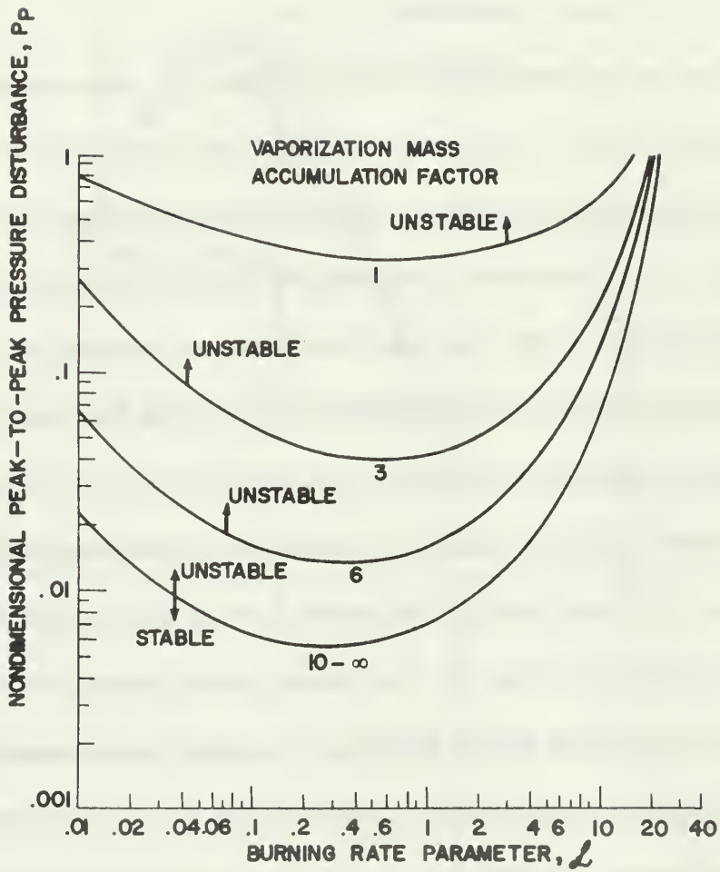
FIGURE 2. INSTABILITY BOUNDARIES FOR VAPORIZATION MODEL [ REF. 3 ]
