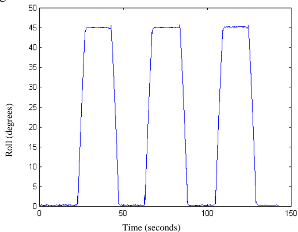
Figure 8: 45 Degree Roll Excursions at 10 deg/sec
