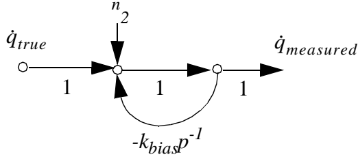
Figure 6: Bias Estimation Filter SFG [15]
