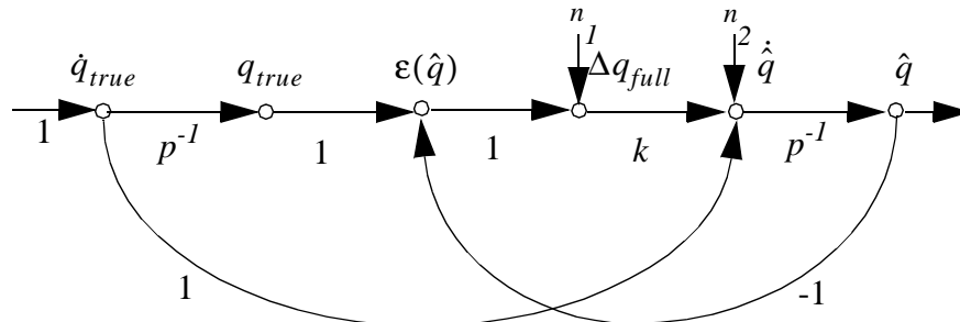
Figure 2: Signal Flow Graph for Linearized System [15]
