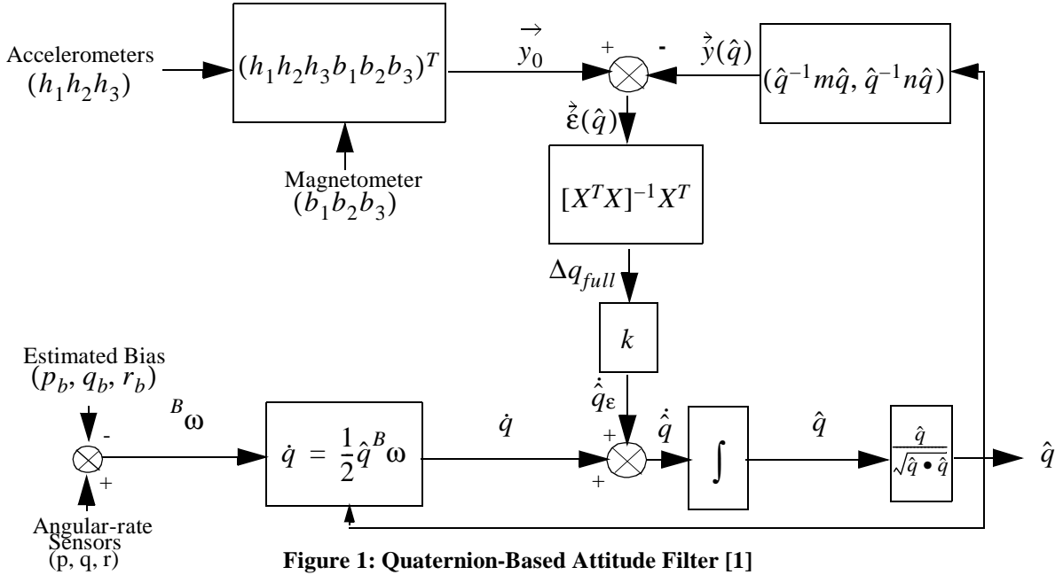
Figure 1: Quaternion-Based Attitude Filter [1]
