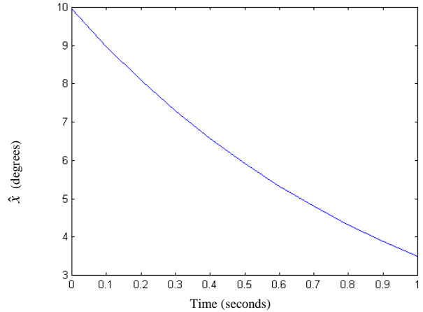
Figure 5: Simulated Nonlinear Filter Response, 10 Degree Offset, \alpha=0.1 , \Delta t=0.1 [7]
