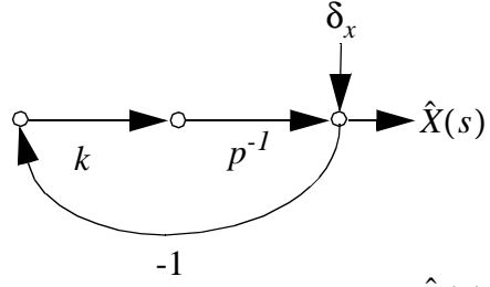
Figure 4: Transform Domain SFG, \hat{X}(s) [16]
