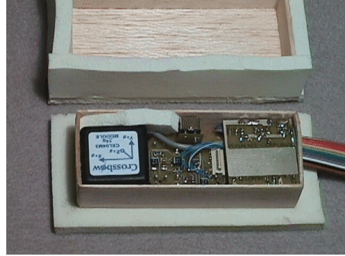
Figure 7: Prototype Nine-axis Inertial Sensor [18]
