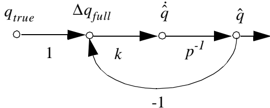
Figure 3: Simplified SFG, Static Testing, Zero Noise [16]
