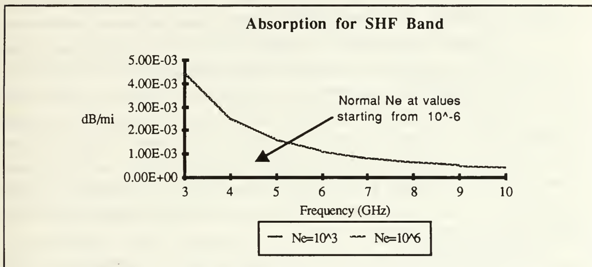
Figure 3.8 D-Region Absorption
