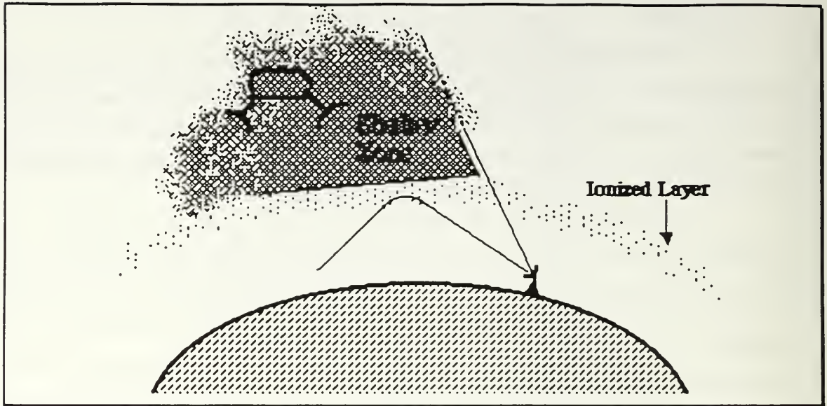
Figure 3.7 Shadow Zone
