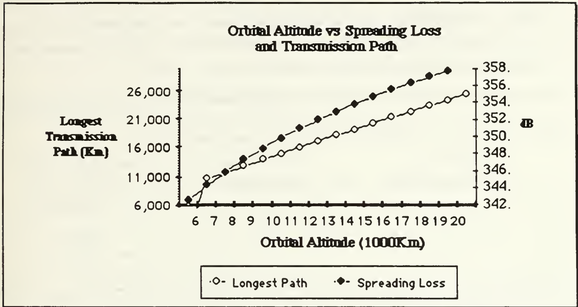
Figure 4.4 Spreading Loss vs Orbital Altitude
