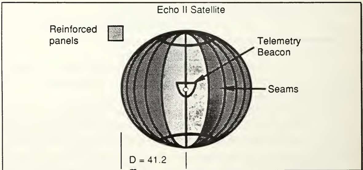
Figure 2.1 Physical Characteristics of the Echo II
