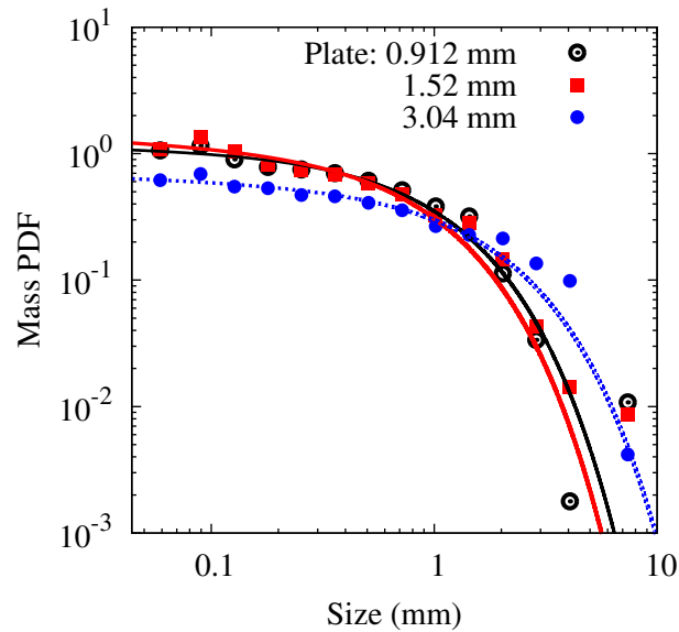
Figure 4: Mass PDF for impact at 1829 m/s on plates of varying thickness. All distributions converge to a similar trend at this impact velocity.
