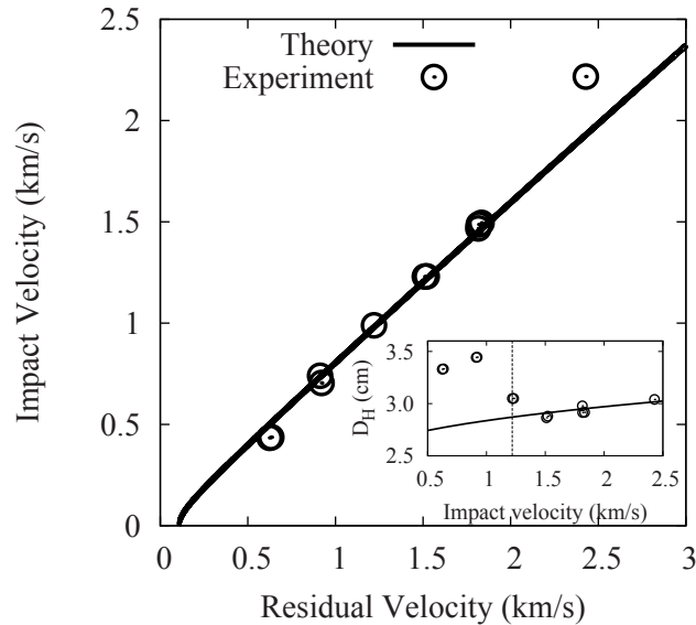
Figure 1: Residual velocity of the debris cloud as a function of initial impact velocity.
