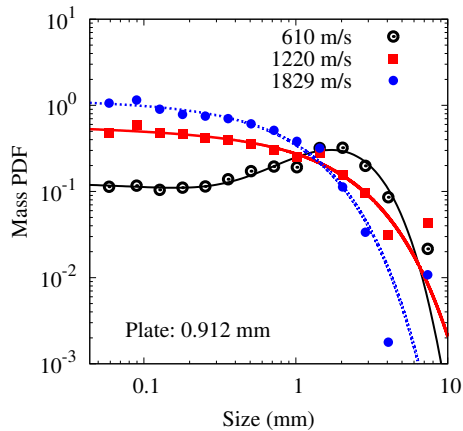
Figure 2: Log-scale mass probability density function (PDF) for fragments generated by impact on a 0.912 mm plate.
