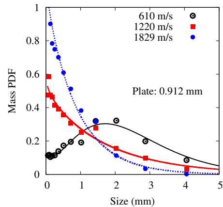
Figure 3: Linear-scale mass PDF for impact on a 0.912 mm plate. Fits are based on equations described in the text.
