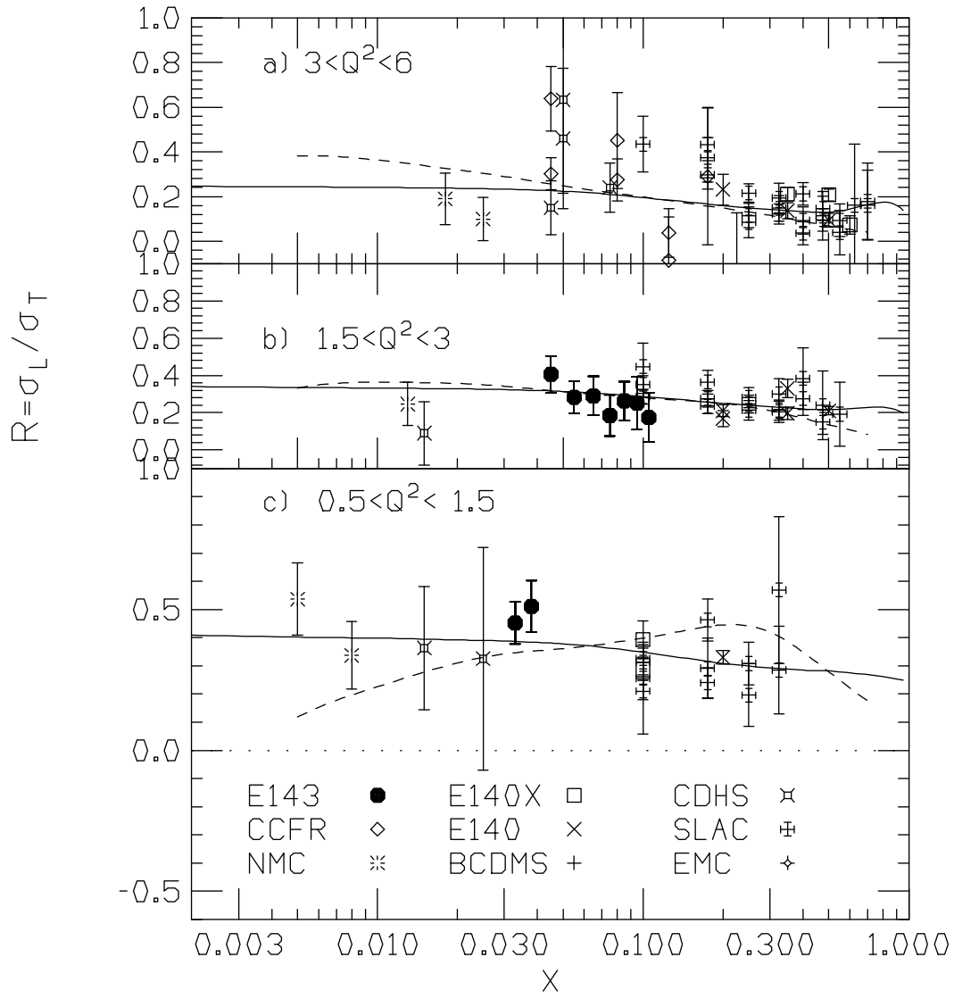
FIG. 4. R as a function of x for: a) 3 \leq Q^2 \leq 6(\text{GeV}/c)^2 ; b) 1.5 \leq Q^2 \leq 3(\text{GeV}/c)^2 ; c) 0.5 \leq Q^2 \leq 1.5(\text{GeV}/c)^2 . The solid curve is the average of the new fits, R_{1998} , and the dashed curve is the NNLO pQCD calculation described in the text.
