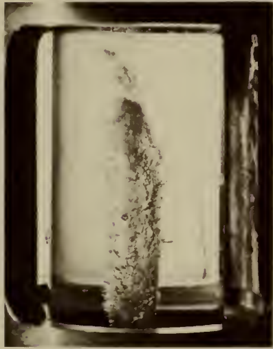
Fig. 25. Freon cavity. T=97.0^{\circ}\text{F} , v=17.45 ft/sec, l=13/8 in.
