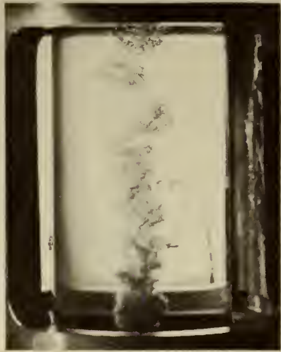
Fig. 18. Freon cavity. T=96.0^{\circ}\text{F} , v=17.52 ft/sec, l=13/16 in.
