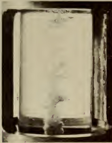
Fig. 21. Freon cavity. T=122.4^{\circ}\text{F} , v=14.07 ft/sec, l=13/16 in.
