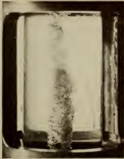
Fig. 26. Freon cavity. T=122.0^{\circ}\text{F} , v=14.70 ft/sec, l=13/8 in.
