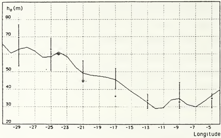
Fig. 8. Model results for the equator. (a) Zonal variation of the nondimensional mixed layer depth H_* . (b) Zonal variation of the Kraus and Turner diagnostic mixed layer depth h_0 . The circles represent observed values, while the small squares represent interpolated values. The vertical bars show the effect of varying the surface heat flux Q_0 by \pm 10 \text{ W/m}^2 . The shaded areas in (a) correspond to the zones where a one-dimensional, steady-state balance is assumed impossible.
