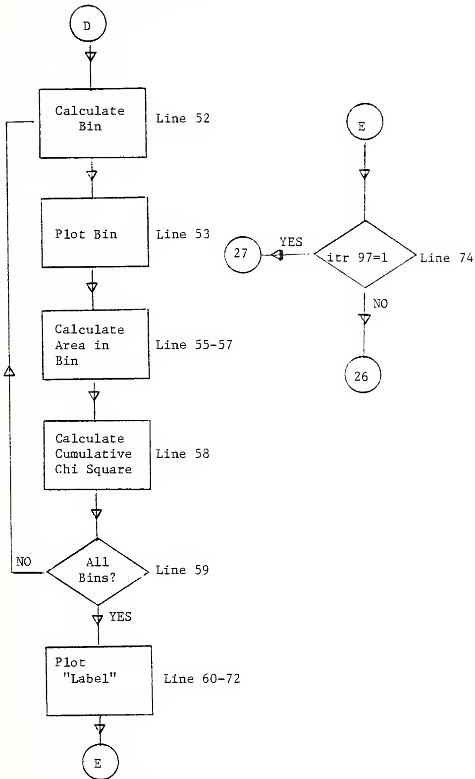
Figure 6D. Data Analysis Program
