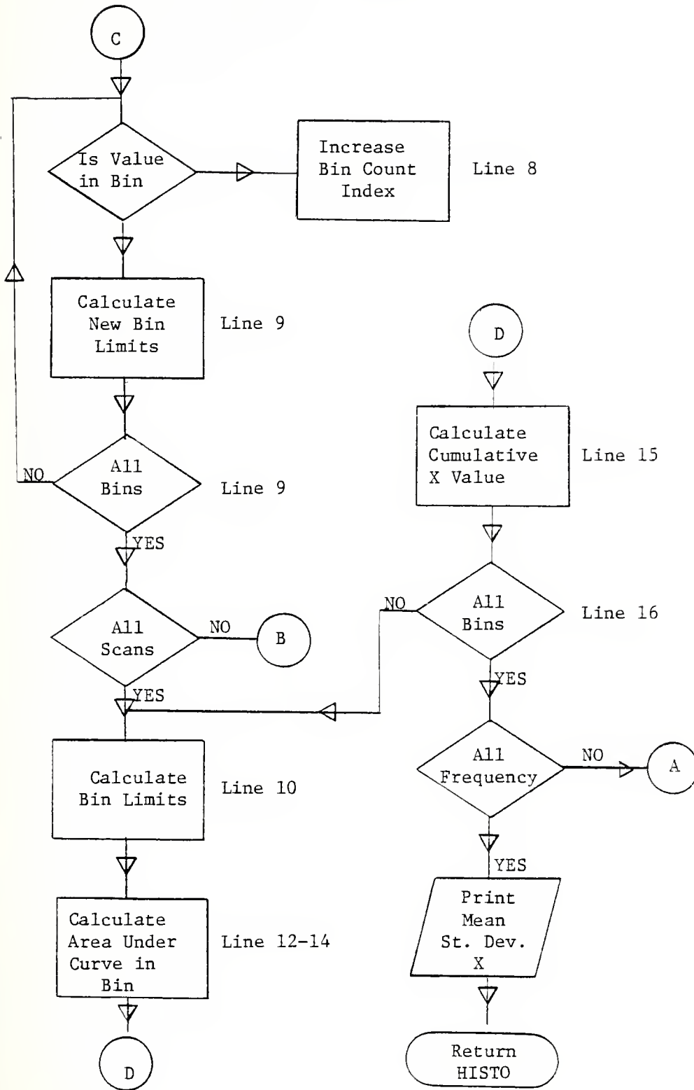
Figure 8B. Data Summary Program
