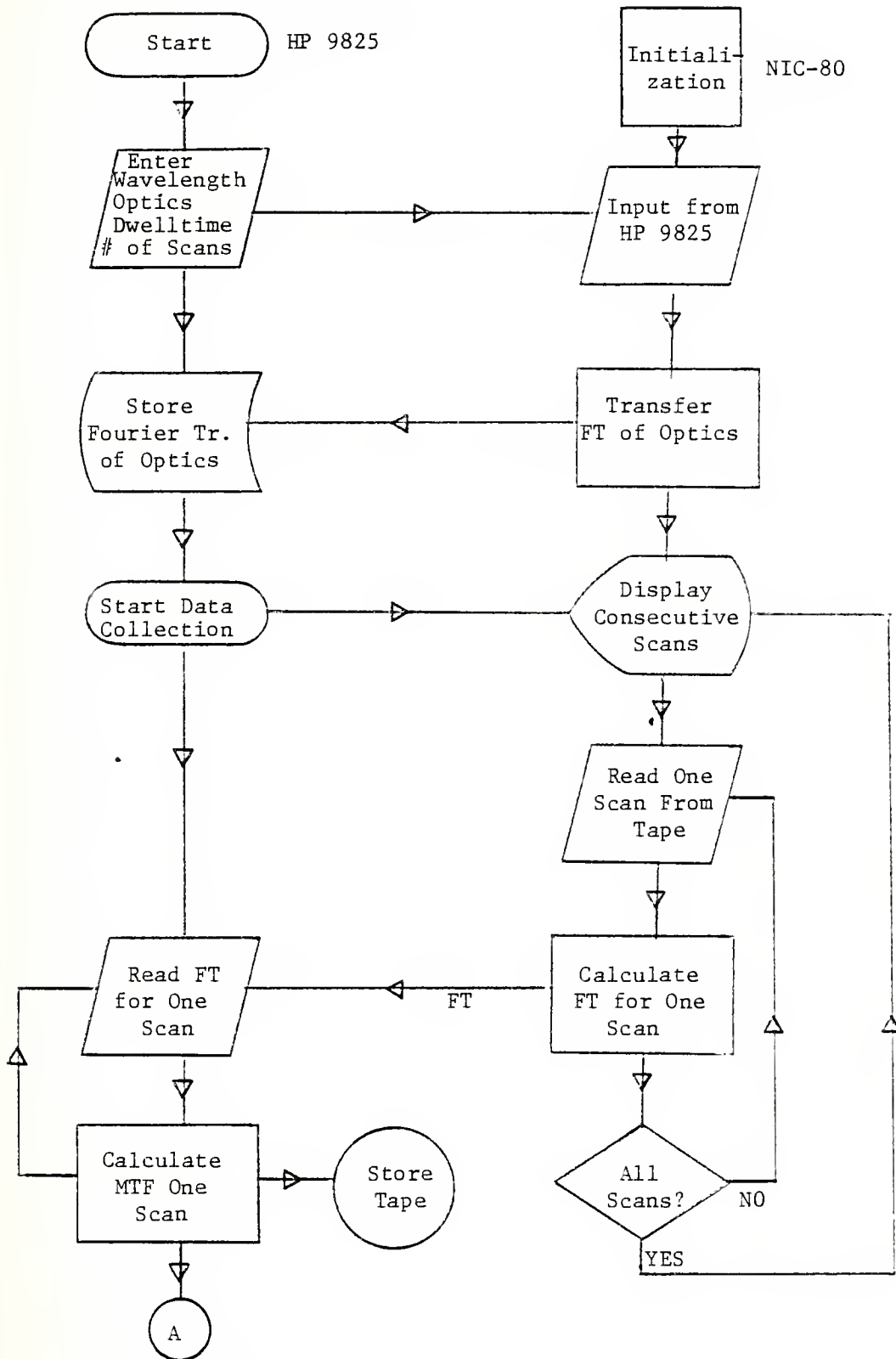
Figure 5A. Program Organization
