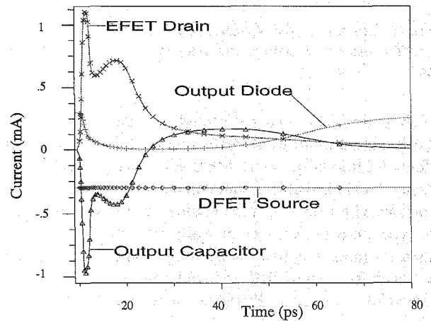
Figure 4: Currents of the E-FET drain, gate diode, capacitor and active load.
