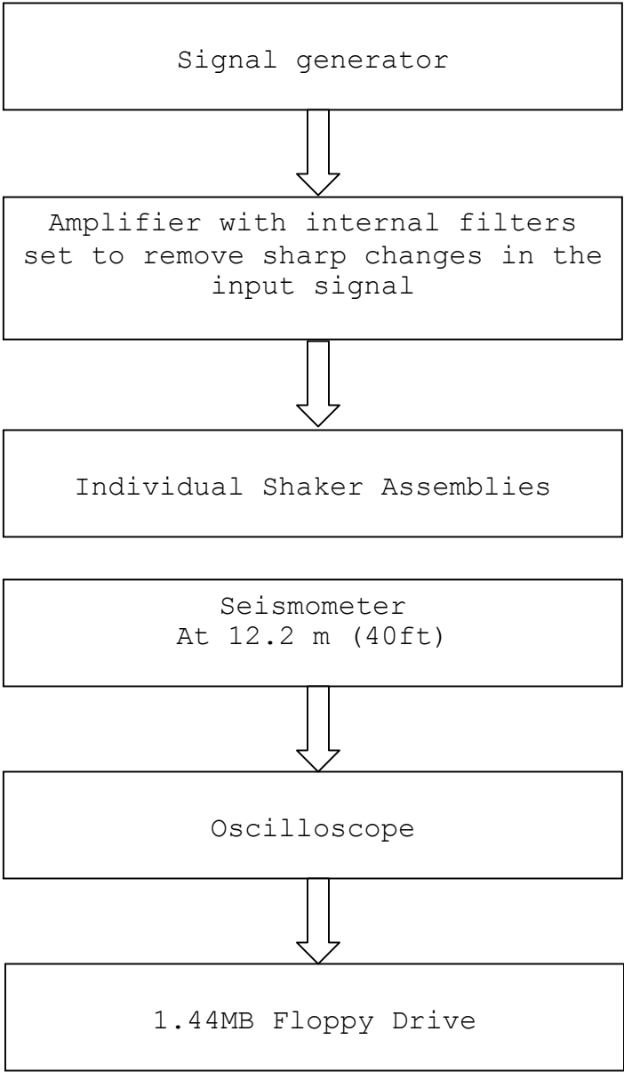
Figure 17. Field testing electronics setup
