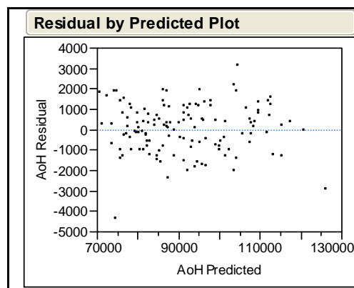
Figure 18. Selected model residual plot
