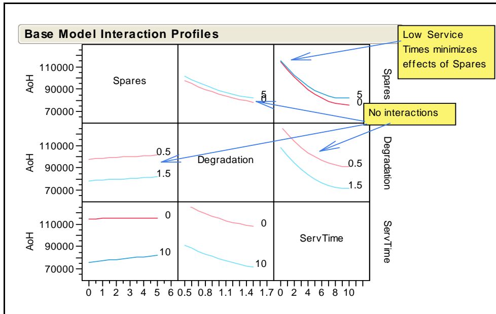
Figure 20. Main model graphical interactions
