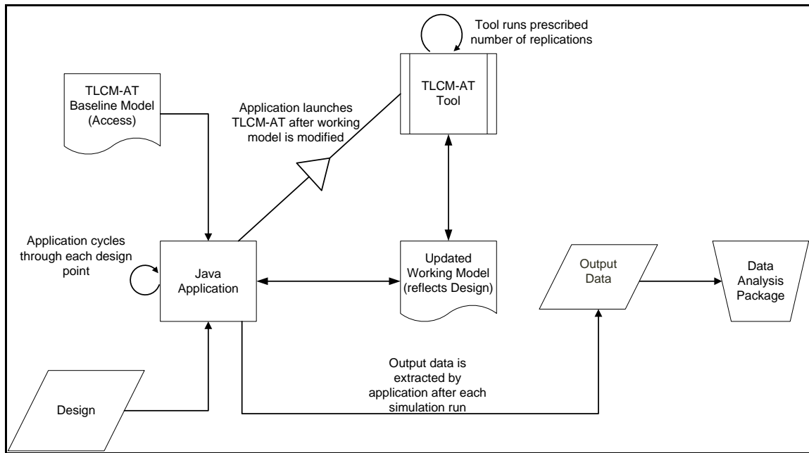
Figure ES-1. Data generation process using Java application
