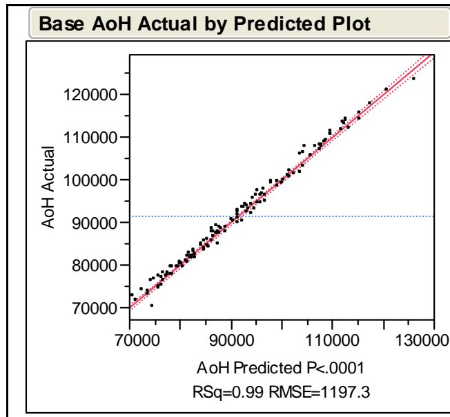
Figure 19. AoH actual versus predicted plot
