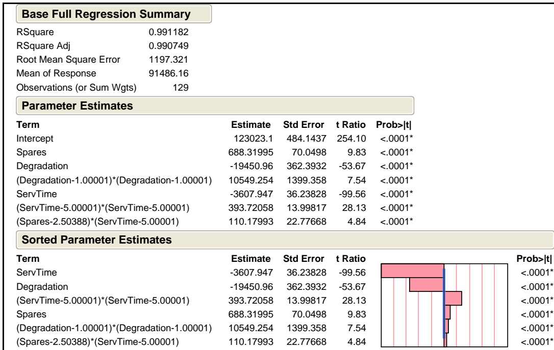
Figure 17. Selected predictive model
