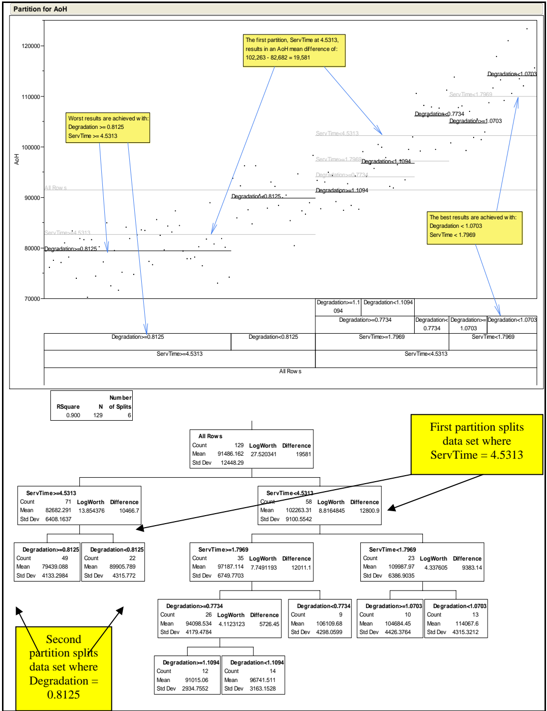
Figure 21. AoH data partition
