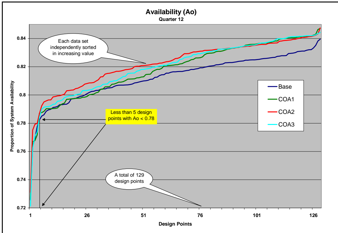
Figure 6. Percent of systems available to operate during the 12 th quarter [Best viewed in color]
