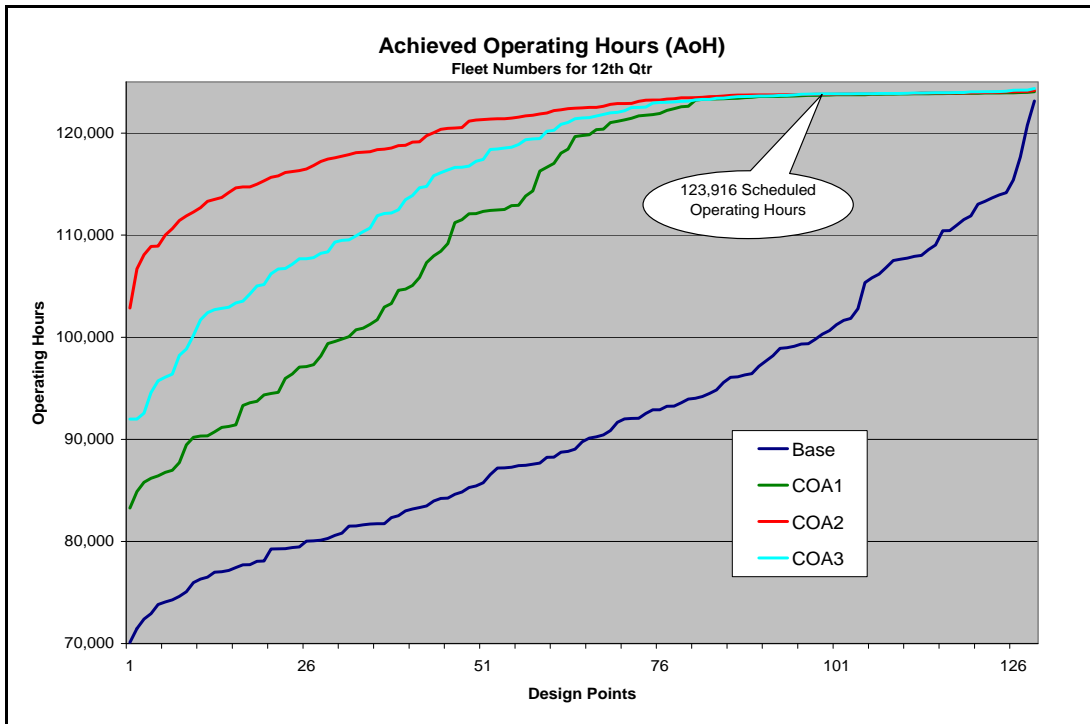
Figure 7. Achieved operating hours [Best viewed in color]
