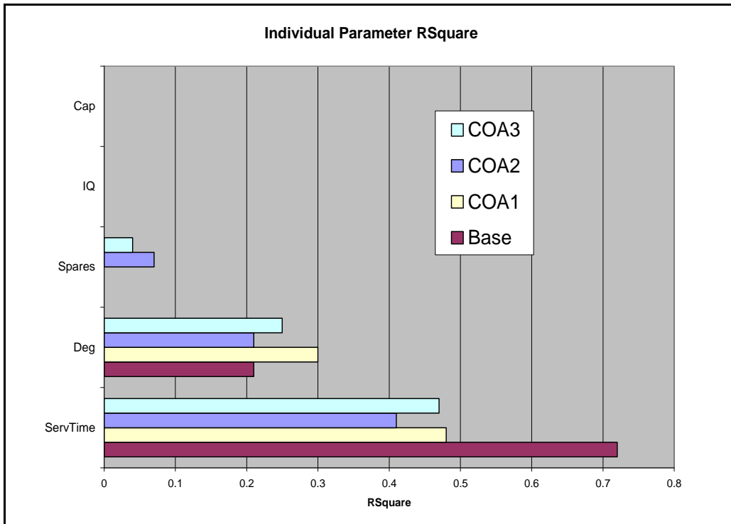
Figure 13. Variability explained by each individual factor without interactions [Best viewed in color]
