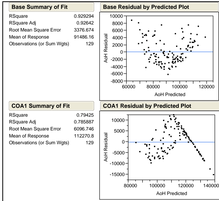
Figure 14. Base and COA1 main parameter model
