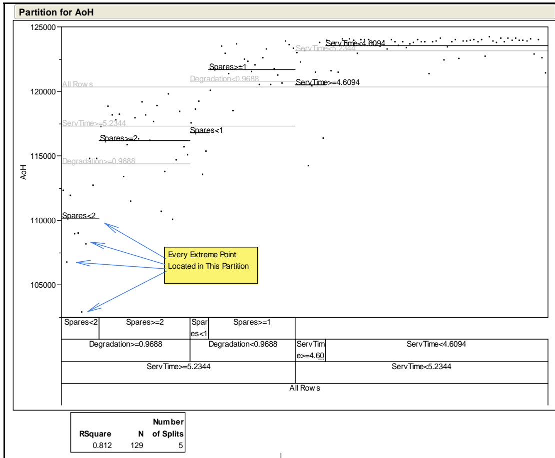
Figure 22. COA2 AoH data partition
