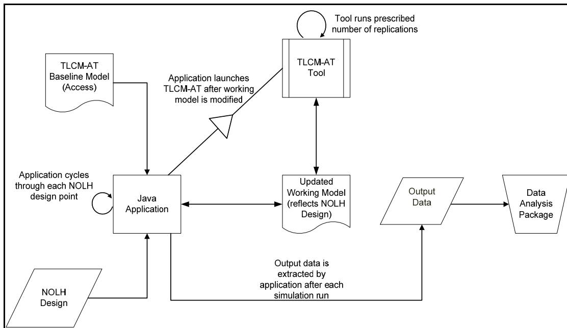
Figure 3. Data generation process
