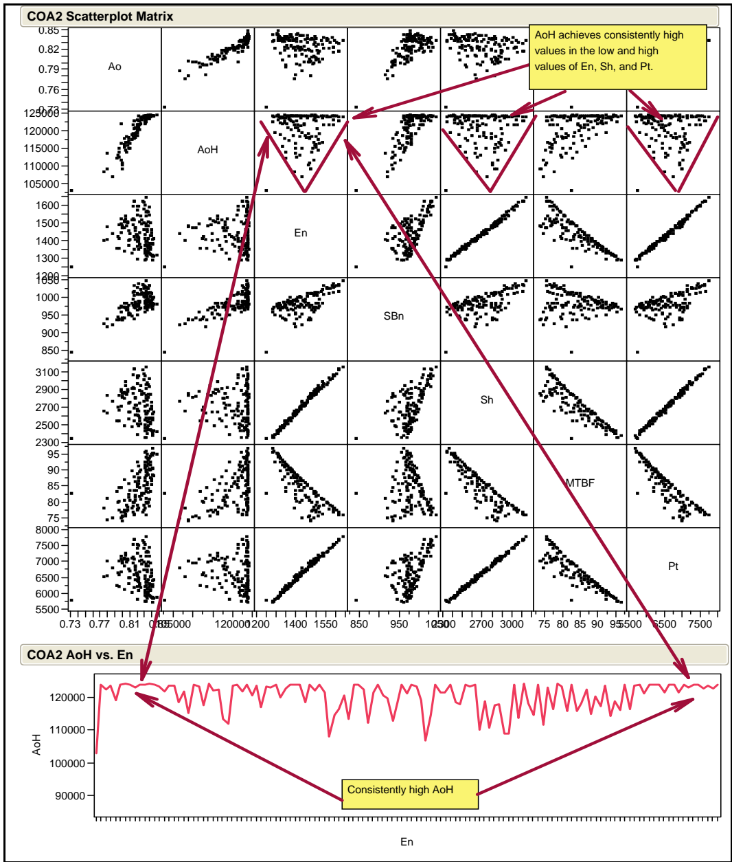
Figure 10. COA2 MOE scatter plot matrix [Best viewed in color]
