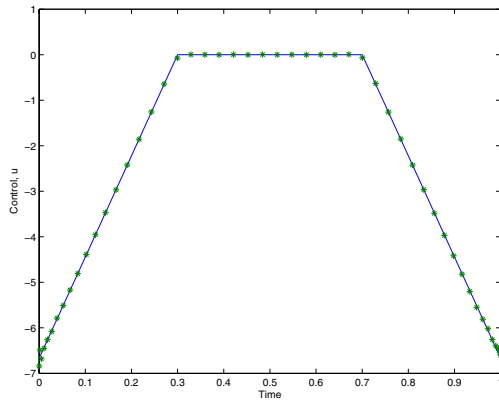
Fig. 3. PS control, u . Solid line is analytical.
