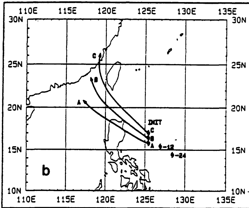
Fig. 5.5. Sensitivity of WPCLPR model to (a) initial longitude and (b) changes in past motion. (Englebretson, 1992)
