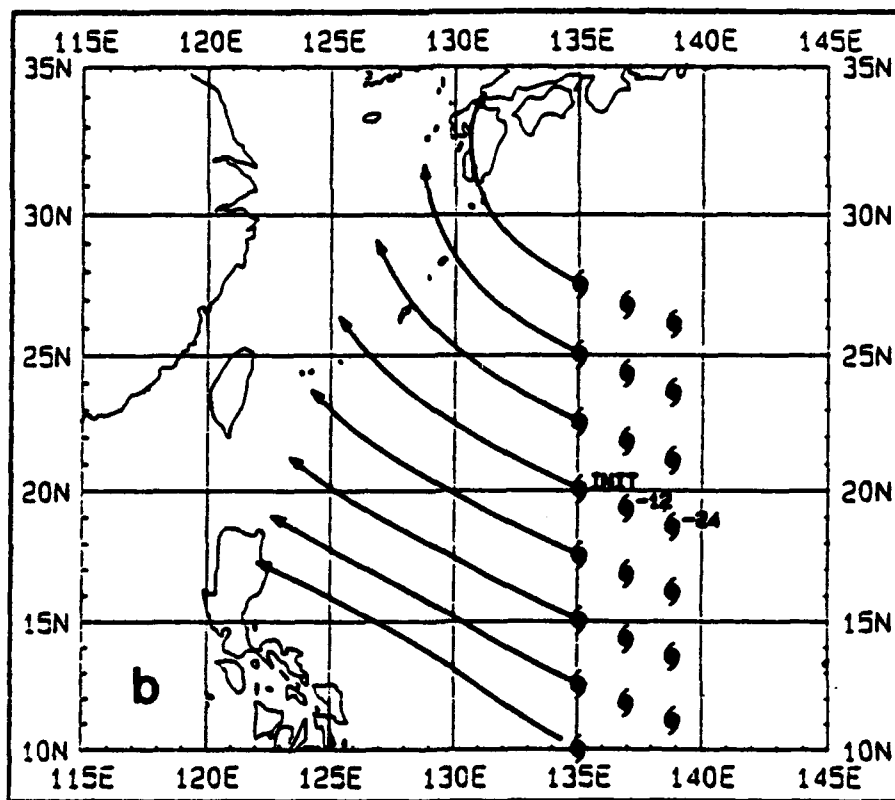
Fig. 5.4. Sensitivity of WPCLPR model to (a) time of year and (b) initial latitude. Shown are 72-h forecast tracks with different initial conditions. (Englebretson, 1992)
