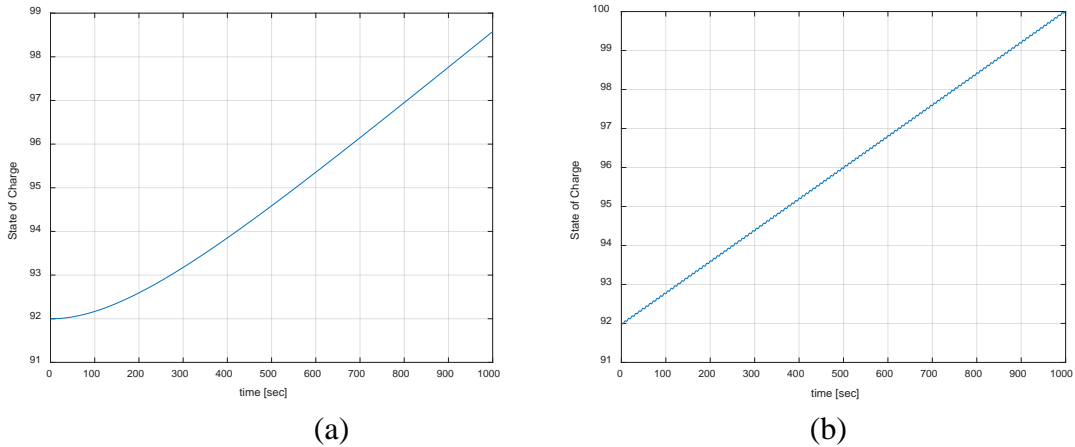
Figure 22. Batteries SOC with SCs (a) and without SCs (b) at Light Load
