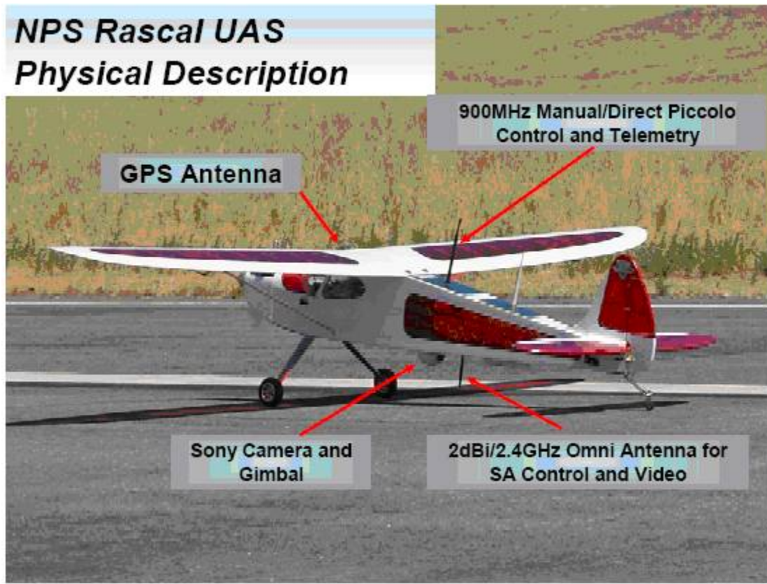
Figure 3. Rascal UAV with comm. antennas 8
