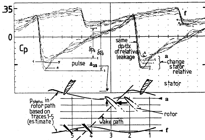
Fig. 6 Pressures at positions 1-5 for stations a and f showing the path of the stator wake deduced from the data.
