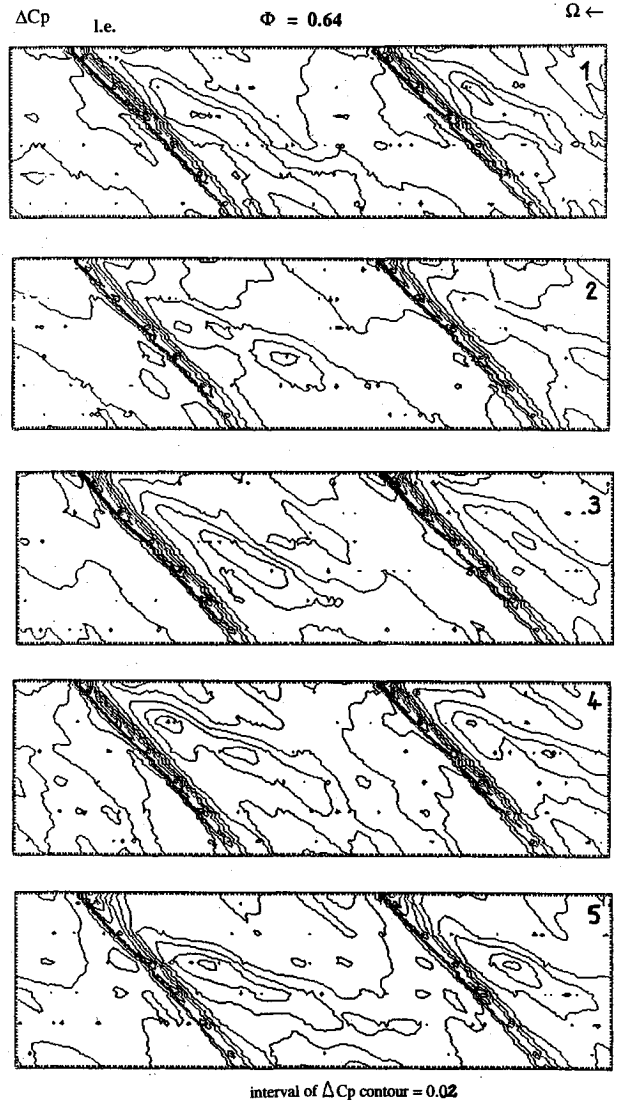
Fig. 8 Contours of the difference in pressure between clearances of e/b = 0.006 and 0.0035 for five stator relative positions. Differentials are small in the passage compared to the zone under the blade.
