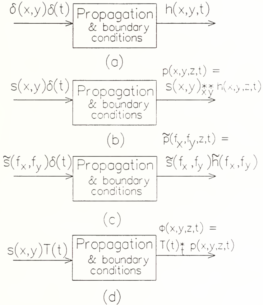
Figure 2.2: Block diagram of (a) the total impulse response h(x,y,t) , (b) the spatial impulse response p(x,y,z,t) in the space–time domain, (c) the spatial impulse response \tilde{p}(f_x, f_y, z, t) in the spatial frequency–time domain, and (d) the general solution \phi(x,y,z,t) .
