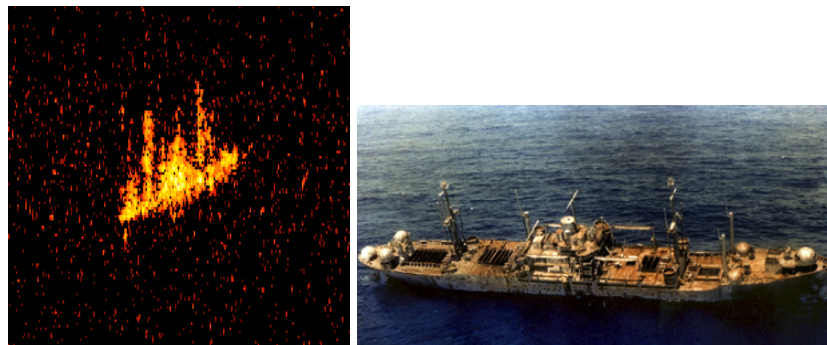
Figure 3. On the left is an ISAR image of a ship; on the right is an optical image of the same ship. (Courtesy Naval Research Laboratory)
