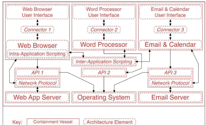
Figure 1. An OA reference model for common software component types interconnected within an integrated, cybersecure C2 system. [14]
