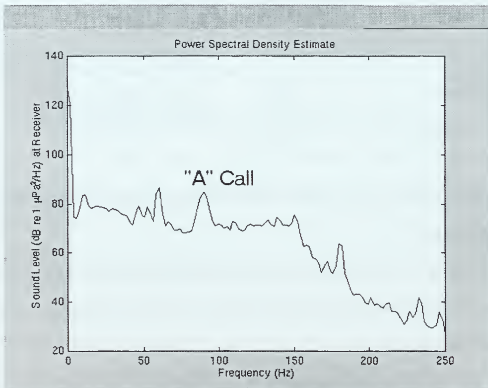
Figure 2: Power spectral density estimate for data segment containing an "A" call. A 75 dB re 1 \mu\text{Pa}^2/\text{Hz} ambient noise level is shown at low frequencies. The roll-off at 150 Hz is caused by the precision filter.
