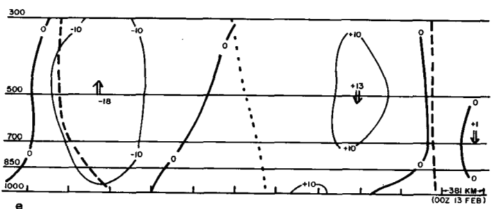
FIGURE 9.—0000 GMT February 13, 1964. (a) 850-mb. divergence and height analysis (50~1500 m.). (b) 500-mb. divergence and height analysis (22~5220 m.). (c) 300-mb. divergence and height analysis (12~9120 m.). (d) Cross section of divergence taken along line AA' in 9c. Divergence in units of 10^{-7}\text{ sec.}^{-1} . (e) Cross section of vertical velocity in units of 10^{-4}\text{ sec.}^{-1} taken along line AA' in 9c.
