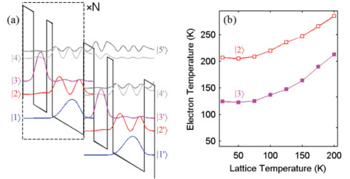
FIG. 1. (Color online) (a) Conduction band diagram of the Ref. 50 QC structure, showing the localized wave functions, extended wave function for state |4\rangle , and the quasibound continuum-like state |5\rangle used in this analysis. The diagonal optical transition is from |3\rangle \rightarrow |2\rangle ( \Delta E_{3-2} \sim 19 meV or 4.6 THz), and the lower lasing state is depopulated via fast intrawell e^- -LO phonon scattering where \Delta E_{2-1} \approx \hbar\omega_{LO} . (b) The effective electron temperature of the upper and lower lasing states as a function of lattice temperature.
