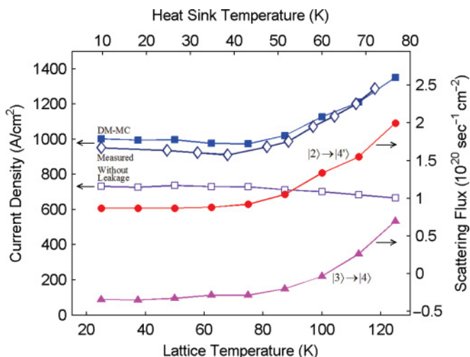
FIG. 2. (Color online) Current density as a function of lattice temperature calculated from the density matrix Monte Carlo method, with and without leakage to the continuum included. The maximum current density measured in CW mode as a function of heat sink temperature is also shown. The heat sink temperature scale is set such that, at 75 K, there is a \Delta T = 45 K between the lattice and heat sink temperatures. This \Delta T estimate is based on the approximate difference between the pulsed and CW maximum device operating temperatures. At 10 K, a \Delta T = 15 K has been set corresponding to the temperature rise typically measured in QC devices. The total net scattering flux from |3\rangle \rightarrow |4\rangle and that due to the incoherent transport between |2\rangle \rightarrow |4'\rangle is shown, which illustrates the scattering channels into |4\rangle and hence the increasing leakage at elevated lattice temperatures.
