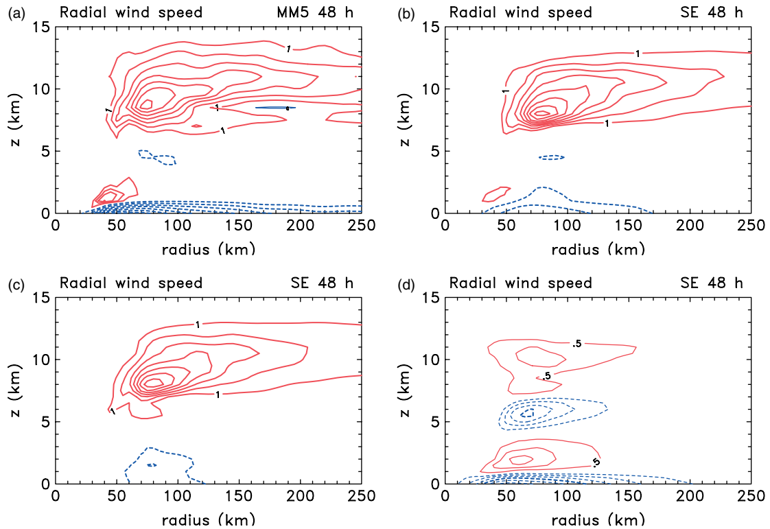
Figure 6. Radius–height sections comparing isotachs of the azimuthally–averaged radial velocity at 48 h in (a) the MM5 calculation, and (b)–(d) the corresponding ones obtained from the Sawyer–Eliassen streamfunction in Figures 4(b)–(d). In (a)–(c), the contour interval is 1 \text{ m s}^{-1} for positive (solid) values, 2 \text{ m s}^{-1} for negative (dashed) values. The zero contour is not plotted, and the thin line in (a) has the value -0.5 \text{ m s}^{-1} . In (d) the thin contours have a spacing of 0.5 \text{ m s}^{-1} . This figure is available in colour online at www.interscience.wiley.com/journal/qj
