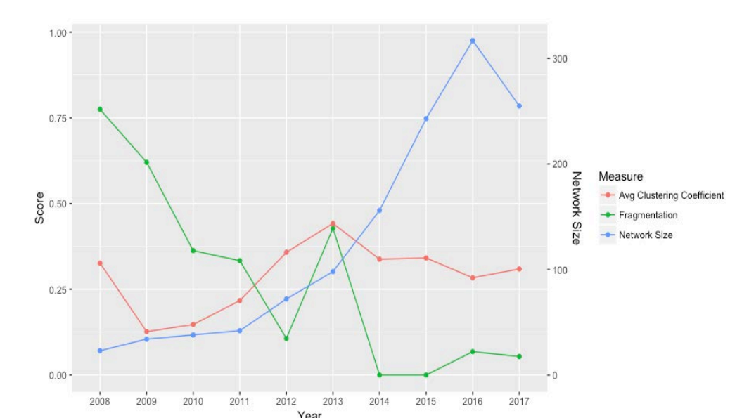
Measures for each year's network Fragmentation and Local Clustering over time.
