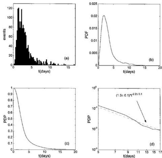
Figure 1. Statistical characteristics of VPP for zero initial error and 55 km tolerance level: (a) histogram of VPP, (b) PDF of VPP computed using the Epanechnikov kernel density, (c) PDP for VPP between 0 to 20 days, and (d) PDP for VPP between 5 to 17 days.
