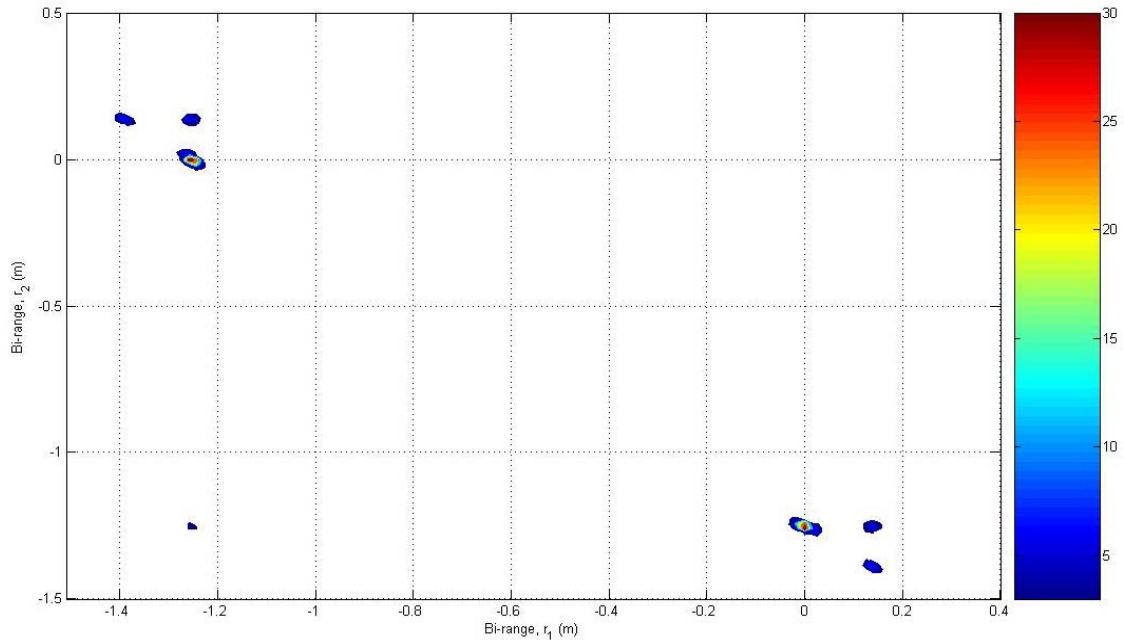
Figure 29 2-D Characteristic Bi-Range Profile of Backhoe Loader at Aspect Angles of \theta_{\text{azimuth}}=0^\circ and \varphi_{\text{elevation}}=0^\circ with HV Polarization
