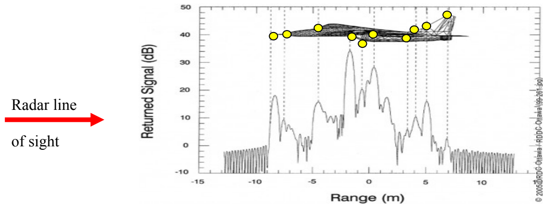
Figure 2 Radial Range Profile of a CAD modeled aircraft (Defence Research and Development Canada).
