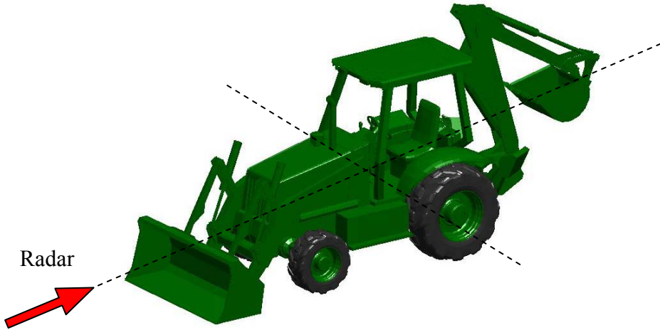
Figure 20 Orientation of CAD-Modeled Backhoe Loader at Aspect Viewing Angles of Azimuth, ( \theta_{\text{azimuth}}=0^\circ and Elevation, ( \varphi_{\text{elevation}}=0^\circ )
