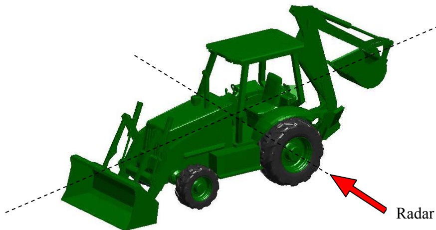
Figure 30 Orientation of CAD-Modeled Backhoe Loader at Aspect Viewing Angles of Azimuth, ( \theta_{\text{azimuth}}=90^\circ ) and Elevation, ( \varphi_{\text{elevation}}=0^\circ )
