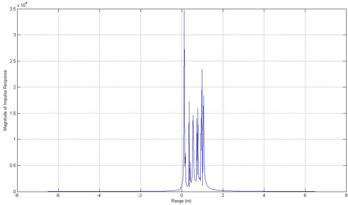
Figure 32 Radial Range Profile of Backhoe Loader at Aspect Angles of \theta_{\text{azimuth}}=90^\circ and \phi_{\text{elevation}}=0^\circ with HH Polarization
