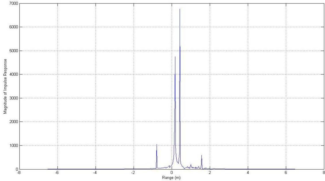
Figure 43 Radial Range Profile of Backhoe Loader at Aspect Angles of \theta_{azimuth}=60^\circ and \varphi_{elevation}=30^\circ with HV Polarization
