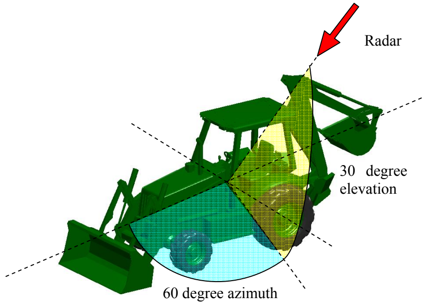
Figure 40 Orientation of CAD-Modeled Backhoe Loader at Aspect Viewing Angles of Azimuth, ( \theta_{\text{azimuth}}=60^\circ and Elevation, ( \varphi_{\text{elevation}}=30^\circ )
