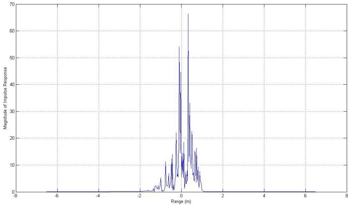
Figure 33 Radial Range Profile of Backhoe Loader at Aspect Angles of \theta_{\text{azimuth}}=90^\circ and \phi_{\text{elevation}}=0^\circ with HV Polarization
