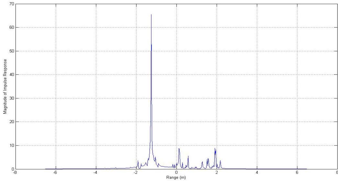
Figure 23 Radial Range Profile of Backhoe Loader at Aspect Angles of \theta_{azimuth}=0^\circ and \varphi_{elevation}=0^\circ with HV Polarization
