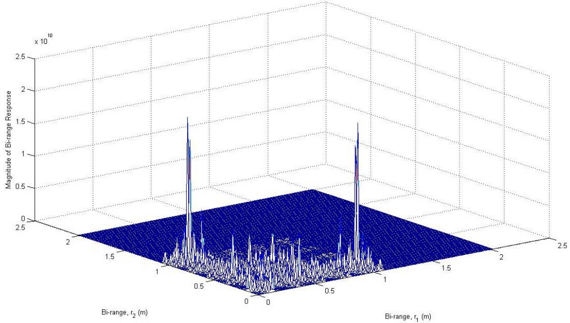
Figure 34 3-D Bi-Range Profile of Backhoe Loader at Aspect Angles of \theta_{azimuth}=90^\circ and \varphi_{elevation}=0^\circ with VV Polarization
