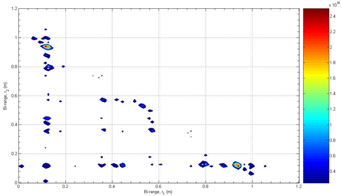
Figure 38 2-D Characteristic Bi-Range Profile of Backhoe Loader at Aspect Angles of \theta_{\text{azimuth}}=90^\circ and \phi_{\text{elevation}}=0^\circ with HH Polarization
