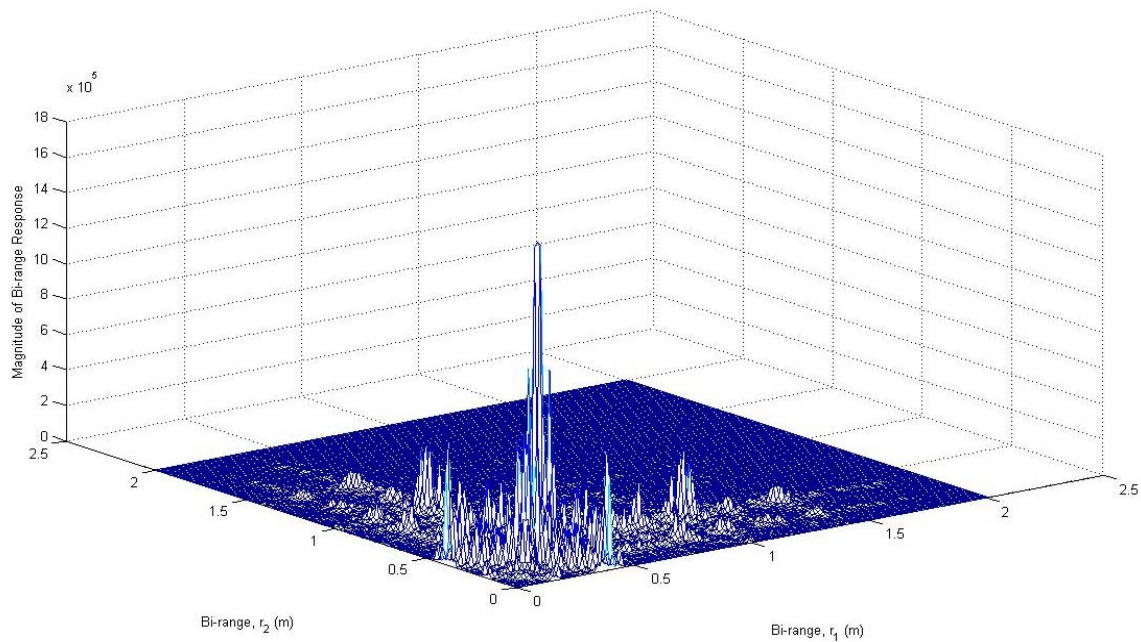
Figure 44 3-D Bi-Range Profile of Backhoe Loader at Aspect Angles of \theta_{azimuth}=60^\circ and \varphi_{elevation}=30^\circ with VV Polarization
