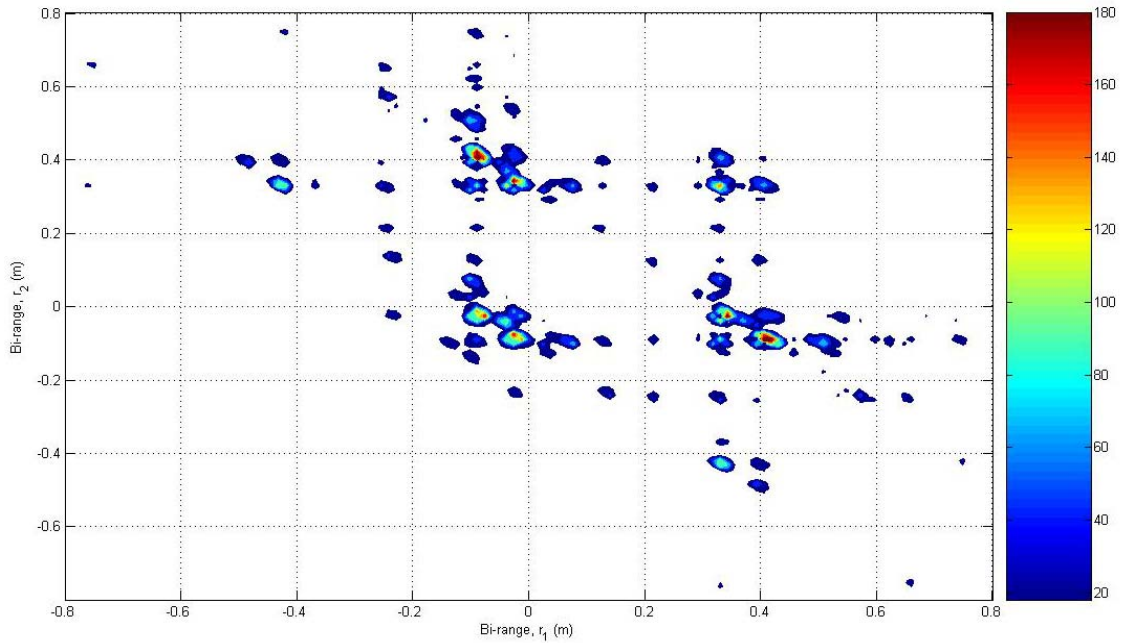
Figure 39 2-D Characteristic Bi-Range Profile of Backhoe Loader at Aspect Angles of \theta_{\text{azimuth}}=90^\circ and \phi_{\text{elevation}}=0^\circ with HV Polarization
