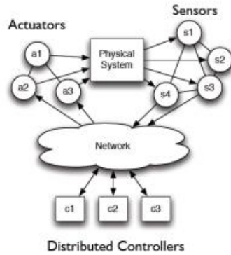
Figure 1. General Architecture of a CPS 28
