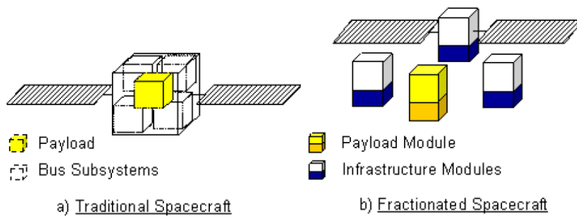
Figure 3. Traditional versus Fractionated Spacecraft 36
