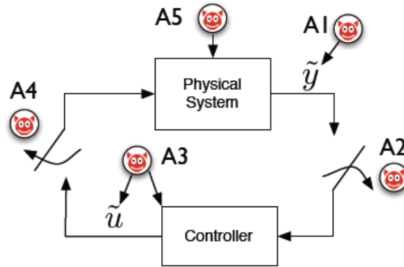
Figure 5. CPS Vulnerabilities 44
