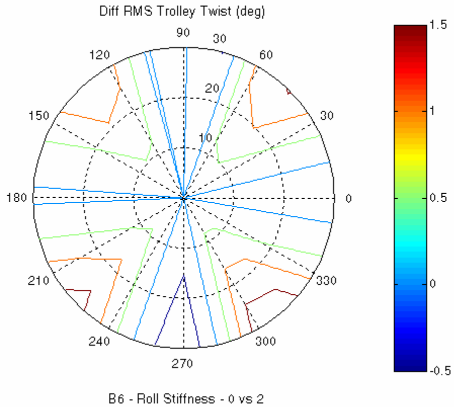
Figure 26. Difference in average vertical trolley twist angle for a Normalized Roll stiffness of 0 and 2 (subjected to Bretchneider spectrum with a wave period of 6 seconds)
