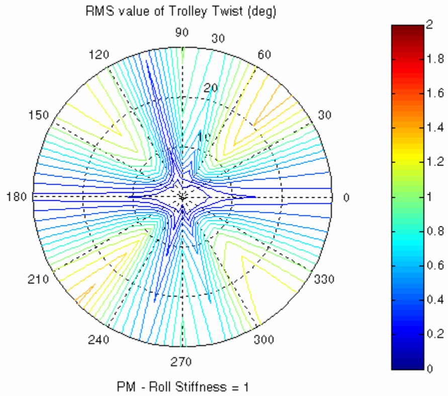
Figure 9. RMS Value of Trolley Twist Angle (degrees) subject to Pierce-Moskowitz spectrum and a Normalized Roll stiffness of 1
