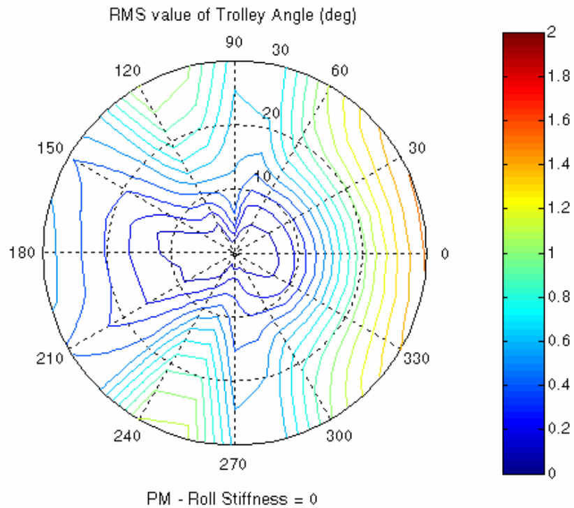
Figure 5. RMS Value of Trolley Angle (degrees) subject to Pierce-Moskowitz spectrum and zero Roll stiffness
