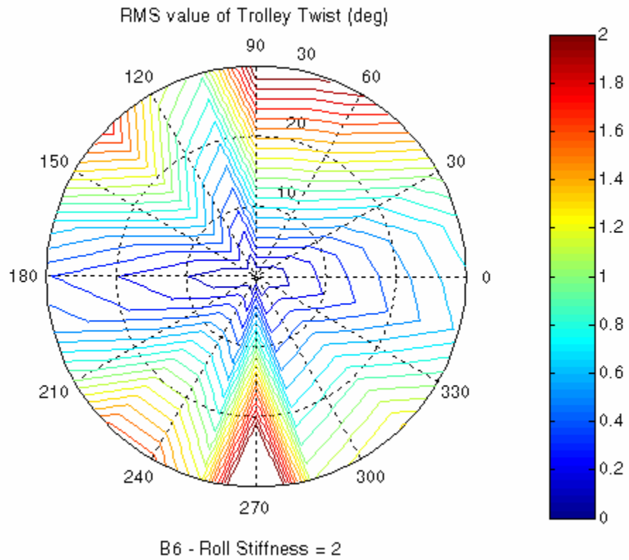
Figure 16. RMS Value of Trolley Twist Angle (degrees) subject to Bretchneider spectrum with a wave period of 6 seconds and a Normalized Roll stiffness of 2
