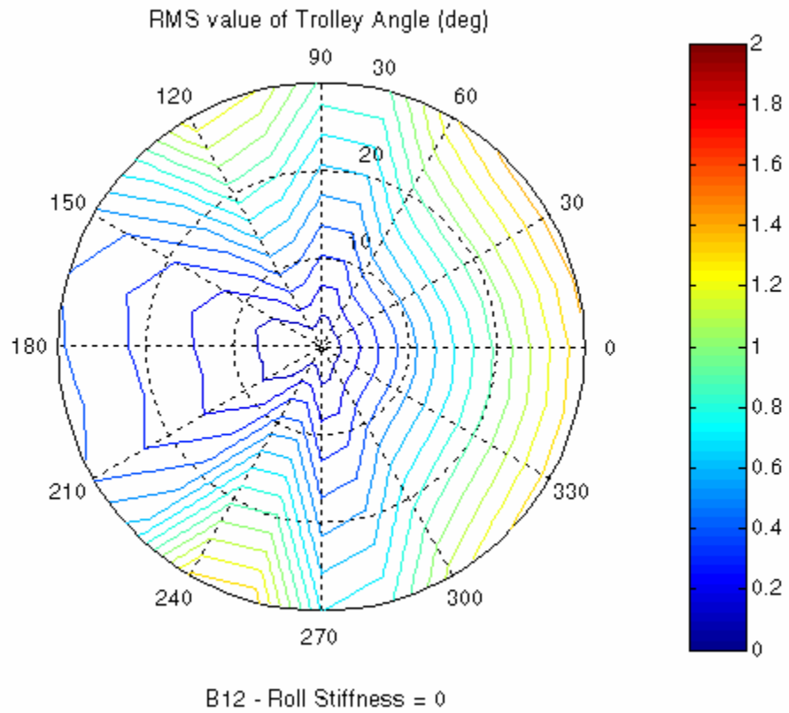
Figure 17. RMS Value of Trolley Angle (degrees) subject to Bretchneider spectrum with a wave period of 12 seconds and zero Roll stiffness
