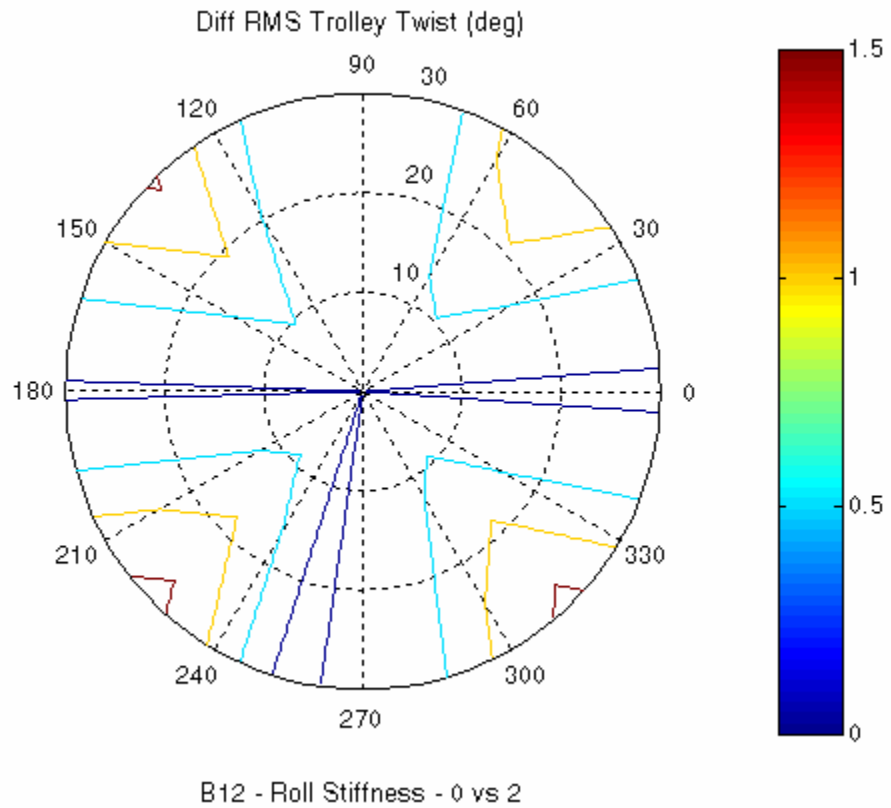
Figure 28. Difference in average vertical trolley twist angle for a Normalized Roll stiffness of 0 and 2 (subjected to Bretchenider spectrum with a wave period of 12 seconds)
