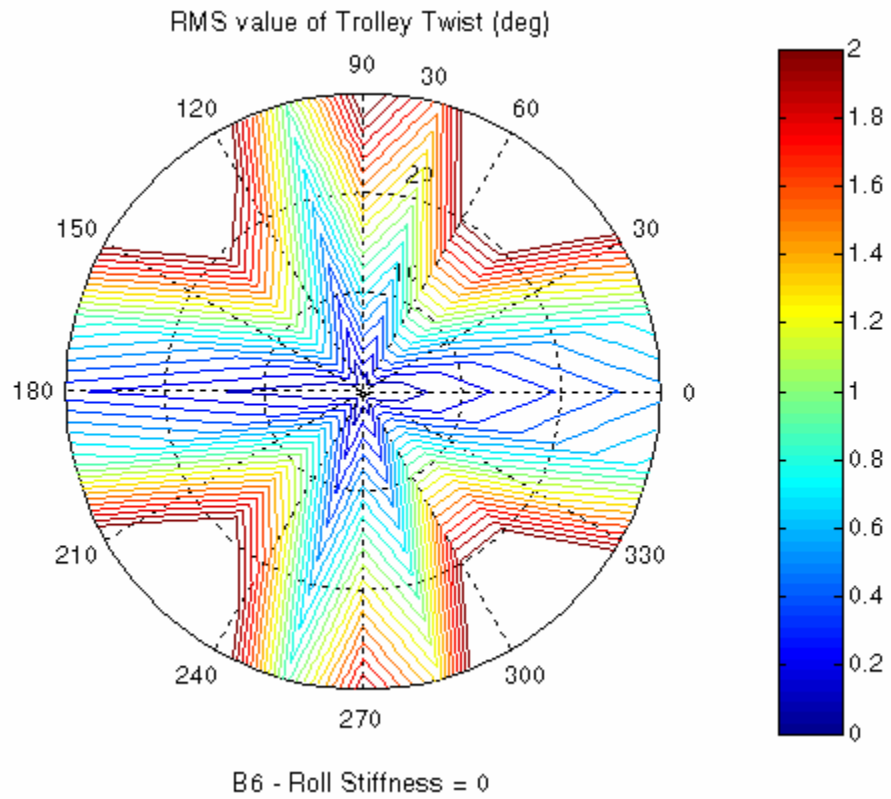
Figure 14. RMS Value of Trolley Twist Angle (degrees) subject to Bretchneider spectrum with a wave period of 6 seconds and zero Roll stiffness
