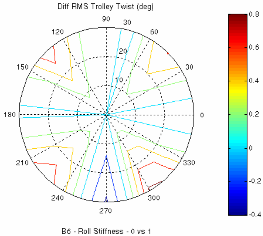
Figure 25. Difference in average vertical trolley twist angle for a Normalized Roll stiffness of 0 and 1 (subjected to Bretchneider spectrum with a wave period of 6 seconds)
